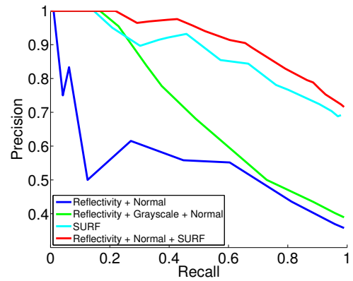
(b) Precision-Recall curve (Oct. 2010)
