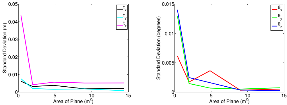
(c) Standard Deviation of estimated translation parameters
