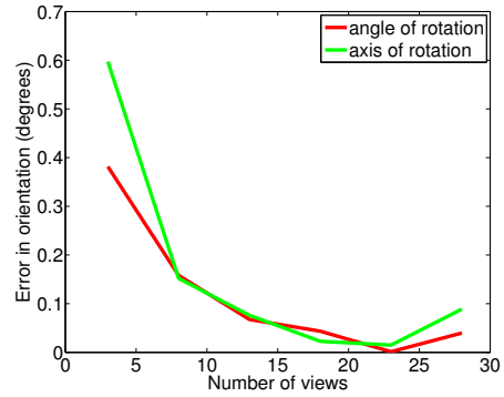
(b) Error in rotation
