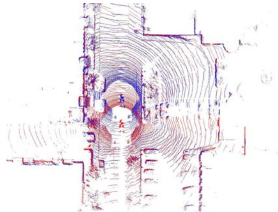
(c) Registration result for MI
