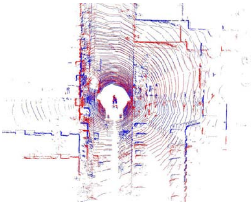
(b) Registration result for GICP
