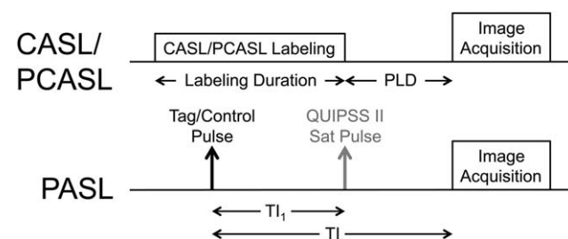
FIG. 3. Timing diagram for CASL/PCASL and PASL. For QUIPSS II PASL, T_{I_1} is the bolus duration, and is analogous to the labeling duration in CASL/PCASL. The PLD in CASL/PCASL is analogous to the quantity (T_I - T_{I_1}) in QUIPSS II PASL.
