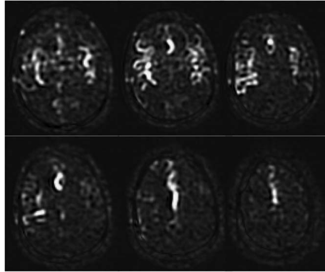
FIG. 9. Borderzone sign. These ASL subtraction images are from an 85-year-old man with dense left hemiparesis, acquired using PCASL with a labeling time of 1500 ms and a PLD of 1500 ms. Only the proximal portions of the arterial tree are present, indicating that the PLD was not long enough for the labeled spins to have reached the tissue, and that the ATT was prolonged bilaterally in this elderly patient. Although longer PLD should improve the visualization of parenchymal CBF, it is not uncommon to see such a finding, known as the borderzone sign, in elderly patients with extremely delayed arrival times.
