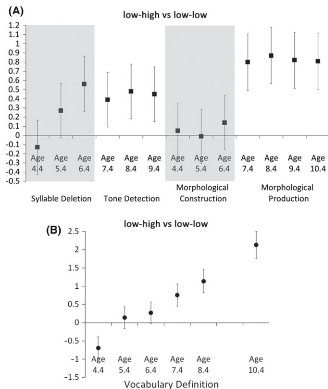
Figure 2 Effect size (Cohen's d ) for Low-high and Low-low in phonological and morphological skills, as well as vocabulary definition test.
