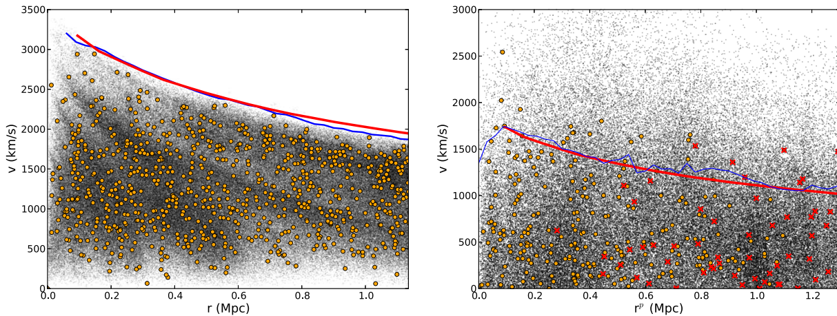
Fig. 2.— Left: Simulated three dimensional phase space of a galaxy cluster. Right: Simulated projected phase space of the same galaxy cluster along its line of sight towards us. In both figures, the black points represent dark matter particles, while the orange dots represent simulated galaxies. The red line represents the cluster’s gravitational potential, while the blue line is the estimate caustic surface. Red crosses in the right figure are interloper galaxies projected into the phase space. Figure taken from (Gifford et al. 2013).
