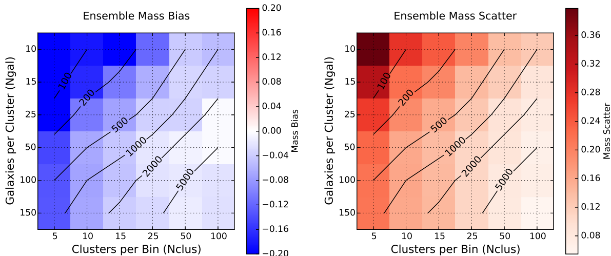
Fig. 9.— Left: Caustic mass bias with respect to the median of the individual cluster masses that make up each ensemble. Right: Caustic mass scatter about the median of the individual cluster masses that make up each ensemble.
