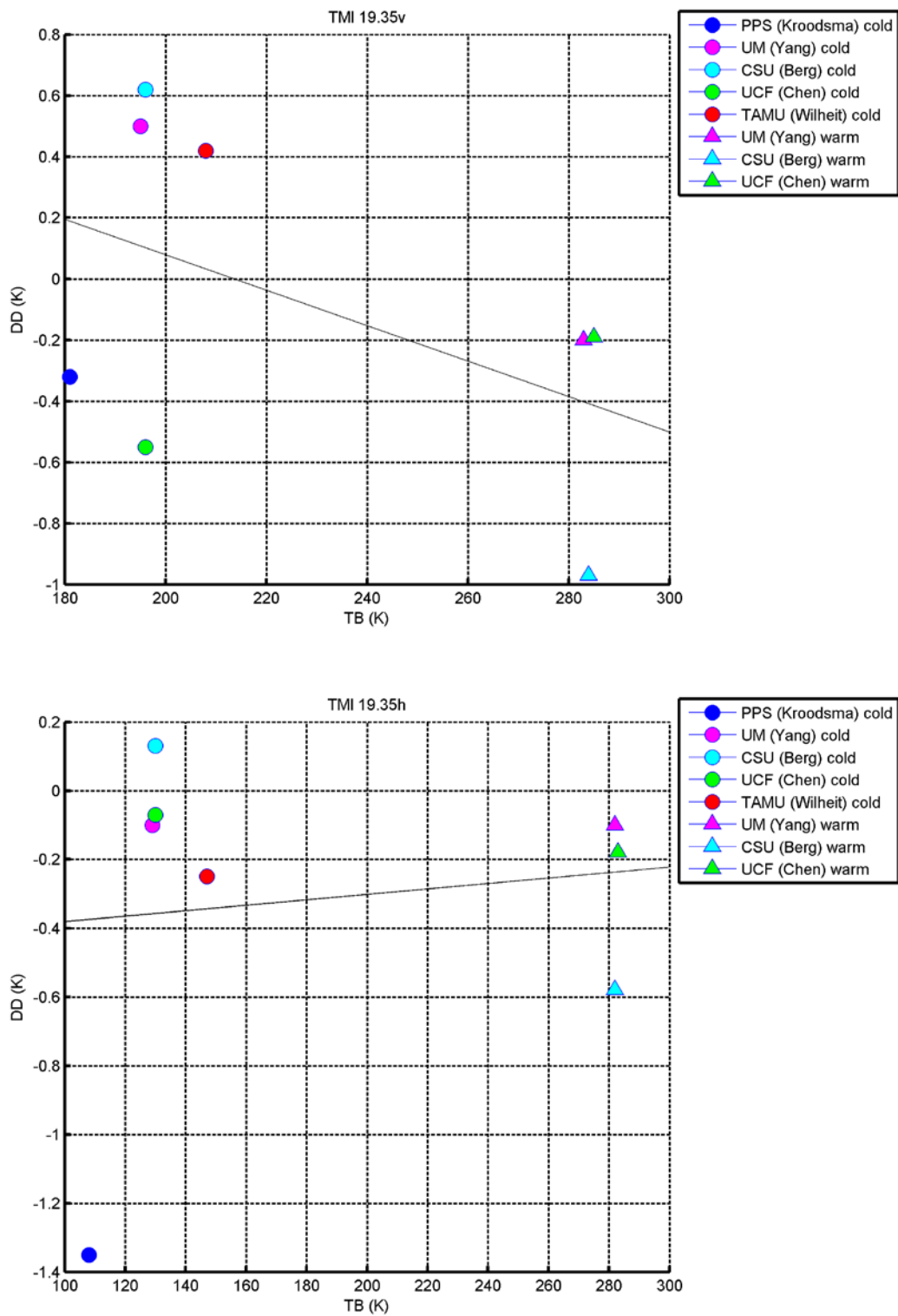
Figure 4.12: GMI-TMI cold-warm intercalibration at 19 GHz from XCAL teams.
