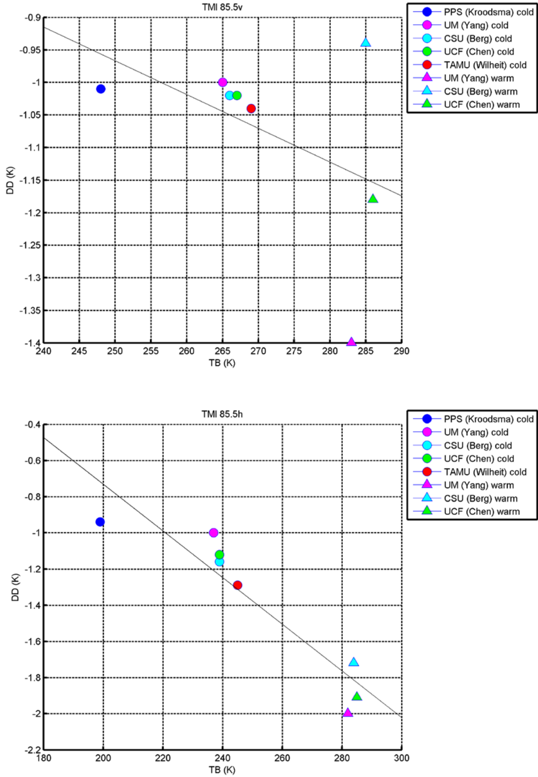
Figure 4.15: GMI-TMI cold-warm intercalibration at 89 GHz from XCAL teams.
