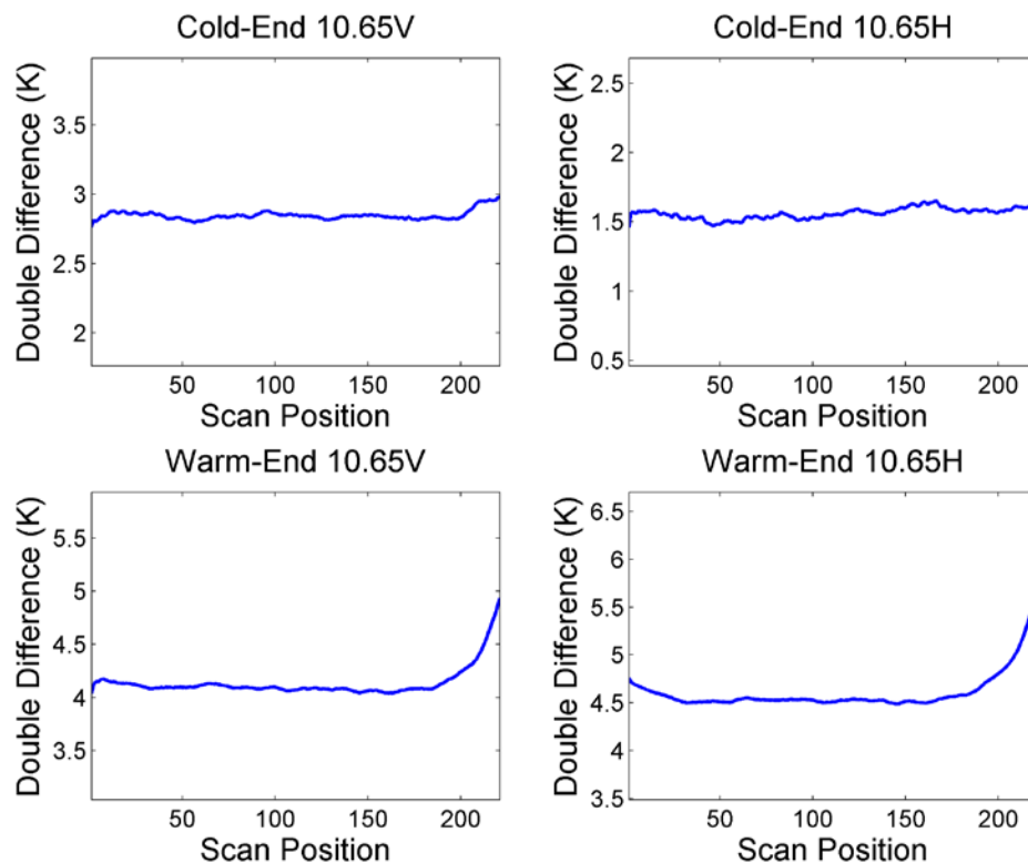
Figure 4.1: The double difference between GMI and WindSat from (upper) cold scenes and (lower) warm scenes. While the cold scene shows no residual along-scan anomalies, the warm-scene shows significant edge-of-scan blockage.
