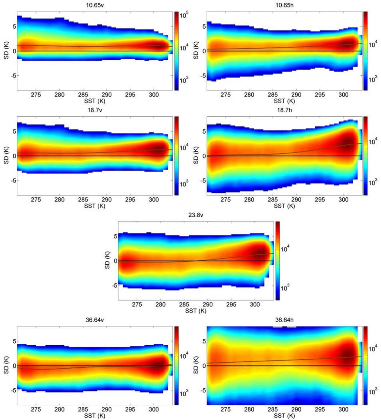
Figure 5.25: The dependence of single difference on SST.
