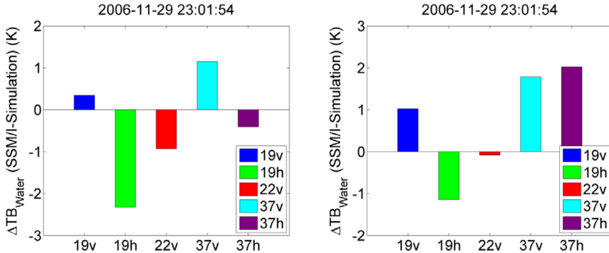
Figure 6.10: The land contamination correction error (estimated TB_{\text{Water}} – RTM simulated TB), using different numbers of pixels. The left panel shows results when using too few pixels, with no warm TBs, with biases relative to simulation of 0.34, -2.33, -0.94, 1.14 and -0.40 K for the five channels, respectively. The right panel shows results when using too many pixels, with biases of 1.02, -1.15, -0.08, 1.79 and 2.03 K, respectively. Both cases produce worse results compared to results using the appropriate number of pixels (Figure 6.7).
