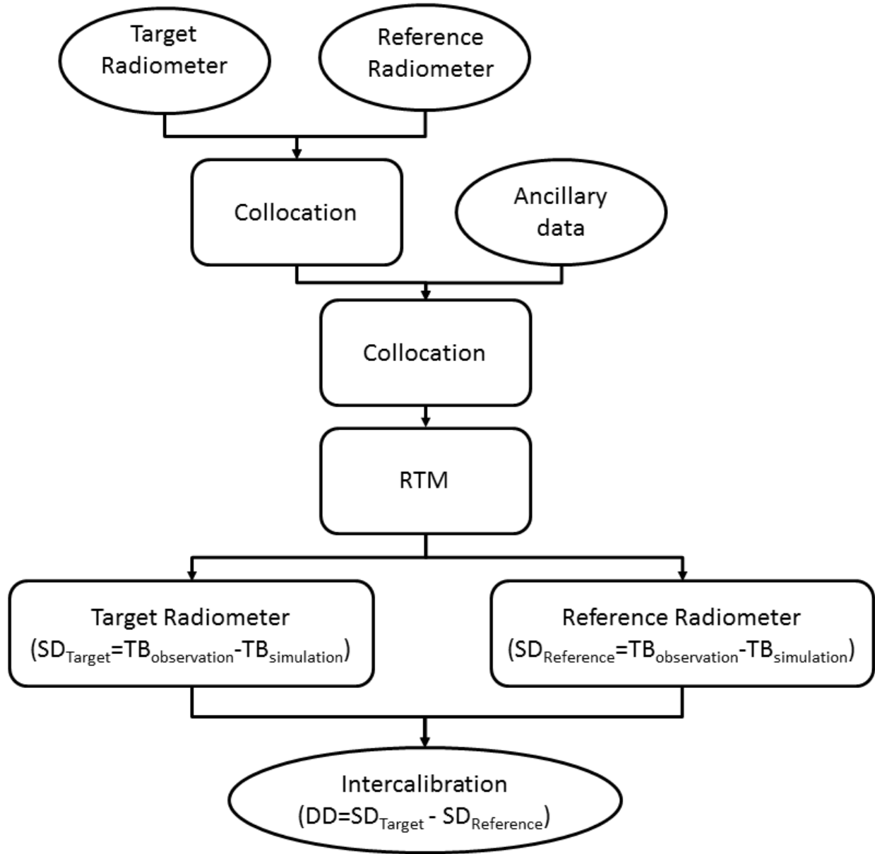
Figure 2.1: Flowchart for computing cold-end calibration single differences (SDs) and intercalibration double differences (DDs). The flowchart can be applied to an individual radiometer or to a target and reference radiometer for intercalibration.
