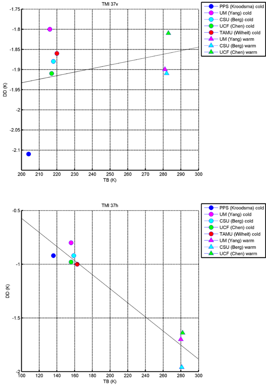
Figure 4.14: GMI-TMI cold-warm intercalibration at 37 GHz from XCAL teams.
