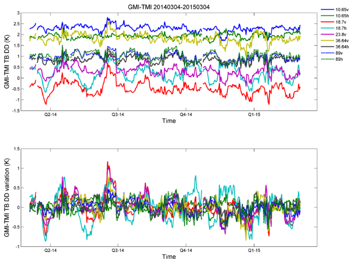
Figure 2.10: Time series of GMI-TMI daily-mean double difference. The upper panel shows the daily-mean DDs and the lower panel shows the variability with mean DDs removed.
