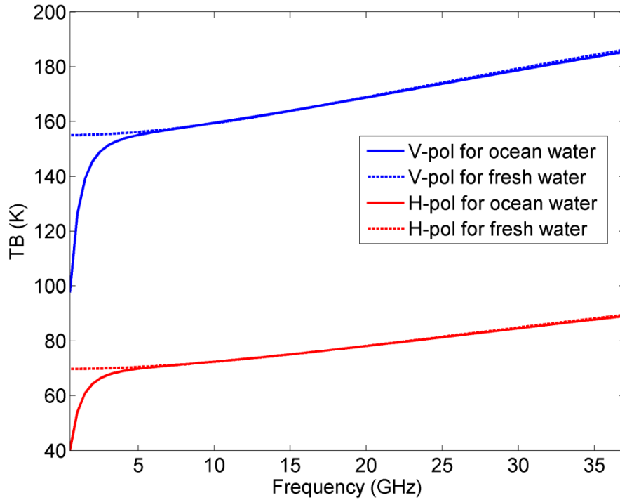
Figure 6.14: Modeled SSM/I TB emitted from the surface for ocean and fresh water, respectively. The impact of salinity becomes negligible for frequencies higher than about 5 GHz. In this model (Meissner and Wentz 2004; Elsaesser 2006), we set parameters as: salinity is 34 PPT for sea water and zero for fresh water; EIA is 53 degrees; water temperature 17 Celsius; wind speed is 6 m/s.
