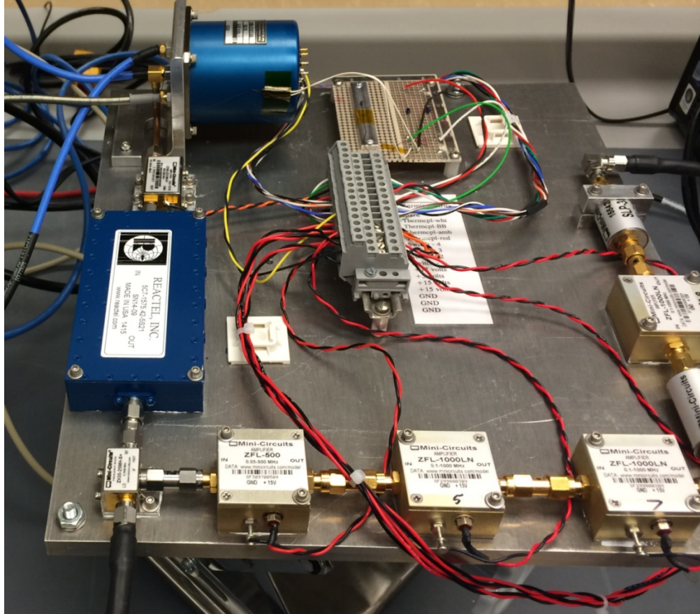
Figure 1.5: An L-band radiometer developed at the University of Michigan (Yang 2015). The circuit consists of a SP4T switch and a series of amplifiers and filters. By employing a number of amplifiers, the total gain of this radiometer is 112.35 dB. That is, the input signal is amplified by a factor of \sim 10^{11} . The input signal is negligible compared to electronic noise and therefore careful calibration is necessary.
