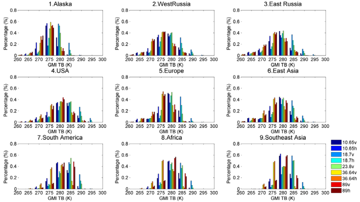
Figure 3.12: TB histograms from different regions. Boreal and temperate regions provide more cold TBs and extend the TB range for warm-end calibration.
