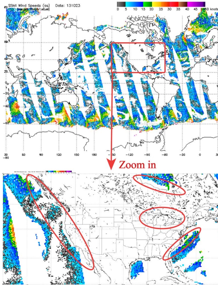
Figure 1.7: Map of SSM/I derived wind speeds globally (upper) and over North America (lower) as produced by NOAA/STAR ( http://manati.star.nesdis.noaa.gov ). The circled regions, such as the Great Lakes and water areas within 100 km of coasts, illustrate the lack of retrieval products due to land contamination.
