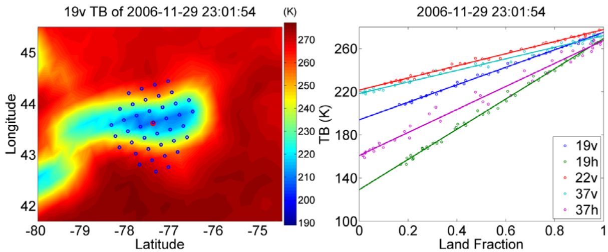
Figure 6.7: An example of solving for TB_{Water} over Lake Ontario. Left panel shows the 19v TB image, with blue circles indicating the centers of samples that are
