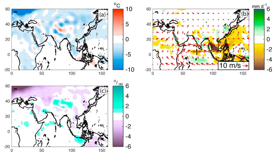
Figure 5. Climate differences due to imposing the ice sheets and sea level of the LGM. Plotting conventions are as in Figure 3, except that 850 mbar winds in Figure 5b are from the LGM ice sheet experiment. The coastline is the z = 0 contour from the ICE-5G reconstruction [Peltier, 2004], which differs from the coastline in the other figures (particularly in southeast Asian and the maritime continent).
