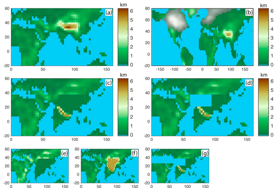
Figure 2. Surface topography for the various experiments shown at model resolution. (a) Control: modern topography; (b) LGM boundary conditions: LGM ice sheets plus sea level differences (shown on an expanded domain); (c) Himalaya South: stylized Indian geometry for ~50 Ma, retaining topography of the modern Himalaya; (d) Paratethys: same as Himalaya South but with a stylized Paratethys Sea added; (e) Flat South: coastline as in Himalaya South but Himalaya removed; (f) Mega-Tibet: coastline as in Himalaya South but interior plateau retained; (g) Greater Paratethys, as in Figure 2d but with Paratethys extending to the Atlantic.
