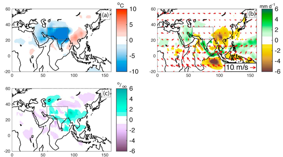
Figure 8. Climate differences between the Paratethys experiment and the Himalaya South experiment. Plotting conventions are as in Figure 3, except that 850 mbar winds in Figure 8b are from the Paratethys experiment. The extent of the idealized Paratethys is indicated by the grey box.
