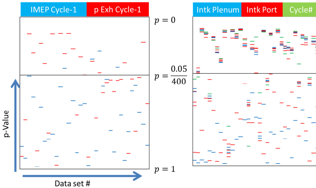
Figure E-2 Statistical significance of previous cycle pressures (left), and current cycles pressures and cycle number (right) on CA10.
