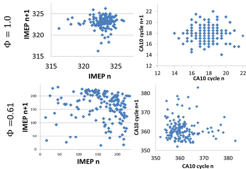
Figure 4-6 Dependence of IMEP and CA10 on previous cycle.
