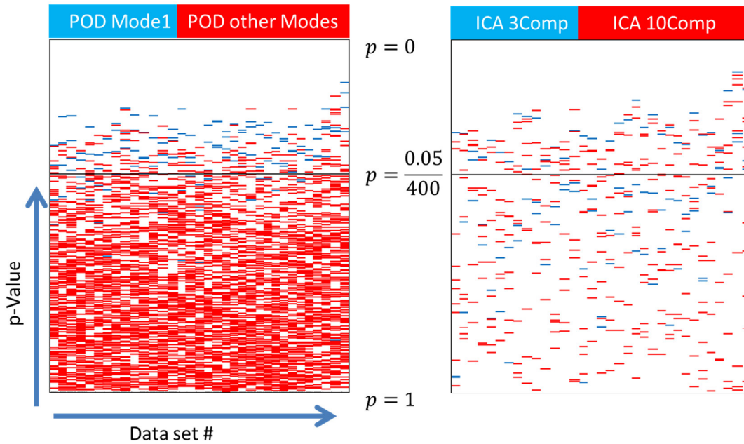
Figure E-1 Statistical significance of POD (left) and ICA (right) mode coefficients on CA10.
