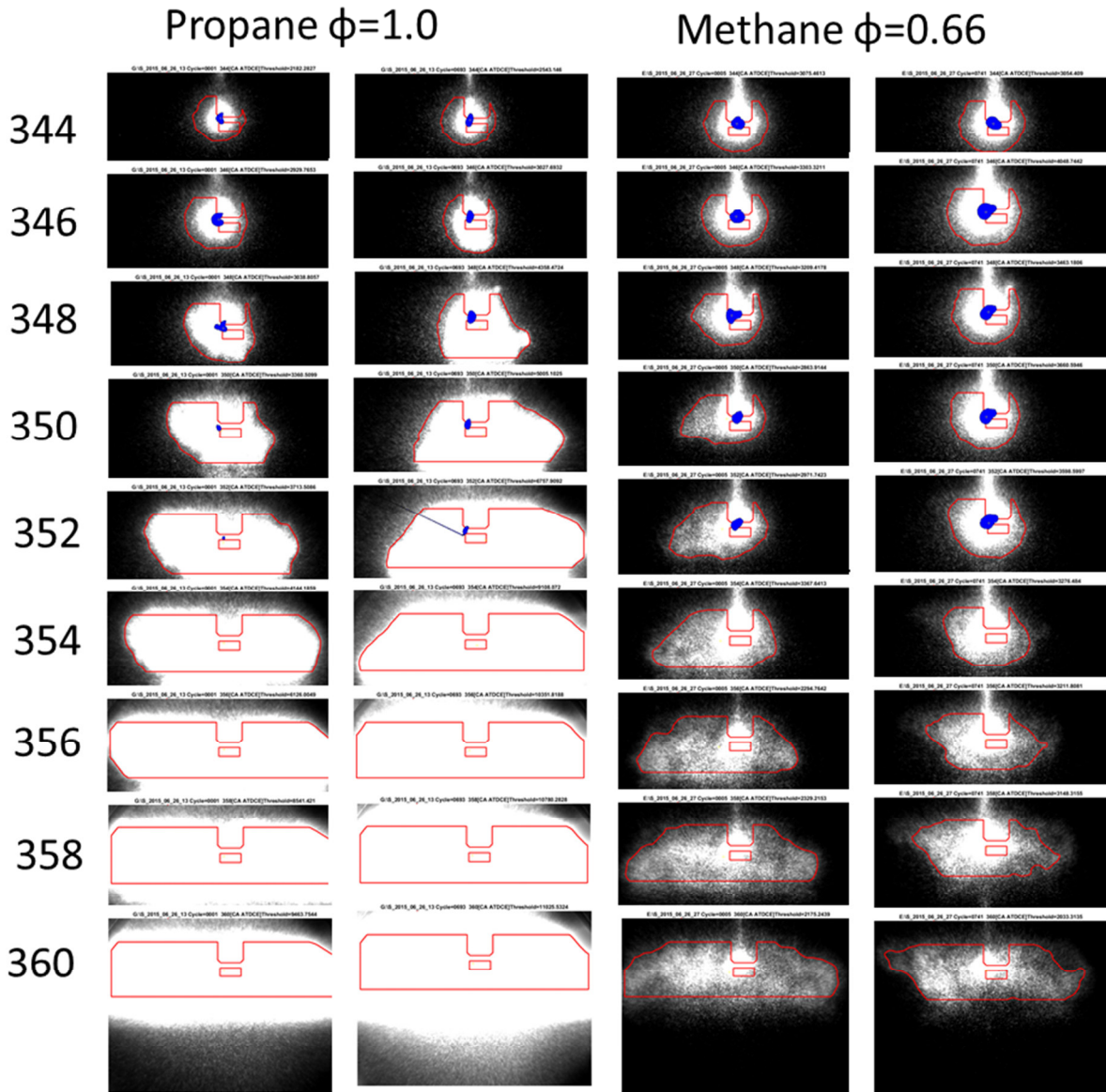
Figure D-1 Examples of OH* contour recognition results.
