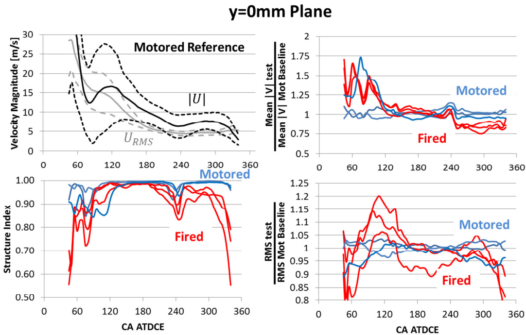
Figure C-2 Quantitative comparison of flow similarities between motored and fired cases in y=0mm plane.
