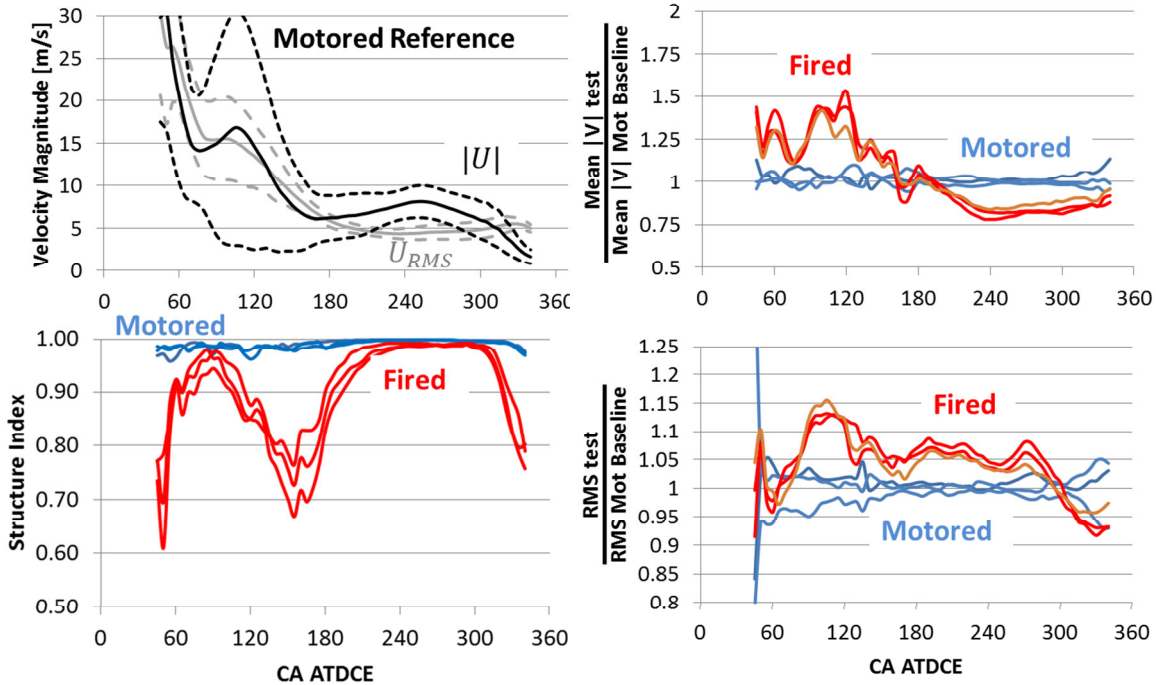
Figure C-3 Quantitative comparison of flow similarities between motored and fired cases in x=0mm plane.
