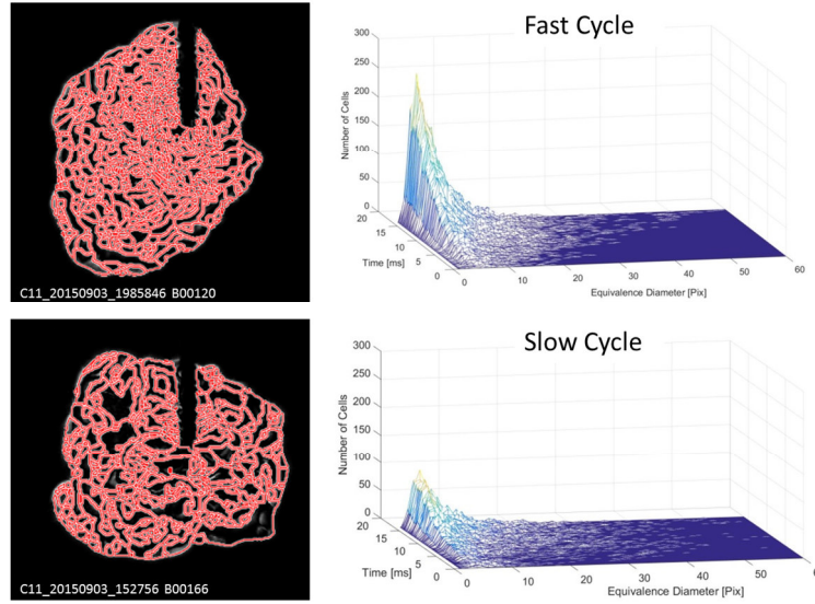
Figure 2-41 Extraction of Schlieren flame structure information
