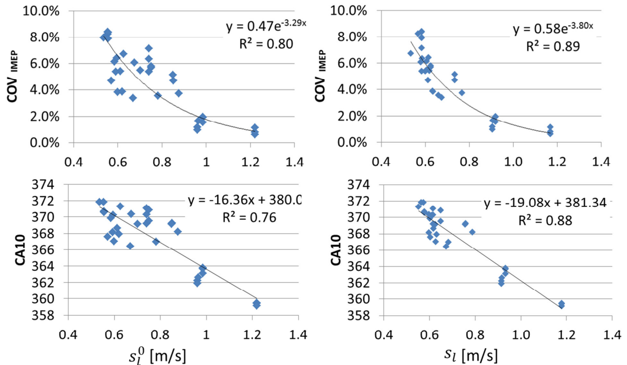
Figure 6-8 Correlation of combustion variability as measured by COV IMEP (top) and combustion phasing (bottom) to unstretched laminar flame speed (left) and stretched laminar flame speed (right).
