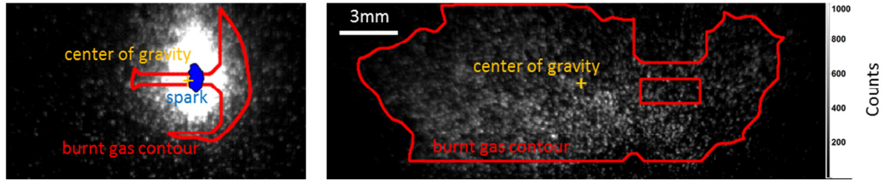
Figure 2-35 Example OH* contour at early spark times (344 CA ATDCE) and at TDC for weak intensity lean methane flames
