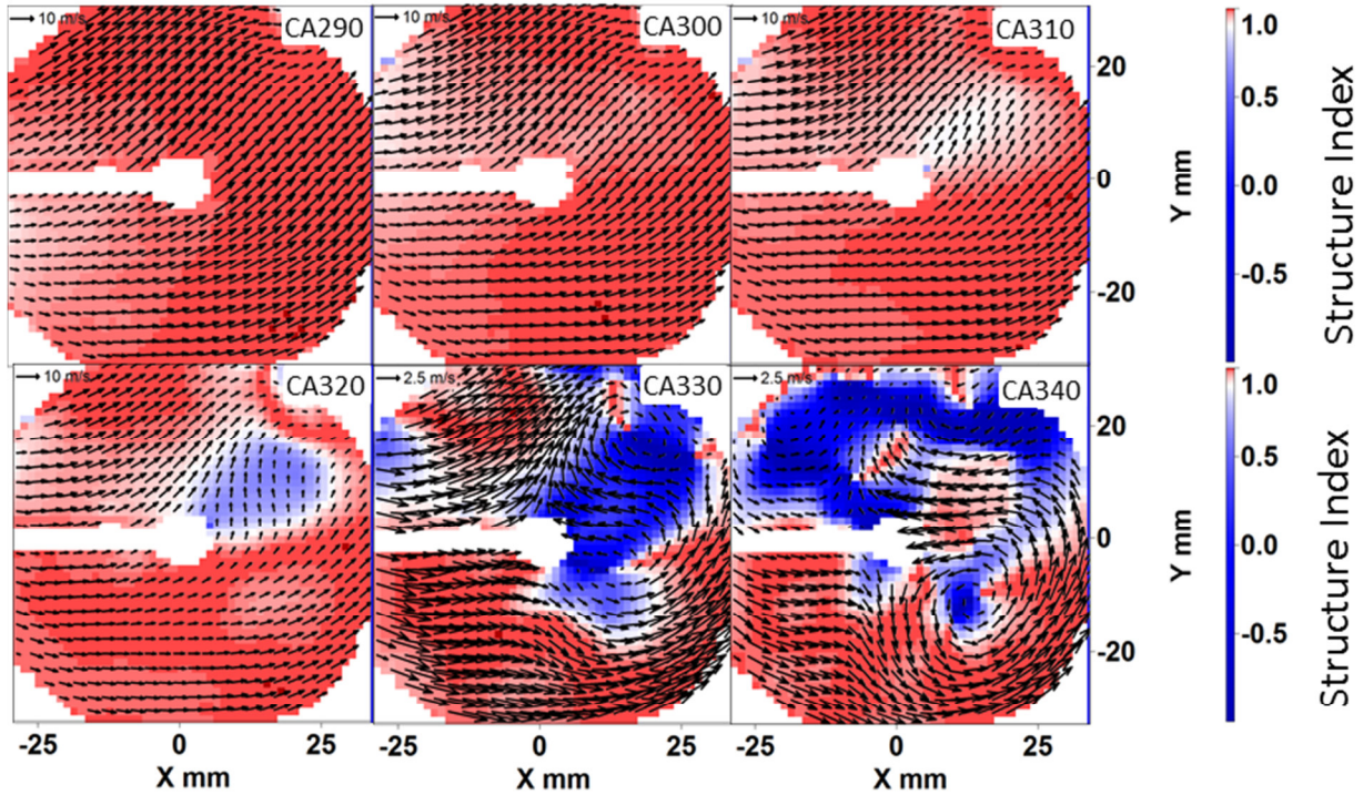
Figure 3-15 Spatial distribution of structure index comparing a ensemble average flow field of a fired test to the reference ensemble average flow field with overlaid motored ensemble average reference flow field (every 4 th vector shown).
