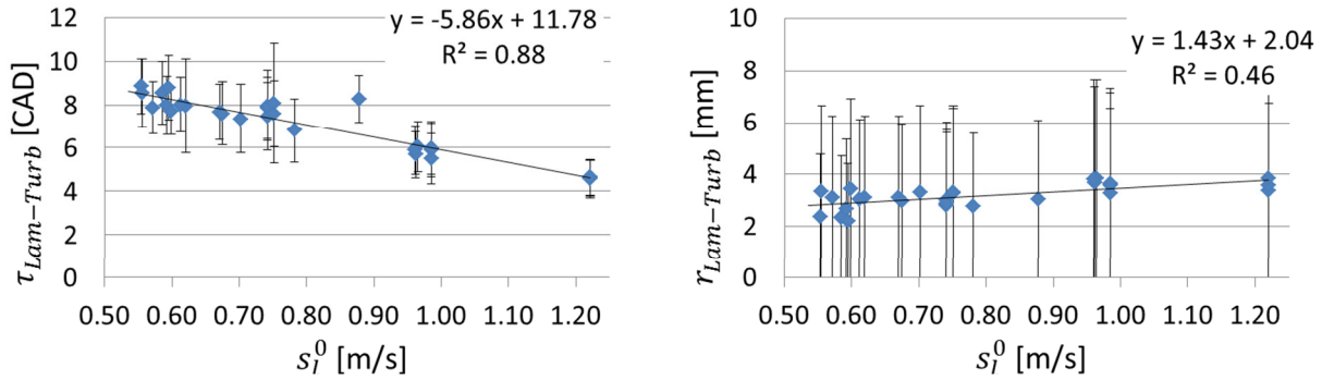
Figure 6-7 The laminar to turbulent transition time is uniquely a function of laminar flame speed. Symbols indicate mean values for each test. Error bars show \pm 1 StDev. The radius at which the transition occurs is approximately constant and is typically smaller than half the clearance distance.
