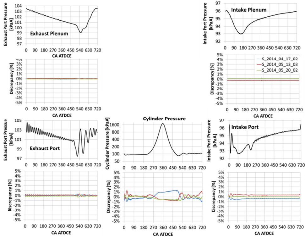
Figure B-1 Pressure traces and test-to-test pressure discrepancy 800RPM 95kPa motored condition
