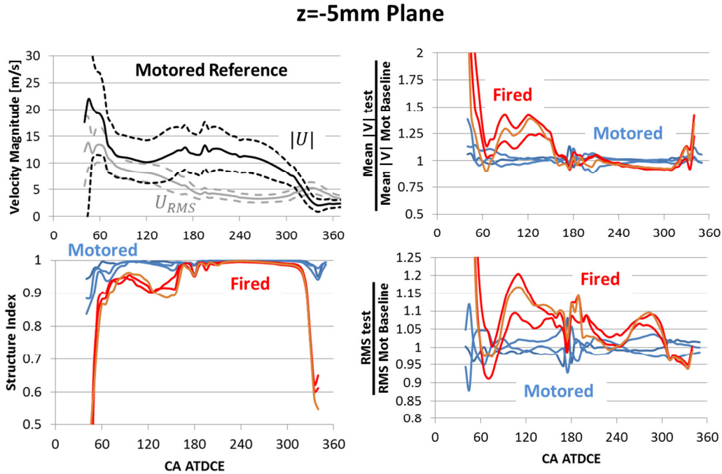
Figure C-1 Quantitative comparison of flow similarities between motored and fired cases in z=-5mm plane.
