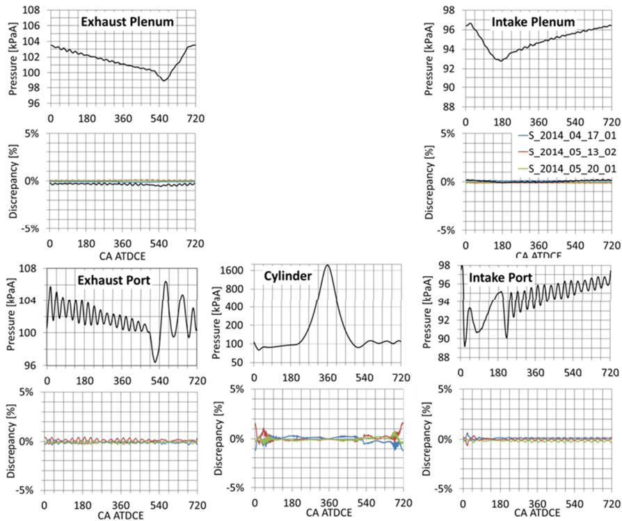
Figure B-2 Pressure traces and test-to-test pressure discrepancy 1300RPM 95kPa motored condition
