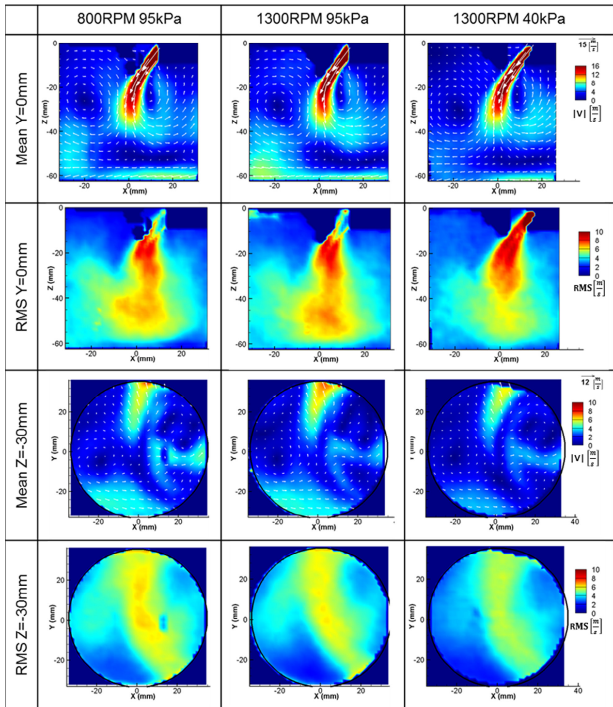
Figure 3-5 Mean and RMS velocities normalized by piston speed for three operation conditions at 100CAD ATDC
