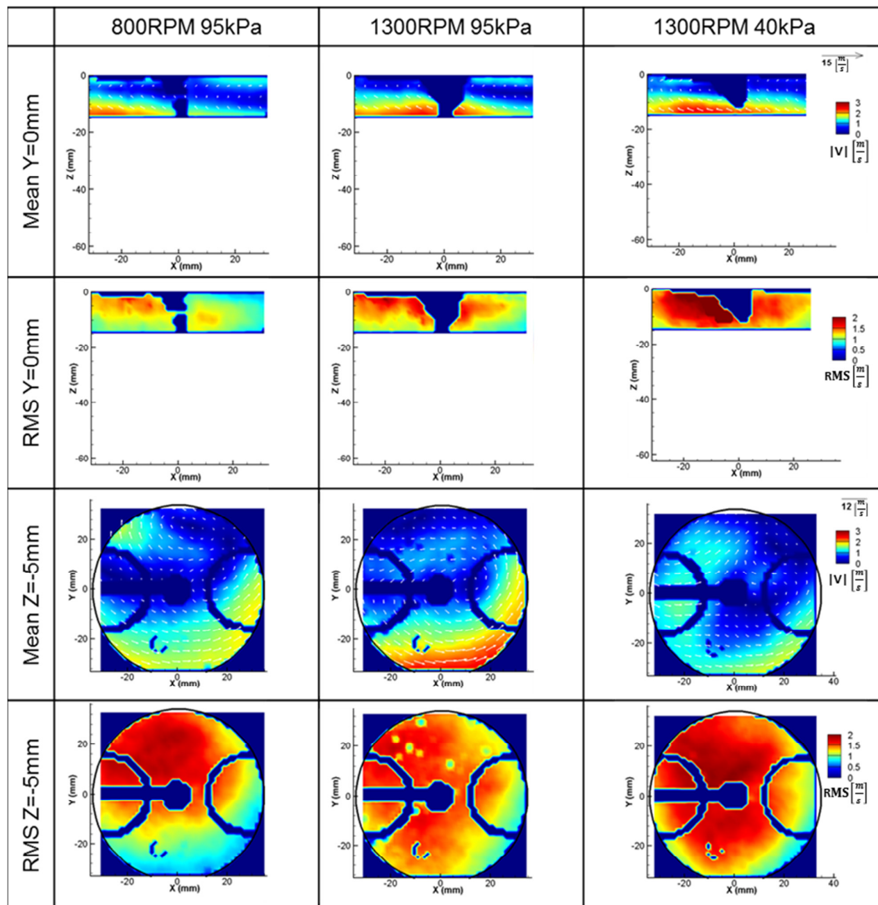
Figure 3-9 Mean and RMS velocities normalized by mean piston speed for three operation conditions at 330CAD ATDCE
