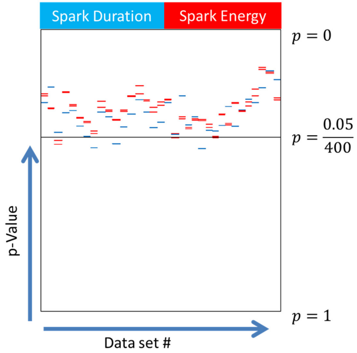
Figure E-3 Statistical significance of spark duration and energy on CA10.
