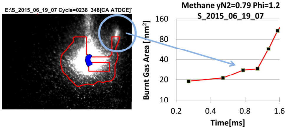
Figure D-2 Interference of cylinder head paint excited by PLIF 266nm laser, causing measurement error in OH* area.
