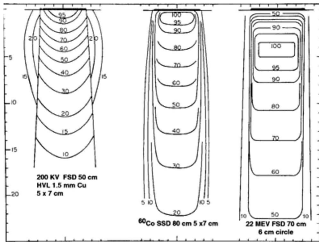
FIG. 6. Isodose curves from typical systems in use in the mid 1960s (Johns and Cunningham).
