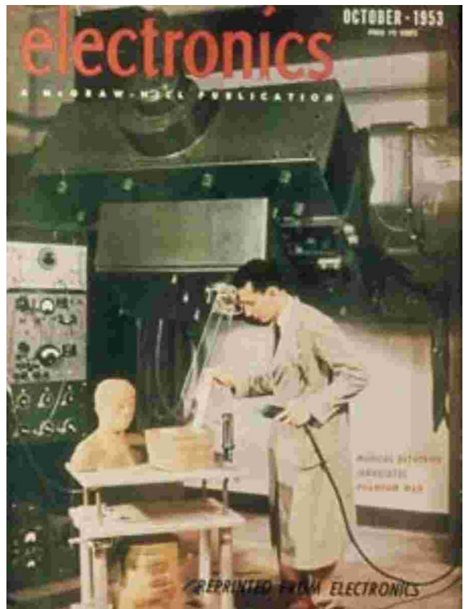
FIG. 4. MSKCC Betatron (electrons only) and phantom with inhomogeneities.
