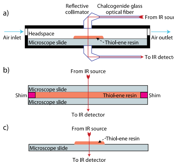
Scheme 2: Schematic diagrams of experimental configurations used to examine oxygen-mediated polymerization kinetics by FTIR spectroscopy. a) A sealed sample cell permits measurement of IR spectra under anaerobic conditions until air is introduced into the cell via inlet and outlet ports. b) Sandwiching a resin formulation, mixed under oxygen-saturated conditions, between two glass slides throughout IR spectra collection prevents additional oxygen from diffusing into the sample during polymerization. c) A resin formulation, mixed under oxygen-saturated conditions, is exposed to the atmosphere throughout IR spectra collection, permitting oxygen to diffuse into the sample during polymerization.
