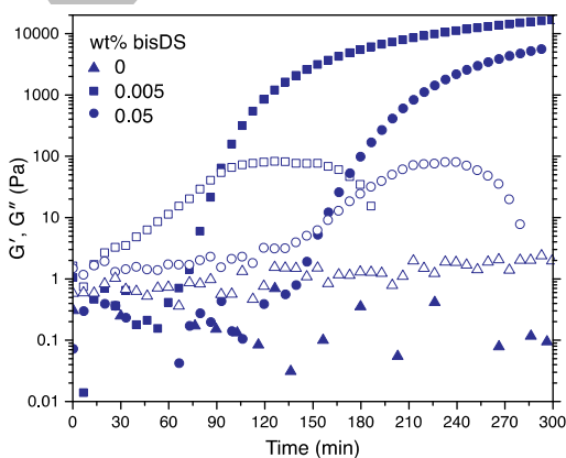
Figure 9: Storage ( G' , closed symbols) and loss ( G'' , open symbols) moduli, measured by parallel plate rheometry, of bisDS-containing ETTMP/TATATO thiol–ene formulations mixed under oxygen-saturated conditions.
