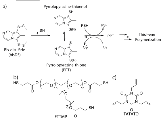
Scheme 1: Structures of the oxygen-mediated initiator and monomers used. a) The bis-disulfide (bisDS) derivative of oltipraz is converted to a PPT intermediate by reaction with a thiol. Subsequently, in the presence of both thiol and oxygen, the PPT participates in a radical-generating redox cycle, 1 resulting in thiol-ene polymerization. b) Ethoxylated trimethylolpropane tri(3-mercaptopropionate) (ETTMP). c) 1,3,5-Triallyl-1,3,5-triazine-2,4,6(1H,3H,5H)-trione (TATATO).
