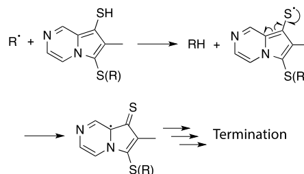
Scheme 3: Proposed polymerization inhibition mechanism. In the presence of excess PPT, an active radical abstracts a hydrogen from the thioenol tautomer, generating a resonance-stabilized, unreactive PPT• intermediate, inhibiting the radical-affording redox cycle as well as removing PPT.
