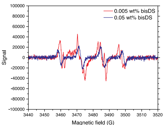
Figure 2: EPR spectra for solutions mixed under anaerobic conditions of bisDS, ETTMP, and DMPO in DMSO, collected 15 minutes after
