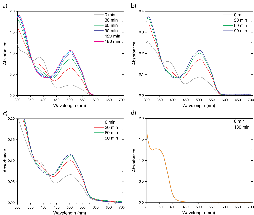
Figure 1: UV-Vis absorption spectra for bisDS-containing resin formulations mixed and maintained under anaerobic conditions. a) 0.05 wt% bisDS in ETTMP and TATATO; b) 0.01 wt% bisDS in ETTMP and TATATO; c) 0.005 wt% bisDS in ETTMP and TATATO; and d) 0.05 wt% in 83.6 wt% PEG (i.e., thiol-free) and 16.4 wt% TATATO.
