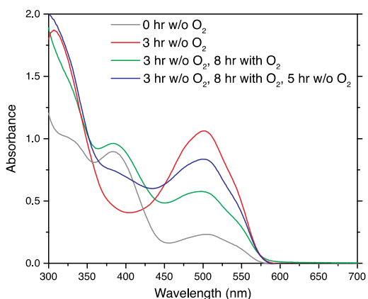
Figure 6: UV-Vis absorption spectra for a thiol-ene formulation of 0.05 wt% bisDS in ETTMP-TATATO immediately after mixing under anaerobic conditions, after 3 hours maintained under anaerobic conditions, after 8 hours of subsequent atmosphere exposure, and finally after 5 hours sealed in a cuvette to eliminate further oxygen diffusion.
