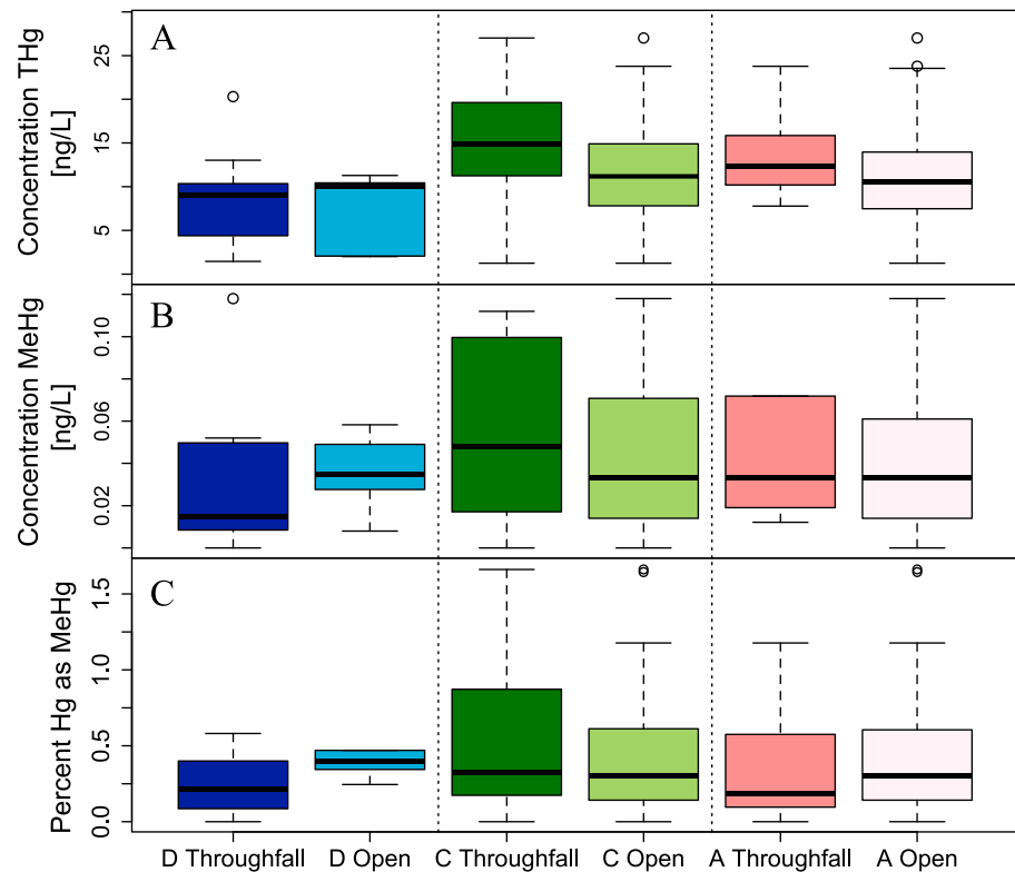
Figure 1. Concentrations of (a) total mercury, (b) methylmercury, and (c) percent mercury as methylmercury in wet deposition (throughfall and open precipitation) across different forest cover types at Whiteface Mountain (D represents deciduous, C represents coniferous, and A represents alpine). Box and whisker plots show median values, Q1, and Q3 within the boxes, and the whiskers represent Q1-1.5 \times interquartile range and Q3 + 1.5 \times interquartile range ( n = 19 for throughfall at each forest cover type, n = 5 for open precipitation at each forest cover type). Only outliers within the given bounds are shown.
