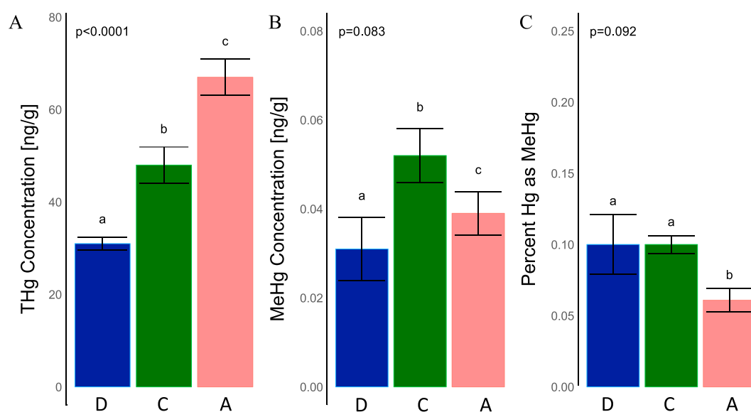
Figure 2. Concentrations of litterfall (a) total mercury, (b) methylmercury, and (c) percent mercury as methylmercury across different forest cover types at Whiteface Mountain (D represents deciduous, C represents coniferous, and A represents alpine). Barplots show mean values, and error bars denote standard error ( n = 4 for each forest cover type). Reported p values represent differences between all levels ( H_0 = means for all forest cover types are equal). Letters denote significant differences using Tukey's post hoc adjustment at an alpha level of 0.05.
