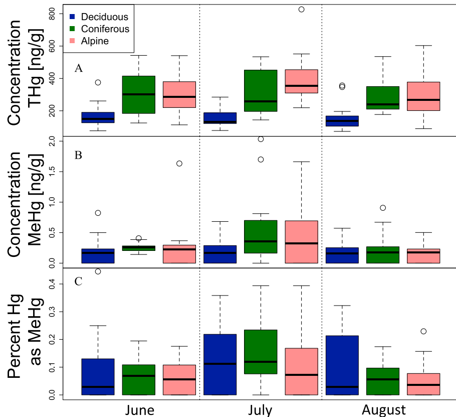
Figure 4. Concentrations of (a) total mercury, (b) methylmercury, and (c) percent mercury as methylmercury in organic soils across the growing season at different forest cover types at Whiteface Mountain. Box-and-whisker plots show median values, Q1, and Q3 within the boxes, and the whiskers represent Q1 - 1.5 \times \text{interquartile range} and Q3 + 1.5 \times \text{interquartile range} ( n = 24 for each forest cover type in each month). Only outliers within the given bounds are shown.
