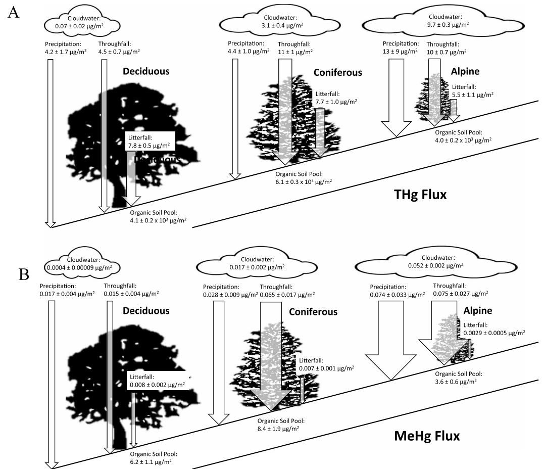
Figure 5. Comparison of growing season (May–September) (a) total mercury and (b) methylmercury fluxes and organic soil pools in different forest cover types at Whiteface Mountain. Values denote mean and standard error (calculated by propagating errors in mercury concentration).
