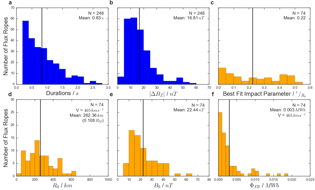
Figure 5. Histograms showing the distribution of several key flux rope parameters. Panels (a) and (b) are shown for the MVA confirmed flux ropes (in blue) while panels (c)-(f) are only shown for the force-free subset (in orange) as they require parameters from the successful model fit. The means of the distribution are indicated with black vertical bars (and numerically in the upper right of the panels). Panel (a) shows the duration of the flux ropes as measured by the in-situ spacecraft data, between the extremes of the bipolar B_Z variation. Panel (b) shows the distribution of |\Delta B_Z| . Panel (c) shows the distribution of best fit impact parameters from the force-free model fit, panel (d) shows the inferred radius of the flux ropes, calculated assuming a velocity of 465 km s^{-1} and correcting for the impact parameter of the encounter. Panel (e) displays the core fields observed, again inferred from the force-free fit. Panel (f) shows the distribution of flux contained within the flux ropes, calculated using Equation 4.
