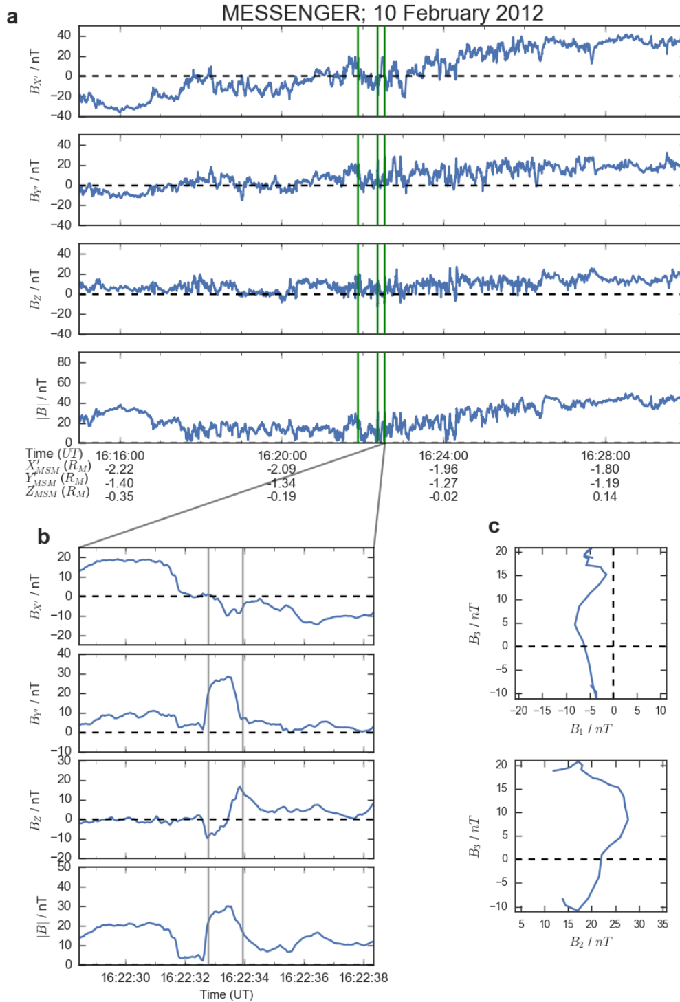
Figure 1. An illustrative plasma sheet crossing (a) with a zoom in of a flux rope detection (b) and example MVA hodograms (c). Panel (a) shows 15 minutes of 20 Hz MESSENGER magnetometer data in aberrated MSM coordinates; flux rope encounters are shaded green. Panel (b) shows 10 s of data around an in-situ flux rope encounter. Once more the data are presented in aberrated MSM coordinates. The vertical grey bars indicate the region selected for minimum variance analysis (MVA), the resulting magnetic field hodograms (in the MVA system) are shown in panel (c).
