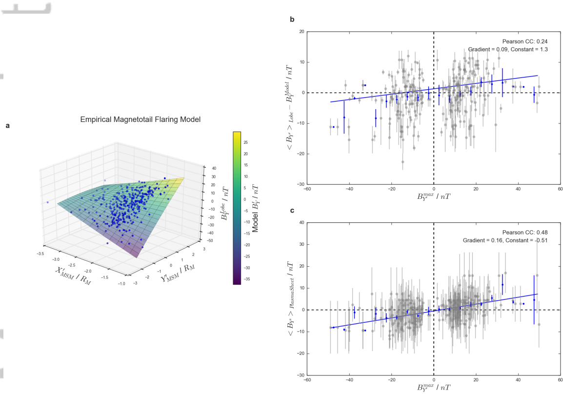
Figure 8. Panel (a) shows the distribution of B_Y measured across the tail within the lobe (projected onto the X'_{MSM} - Y'_{MSM} plane). The surface shows the least squares quadratic fit to the data, the color bar corresponds to the resulting modeled value of B_Y . Panel (b) shows the model subtracted value of B_Y measured in the lobe plotted against the maximum B_Y recorded in the 248 MVA confirmed flux ropes. Panel (c) shows the average B_Y measured within the plasma sheet compared to the maximum B_Y recorded within the 248 MVA confirmed flux ropes. For panels (b) and (c) the grey points indicate individual flux ropes (with the error bars showing \pm 1\sigma ) while the data are also placed into 5 nT bins, the mean and standard error of the mean are shown in blue. The blue lines show the result of a least squares fit to the grey points. The values of the Pearson correlation coefficient and least squares fit are provided in the top right of the panels.
