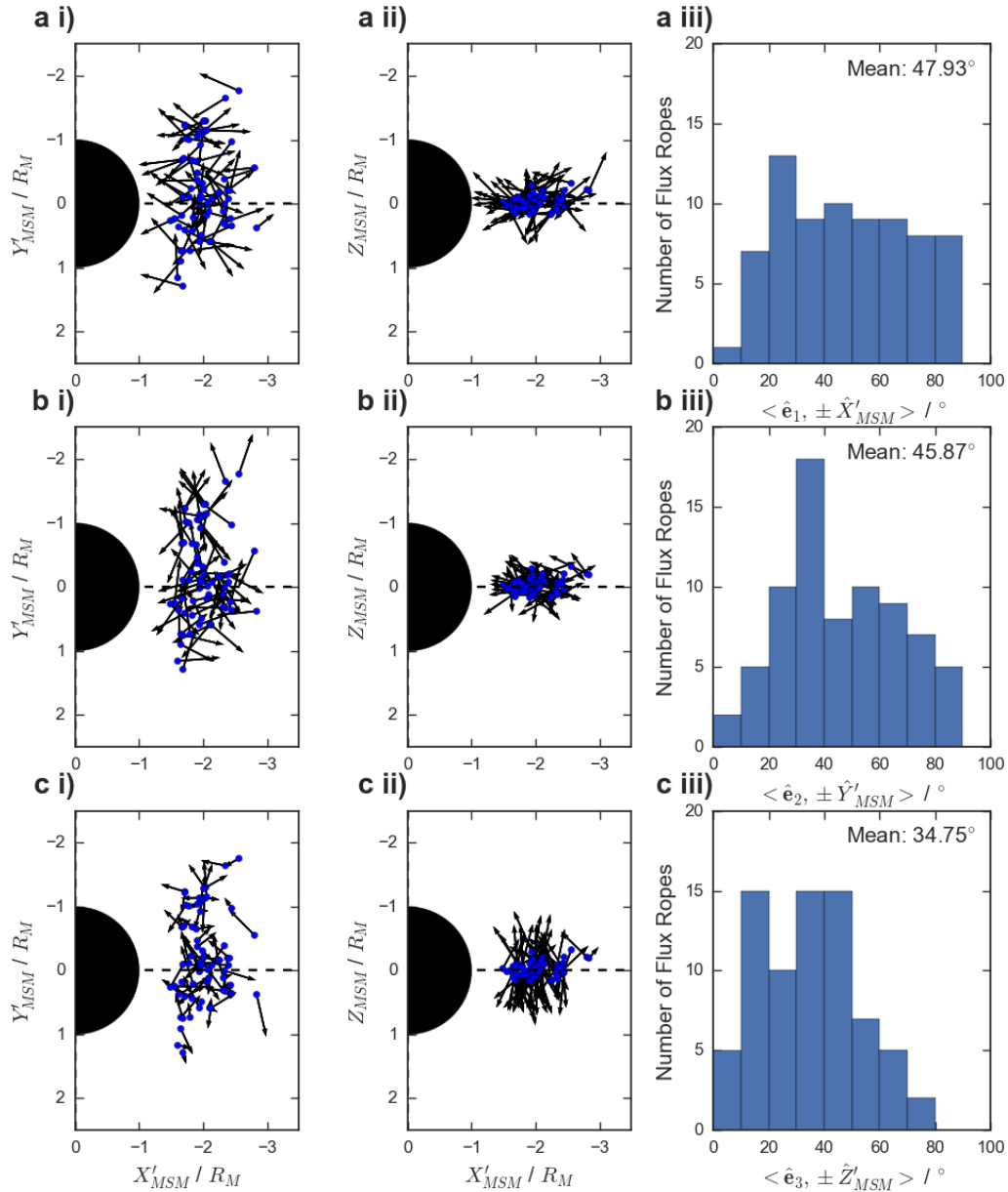
Figure 4. Minimum Variance Analysis (MVA) results for the 74 force-free flux ropes. The first two columns shows the X'_{MSM} - Y'_{MSM} and X'_{MSM} - Z'_{MSM} projections respectively. The right hand column shows the angular difference in degrees between the variance vectors and the relevant MSM base vector. The rows, from top to bottom, show the minimum, intermediate and maximum variance vectors.
