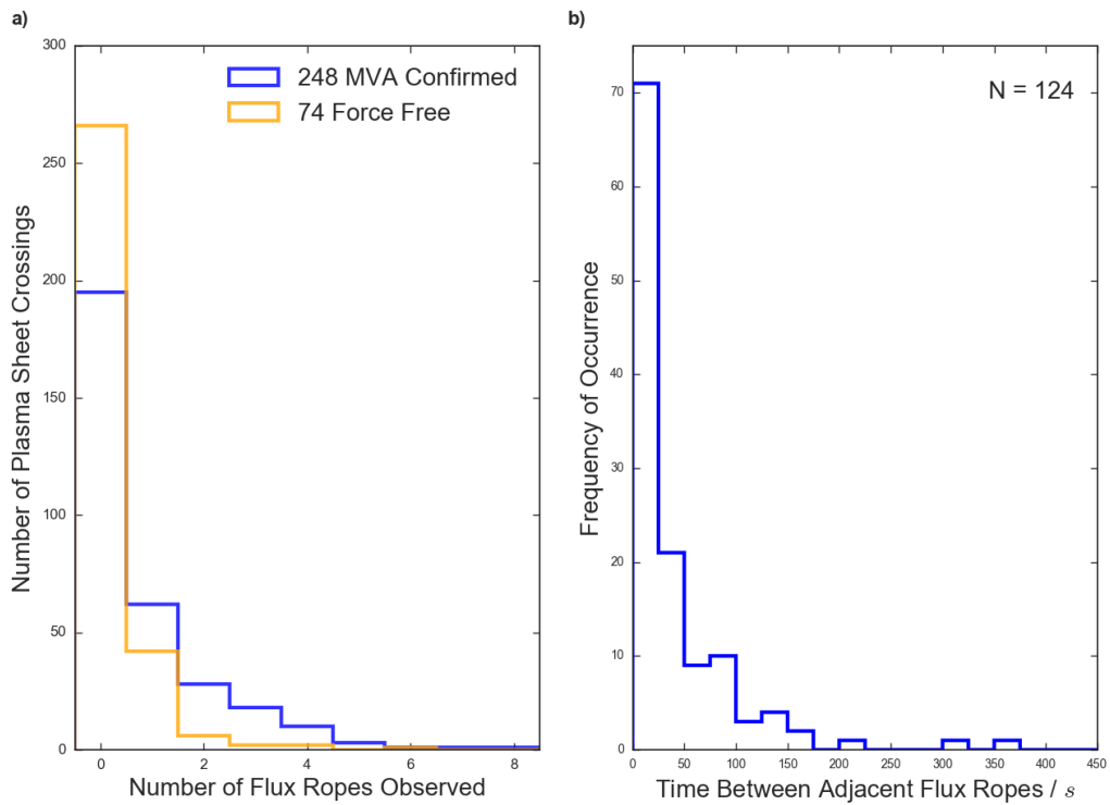
Figure 3. Panel (a) shows a histogram of the number of MVA confirmed (blue) and force-free (orange) flux ropes observed during each plasma sheet crossing. Panel (b) shows the distribution of times between adjacent MVA confirmed flux ropes.
