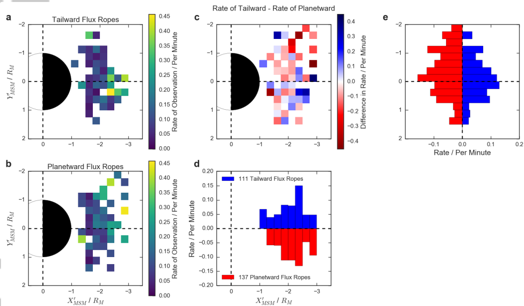
Figure 6. Histograms showing the rate of observation of 111 tailward (Panel a) and 137 planetward (Panel b) moving MVA confirmed flux ropes. Data are binned in 0.25 R_M increments and projected onto the equatorial plane of the MSM coordinate system. Panel (c) shows the rate of tailward moving flux ropes minus the rate of the planetward moving flux ropes. Positive (blue) values indicate regions where tailward moving flux ropes are observed more often, while negative (red) regions show locations where planetward moving flux ropes are more commonly observed. Panels (d) and (e) show the rates of planetward (red) and tailward (blue) moving flux ropes binned along the X'_{MSM} and Y'_{MSM} axes respectively.
