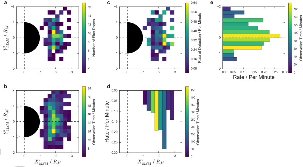
Figure 2. Histograms showing the distribution of 248 (MVA confirmed) flux ropes within the Hermean magnetotail. Data are binned in 0.25 R_M increments and projected onto the equatorial plane of the MSM coordinate system. Panel (a) describes the distribution of flux rope observations. Panel (b) shows the distribution of plasma sheet observations in minutes per spatial bin. Panel (c) shows the resulting rate of flux rope observations ( \# / T ). Panels (d) and (e) show the rate projected onto the X'_{MSM} and Y'_{MSM} axes respectively. The color bars for Panels (d) and (e) show the plasma sheet observation time projected onto the X'_{MSM} and Y'_{MSM} axes, this is shown to provide an approximate measure of how well determined (or how much data) has produced the rates for that region.
