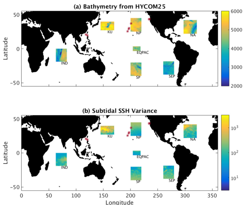
Figure 2. (a) HYCOM25 bathymetries (m) from seven regions used to compute frequency-horizontal wavenumber spectral densities overlaid on map of regions. Bathymetries from MITgcm48 are comparable. Abbreviations for the regions are listed in Table 3. Locations of nine McLane profilers are overlaid on map as red stars. (b) Low-frequency SSH variance ( \text{cm}^2 ) from HYCOM25 computed as in Savage et al. [2017] in seven regions used in study.
