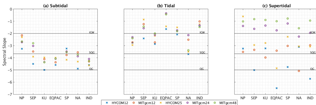
Figure 10. Spectral slopes computed from all five simulations in the (a) subtidal, (b) tidal, and (c) supertidal frequency bands. Slopes were computed over wavenumbers ranging from 1/250 to 1/70 cpkm in the subtidal and tidal bands, and over wavenumbers ranging from 1/70 to 1/30 cpkm in the supertidal band. Abbreviations for the regions are listed in Table 3.
