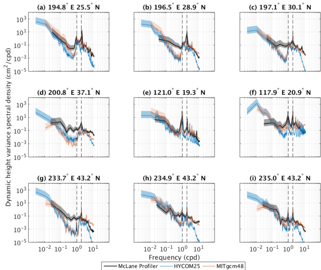
Figure 3. Dynamic height variance frequency spectral densities from McLane profilers and nearest neighbor HYCOM25 and MITgcm48 grid points. The dashed vertical lines denote K_1 diurnal and M_2 semidiurnal tidal frequencies. The shaded regions are the 95% confidence intervals that account only for random error in spectral density calculations.
