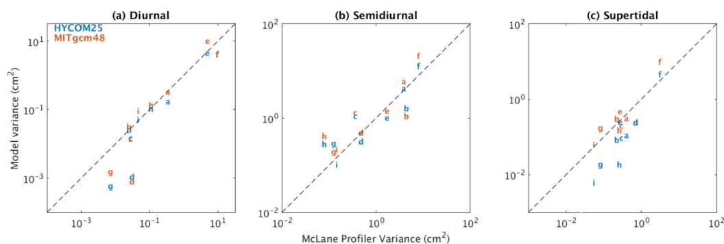
Figure 4. Scatterplots of band-integrated dynamic height variance vs. McLane profilers in 1/25° HYCOM and 1/48° MITgcm in (a) diurnal, (b) semidiurnal, and (c) supertidal frequency bands. Letters on scatterplots correspond to profiler locations listed in Table 1.
