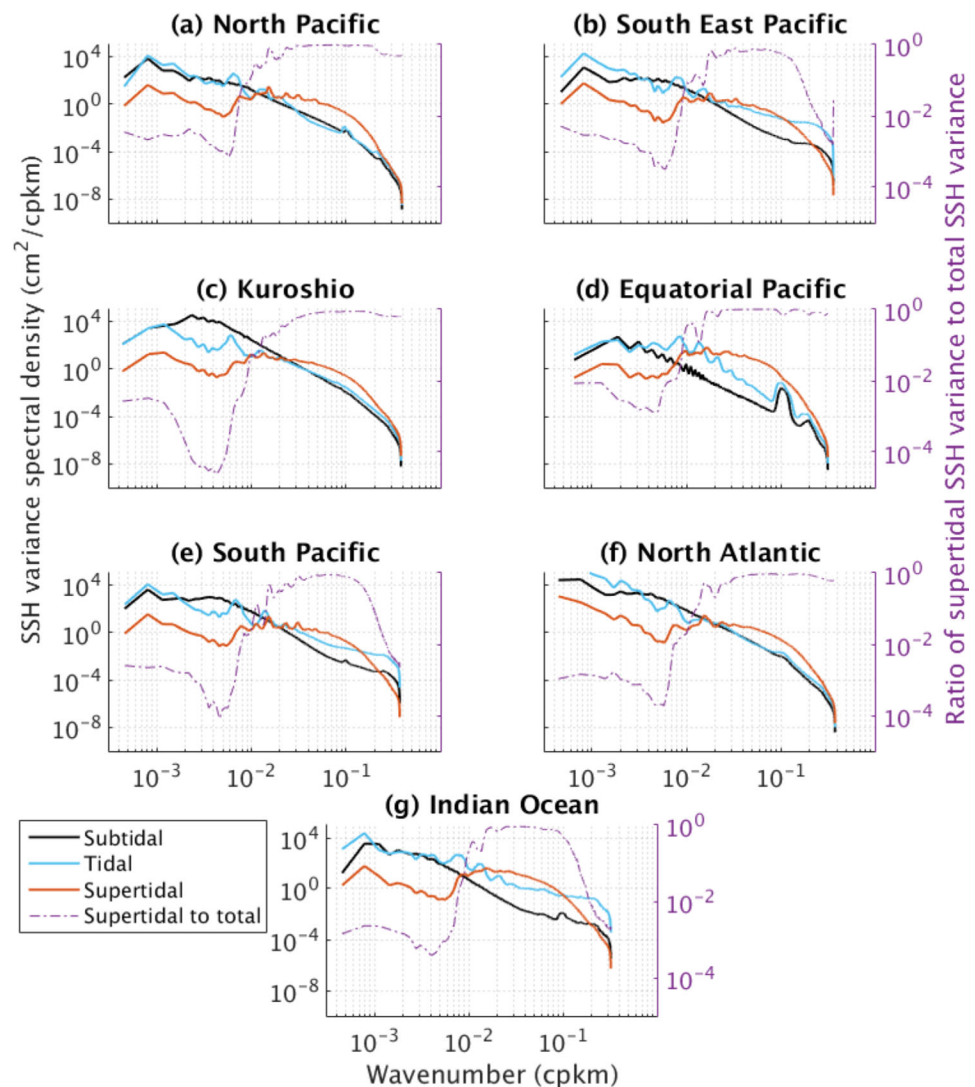
Figure 7. Horizontal wavenumber spectral density of SSH variance in all regions in MITgcm48 integrated over subtidal, tidal, and supertidal frequency bands (see text for definition of bands). The 95% confidence intervals span 76%–137% of shown value for the subtidal band, 85%–119% for the tidal band, and 94%–107% for the supertidal band. Right-hand axis shows ratio of supertidal to total SSH variance as a function of isotropic wavenumber.
