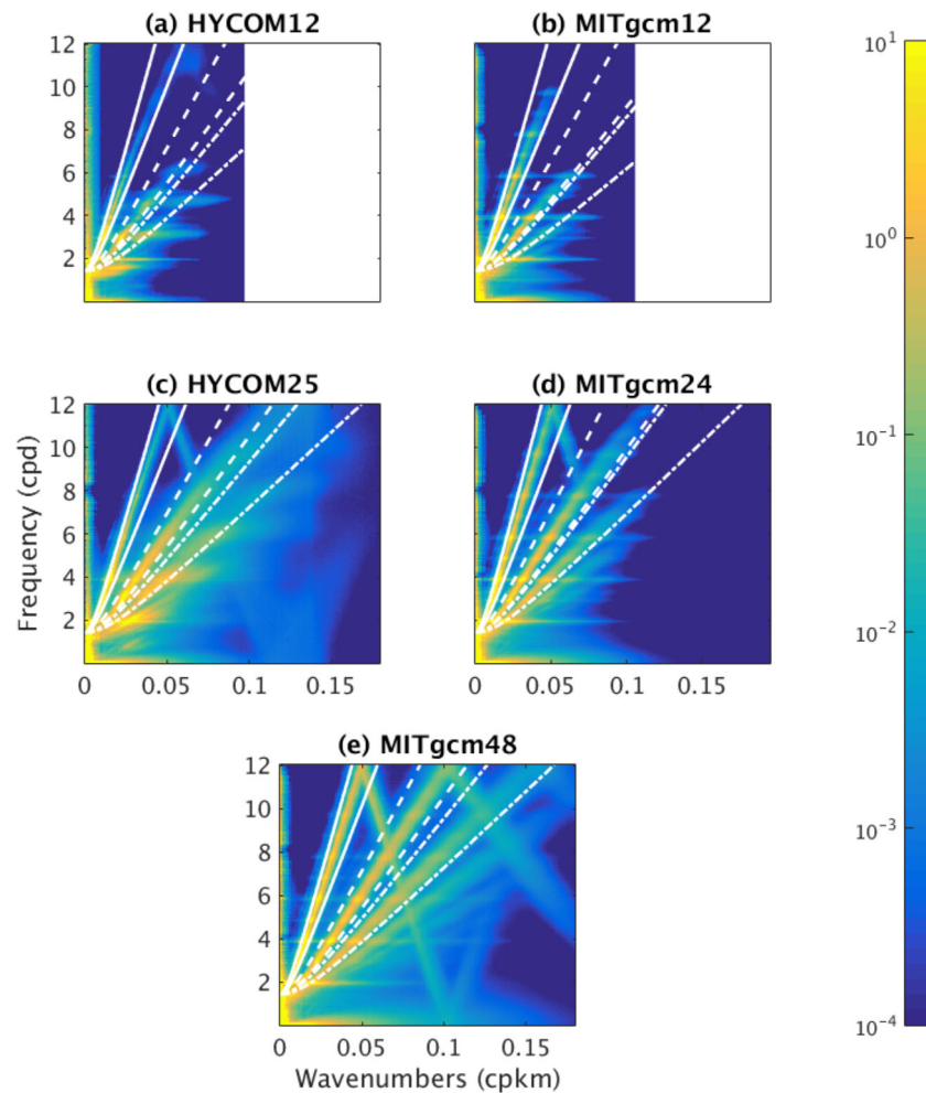
Figure 6. Sea surface height variance frequency-horizontal wavenumber spectral density ( \text{cm}^2 / (\text{cpd cpkm}) ) computed in North Pacific region in all five simulations. Wavenumber axes are the same in each plot, and are set to the maximum wavenumber for the HYCOM25 calculation. White curves show theoretical IGW linear dispersion relations for first (solid), second (dashed), and third (dashed-dotted) vertical modes. Bounding curves for each vertical mode are computed from the maximal and minimal eigenspeeds along the northern and southern boundaries, as in Müller et al. [2015].
