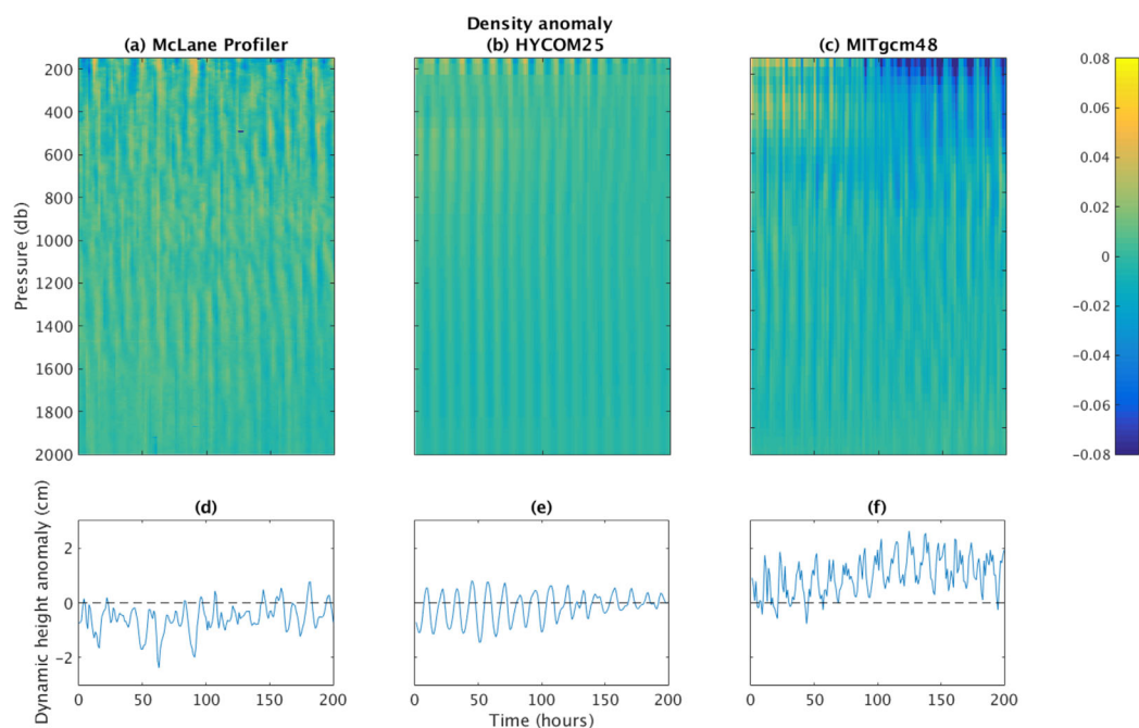
Figure 1. Density anomaly profile time series ( \text{kg}/\text{m}^3 ) over the pressure intervals sampled by the McLane profiler located at 233.7^\circ\text{E} , 43.2^\circ\text{N} from (a) a McLane profiler, (b) HYCOM25, and (c) MITgcm48. The bottom row displays time series of dynamic height anomaly (cm) computed as in equation (1) for (d) a McLane profiler, (e) HYCOM25, and (f) MITgcm48. Data are shown from the first 200 h of each data set and are therefore shown over different time intervals (September for Figures 1a and 1d, January for Figures 1b and 1e, and October for Figures 1c and 1f).
