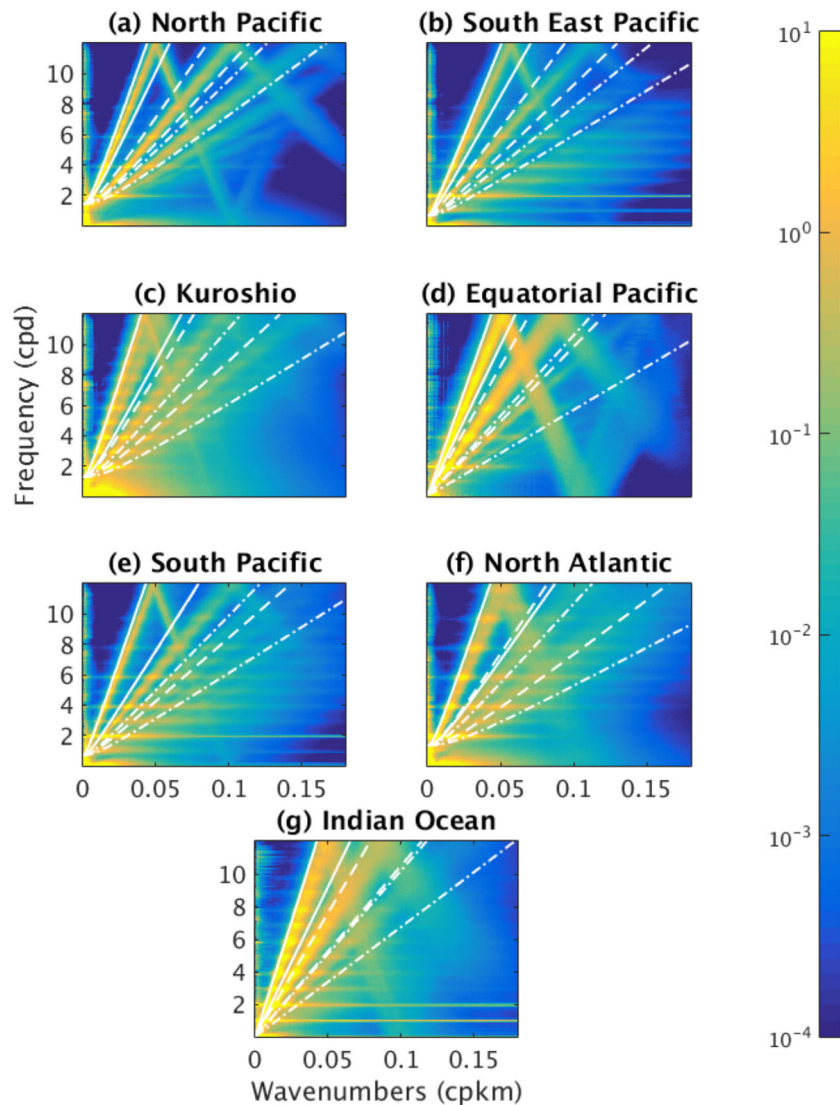
Figure 5. Sea surface height variance frequency-horizontal wavenumber spectral density ( \text{cm}^2 / (\text{cpd cpkm}) ) computed over seven regions from MITgcm48. Wavenumber axes are set to the maximum wavenumber for each region computed in HYCOM25. White curves show theoretical IGW linear dispersion relations for first (solid), second (dashed), and third (dashed-dotted) vertical modes. Bounding curves for each vertical mode are computed from the maximal and minimal eigenspeeds along the northern and southern boundaries, as in Müller et al. [2015].
