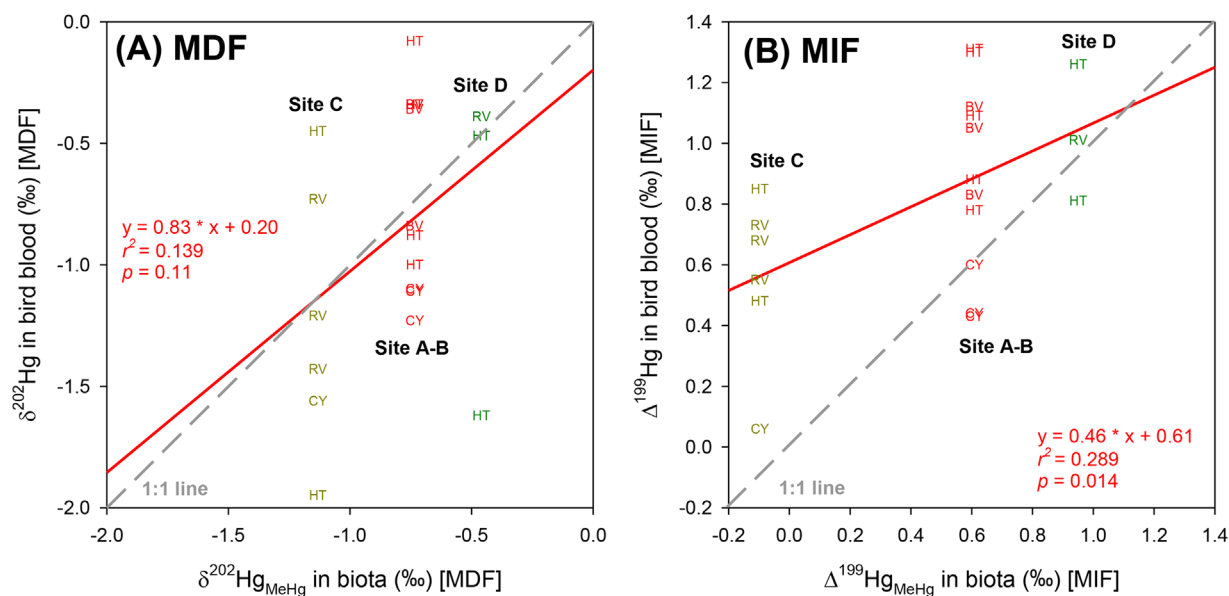
FIGURE 5: Relationship between bird blood mercury (Hg) isotope data and those of mean Hg isotope data in each habitat where bird samples were collected (site A-B, site C, site D). (A) Mass-dependent fractionation (MDF). (B) Mass-independent fractionation (MIF). Data are denoted as bird species; CY = common yellowthroat; HT = hermit thrush; BV = blue-headed vireo; RV = red-eyed vireo. Note that all non-bird data at sites A and B are included for comparing bird blood samples from site A-B. Regression line is shown as red solid line. Dashed shaded line indicates 1:1 relationship.
