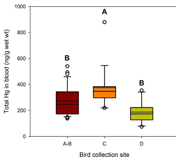
FIGURE 2: Box plot (including outliers) of total mercury (Hg) data in all bird blood samples ( n=49 ; note that only 20 samples were analyzed for Hg isotopes) among the 3 sampling sites. Means for a treatment are not significantly different ( p > 0.05 ) if they bear the same letter.
