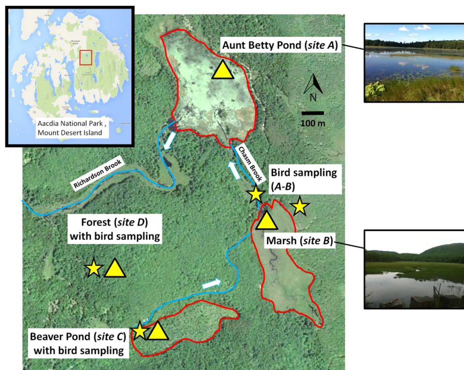
FIGURE 1: Locations of sampling sites in the Acadia National Park. Triangle denotes non-bird biota sampling and star denotes bird sampling at Aunt Betty Pond (site A, without bird collection), Marsh (site B, without bird collection), Beaver Pond (site C, with bird collection), and Forest (site D, with bird collection). Bird sampling was performed at 2 locations between site A and site B, and is denoted as a single site A-B.
