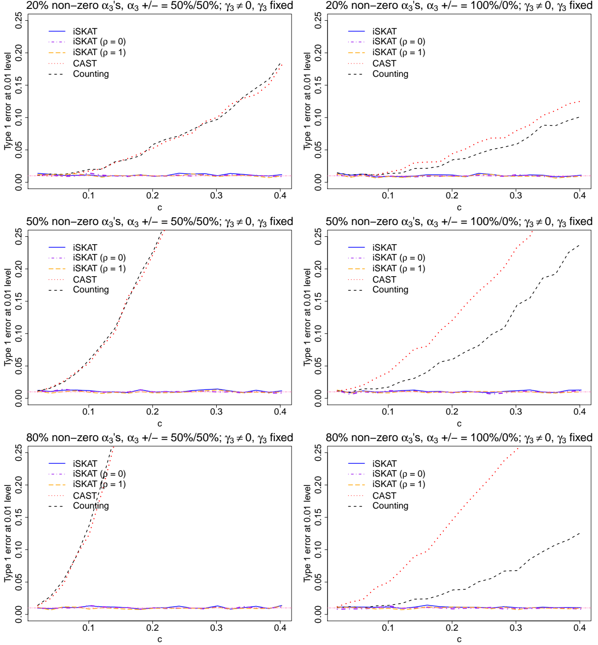
Web Figure 14: Empirical Type 1 error rates at \alpha = 0.01 nominal level for continuous outcome when \mathbf{G} and E are dependent and there are main effects for n = 4000 - iSKAT (solid line), iSKAT with \rho = 0 (dashed-and-dotted line), iSKAT with \rho = 1 (long dashed line), CAST (dotted line) and Counting (short dashed line). Top panel - 20% non-zero \alpha_{3j} 's; Middle panel - 50% non-zero \alpha_{3j} 's; Bottom panel - 80% non-zero \alpha_{3j} 's. Left panel - 50% of \alpha_{3j} 's are positive; Right panel - 100% of \alpha_{3j} 's are positive. \gamma_{3j} = 0.4 \text{sgn}(\alpha_{3j}) |\log_{10} \text{MAF}_j| . \alpha_3 controls the association between \mathbf{G} and Y . \gamma_3 controls the association between \mathbf{G} and E . As c increases, the \mathbf{G} - Y association increases but \mathbf{G} - E association remains fixed. Since there are main effects for rare variants, iSKAT gives a correct Type 1 error rate but burden tests can have inflated Type 1 error rates. Bias of burden tests increase with increasing \mathbf{G} - Y association when \mathbf{G} and E are dependent.
