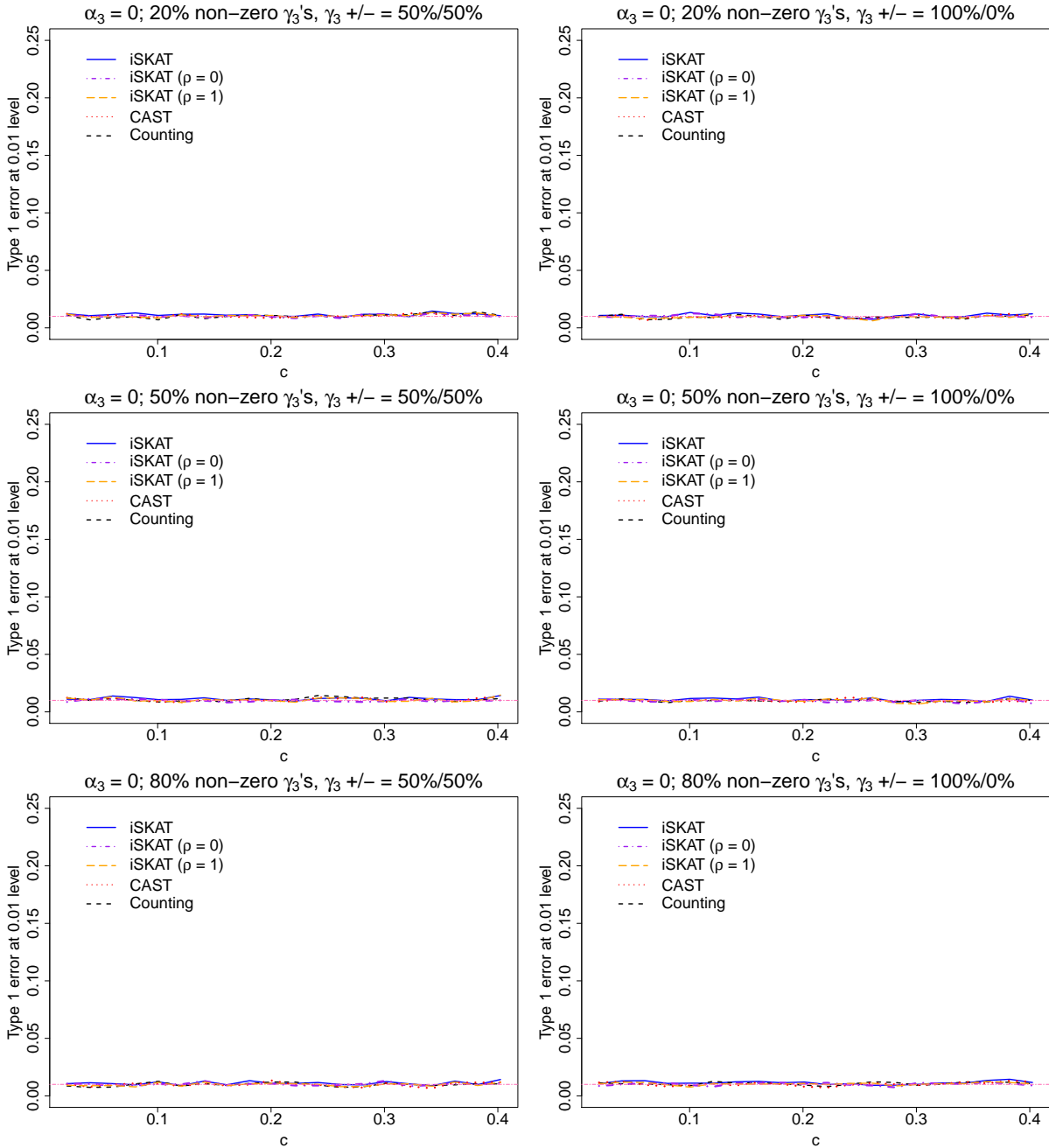
Web Figure 7: Empirical Type 1 error rates at \alpha = 0.01 nominal level for continuous outcome when \mathbf{G} and E are dependent and there are no main effects for n = 2000 - iSKAT (solid line), iSKAT with \rho = 0 (dashed-and-dotted line), iSKAT with \rho = 1 (long dashed line), CAST (dotted line) and Counting (short dashed line). Top panel - 20% non-zero \gamma_{3j} 's; Middle panel - 50% non-zero \gamma_{3j} 's; Bottom panel - 80% non-zero \gamma_{3j} 's. Left panel - 50% of \gamma_{3j} 's are positive; Right panel - 100% of \gamma_{3j} 's are positive. \alpha_3 = 0 . \gamma_3 controls the association between \mathbf{G} and E . As c increases, the \mathbf{G} - E association increases. Since there are no main effects for rare variants, all five methods have correct Type 1 error rates.
