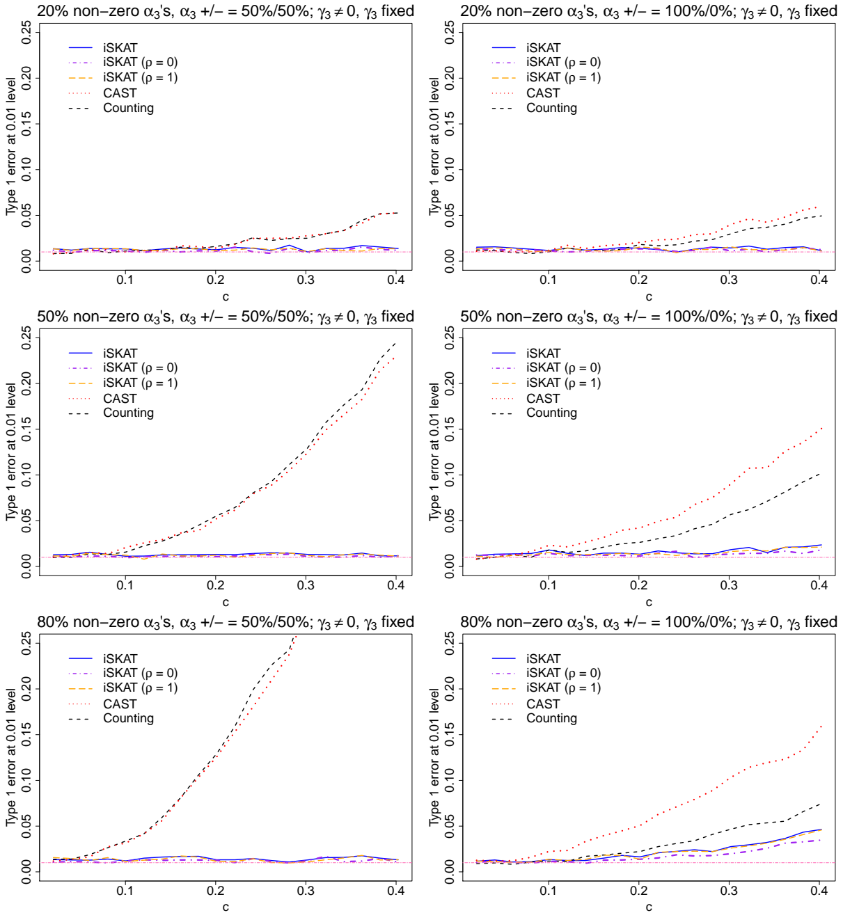
Web Figure 24: Empirical Type 1 error rates at \alpha = 0.01 nominal level for binary outcome when \mathbf{G} and E are dependent and there are main effects for n = 4000 - iSKAT (solid line), iSKAT with \rho = 0 (dashed-and-dotted line), iSKAT with \rho = 1 (long dashed line), CAST (dotted line) and Counting (short dashed line). Top panel - 20% non-zero \alpha_{3j} 's; Middle panel - 50% non-zero \alpha_{3j} 's; Bottom panel - 80% non-zero \alpha_{3j} 's. Left panel - 50% of \alpha_{3j} 's are positive; Right panel - 100% of \alpha_{3j} 's are positive. \gamma_{3j} = 0.4 \text{sgn}(\alpha_{3j}) |\log_{10} \text{MAF}_j| . \alpha_3 controls the association between \mathbf{G} and Y . \gamma_3 controls the association between \mathbf{G} and E . As c increases, the \mathbf{G} - Y association increases but \mathbf{G} - E association remains fixed. Since there are main effects for rare variants and \mathbf{G} and E are dependent, iSKAT gives a correct Type 1 error rate but burden tests can have inflated Type 1 error rates. Bias of burden tests increase with increasing \mathbf{G} - Y association when \mathbf{G} and E are dependent.
