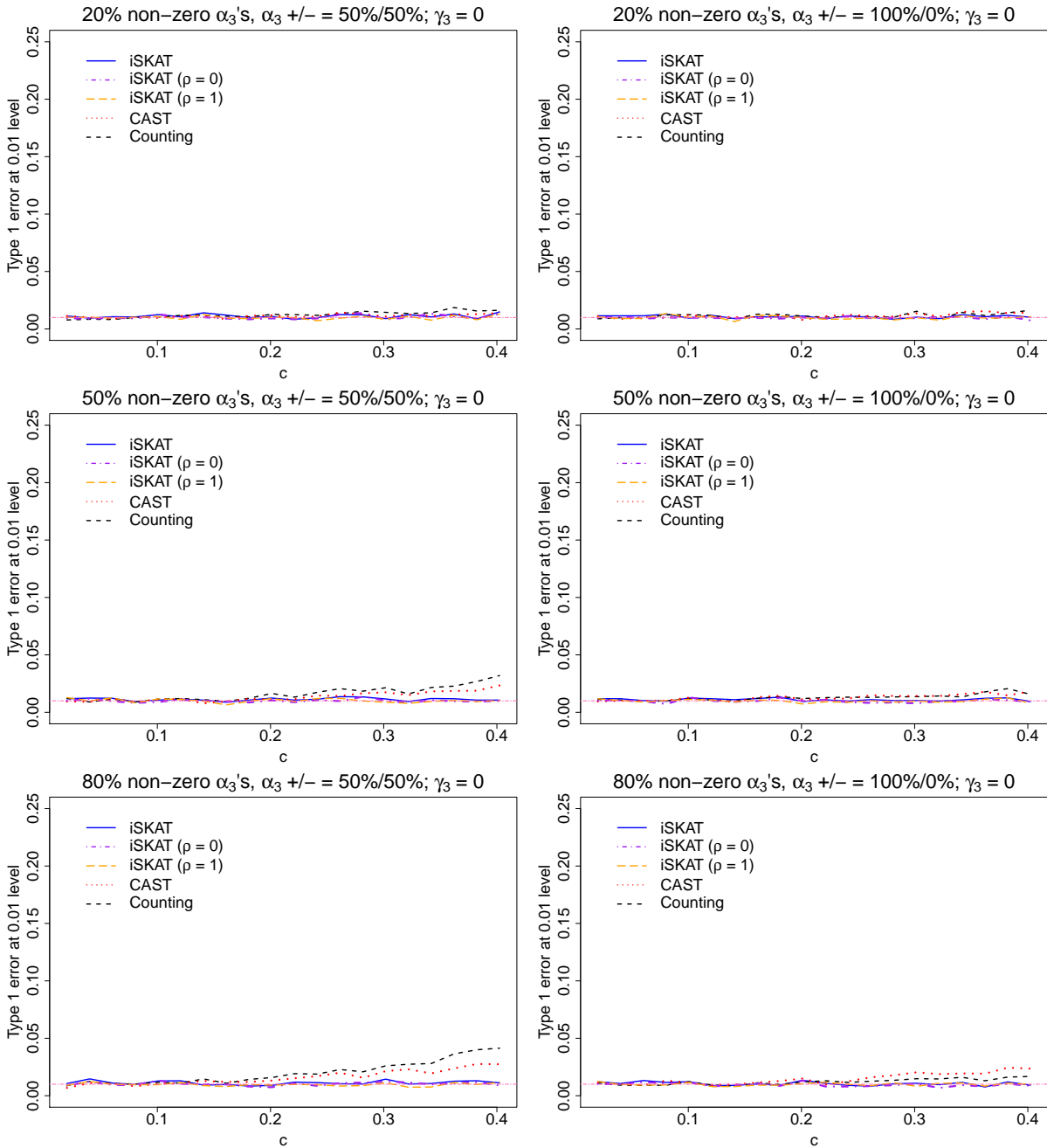
Web Figure 10: Empirical Type 1 error rates at \alpha = 0.01 nominal level for continuous outcome when \mathbf{G} and E are independent and there are main effects for n = 4000 - iSKAT (solid line), iSKAT with \rho = 0 (dashed-and-dotted line), iSKAT with \rho = 1 (long dashed line), CAST (dotted line) and Counting (short dashed line). Top panel - 20% non-zero \alpha_{3j} 's; Middle panel - 50% non-zero \alpha_{3j} 's; Bottom panel - 80% non-zero \alpha_{3j} 's. Left panel - 50% of \alpha_{3j} 's are positive; Right panel - 100% of \alpha_{3j} 's are positive. \gamma_3 = \mathbf{0} . \alpha_3 controls the association between \mathbf{G} and Y . As c increases, the \mathbf{G} - Y association increases. Since there are main effects for rare variants, iSKAT gives a correct Type 1 error rate but burden tests can have inflated Type 1 error rates.
