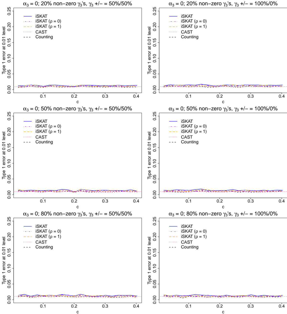
Web Figure 18: Empirical Type 1 error rates at \alpha = 0.01 nominal level for binary outcome when \mathbf{G} and E are dependent and there are no main effects for n = 4000 - iSKAT (solid line), iSKAT with \rho = 0 (dashed-and-dotted line), iSKAT with \rho = 1 (long dashed line), CAST (dotted line) and Counting (short dashed line). Top panel - 20% non-zero \gamma_{3j} 's; Middle panel - 50% non-zero \gamma_{3j} 's; Bottom panel - 80% non-zero \gamma_{3j} 's. Left panel - 50% of \gamma_{3j} 's are positive; Right panel - 100% of \gamma_{3j} 's are positive. \alpha_3 = \mathbf{0} . \gamma_3 controls the association between \mathbf{G} and E . As c increases, the \mathbf{G} - E association increases. Since there are no main effects for rare variants, all five methods have correct Type 1 error rates.
