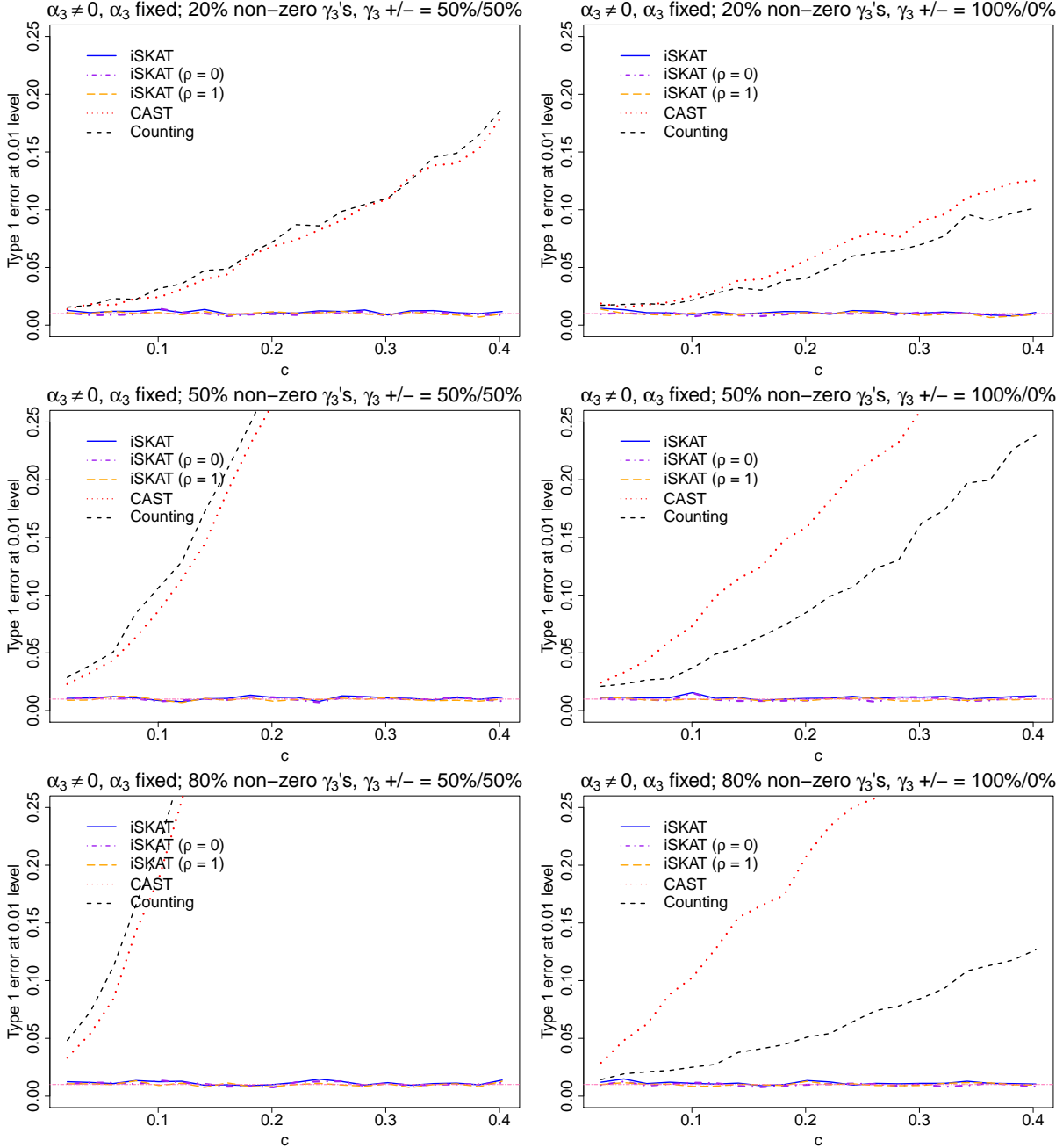
Web Figure 16: Empirical Type 1 error rates at \alpha = 0.01 nominal level for continuous outcome when \mathbf{G} and E are dependent and there are main effects for n = 4000 - iSKAT (solid line), iSKAT with \rho = 0 (dashed-and-dotted line), iSKAT with \rho = 1 (long dashed line), CAST (dotted line) and Counting (short dashed line). Top panel - 20% non-zero \gamma_{3j} 's; Middle panel - 50% non-zero \gamma_{3j} 's; Bottom panel - 80% non-zero \gamma_{3j} 's. Left panel - 50% of \gamma_{3j} 's are positive; Right panel - 100% of \gamma_{3j} 's are positive. \alpha_{3j} = 0.4\text{sgn}(\gamma_{3j})|\log_{10} \text{MAF}_j| . \alpha_3 controls the association between \mathbf{G} and Y . \gamma_3 controls the association between \mathbf{G} and E . As c increases, the \mathbf{G} - E association increases but \mathbf{G} - Y association remains fixed. Since there are main effects for rare variants, iSKAT gives a correct Type 1 error rate but burden tests can have inflated Type 1 error rates. Bias of burden tests increase with increasing \mathbf{G} - E association when \mathbf{G} and Y are associated.
