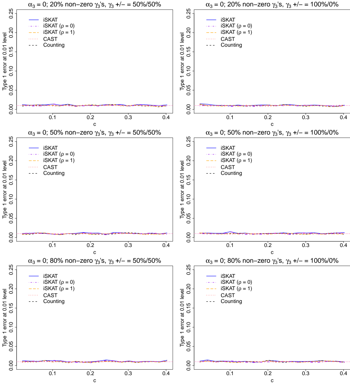
Web Figure 8: Empirical Type 1 error rates at \alpha = 0.01 nominal level for continuous outcome when \mathbf{G} and E are dependent and there are no main effects for n = 4000 - iSKAT (solid line), iSKAT with \rho = 0 (dashed-and-dotted line), iSKAT with \rho = 1 (long dashed line), CAST (dotted line) and Counting (short dashed line). Top panel - 20% non-zero \gamma_{3j} 's; Middle panel - 50% non-zero \gamma_{3j} 's; Bottom panel - 80% non-zero \gamma_{3j} 's. Left panel - 50% of \gamma_{3j} 's are positive; Right panel - 100% of \gamma_{3j} 's are positive. \alpha_3 = 0 . \gamma_3 controls the association between \mathbf{G} and E . As c increases, the \mathbf{G} - E association increases. Since there are no main effects for rare variants, all five methods have correct Type 1 error rates.
