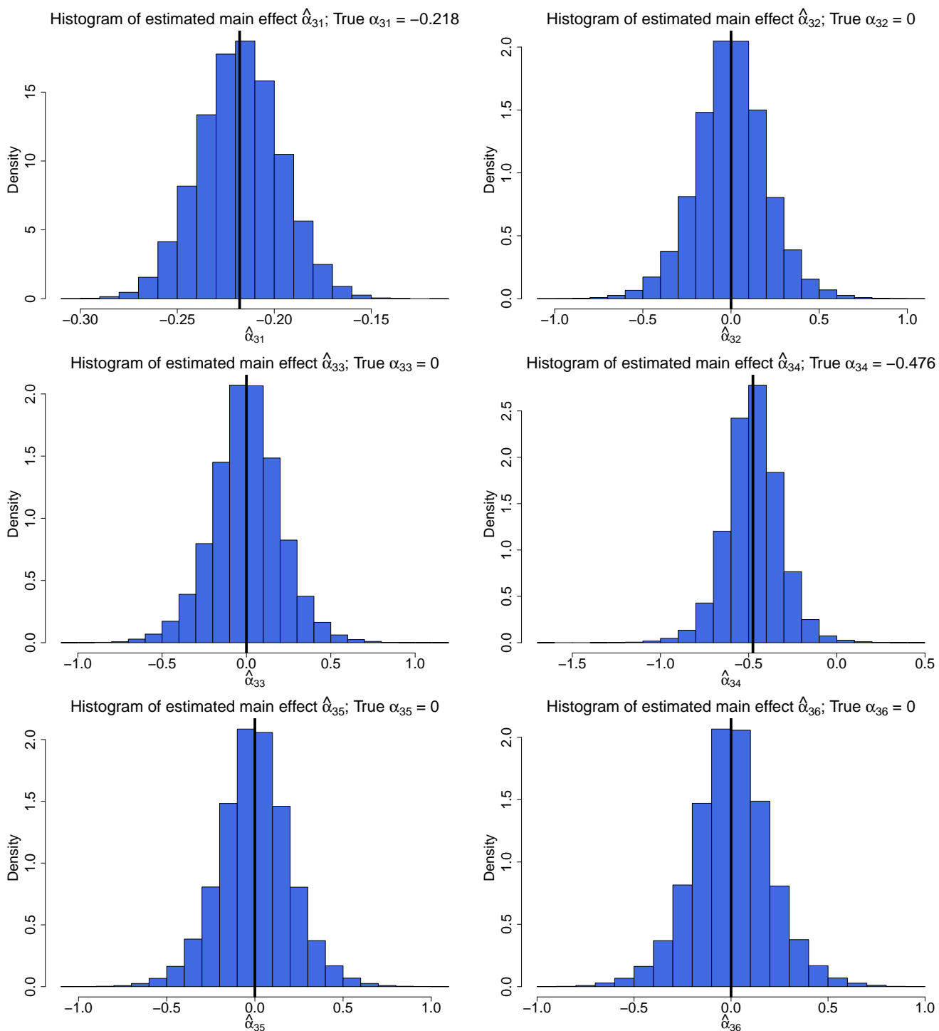
Web Figure 3: Histograms of estimated rare variants main effects \hat{\alpha}_3 from iSKAT, for continuous outcome when there are rare variants main effects, for n = 4000 . True rare variants main effect sizes \alpha_3 are indicated with vertical lines. This figure gives \hat{\alpha}_{3j} for j = 1 - 6 while Web Figure 4 gives \hat{\alpha}_{3j} for j = 7 - 11 . Datasets were generated by sampling the genotypes and covariates jointly with replacement from the CoLaus dataset to preserve the association between \mathbf{G} and E . Note that the p-value for the association between \mathbf{G} and E in the CoLaus dataset was 0.042, which suggests plausible \mathbf{G} - E dependence. Estimated rare variants main effects \hat{\alpha}_3 are similar to the true rare variants main effects \alpha_3 .
