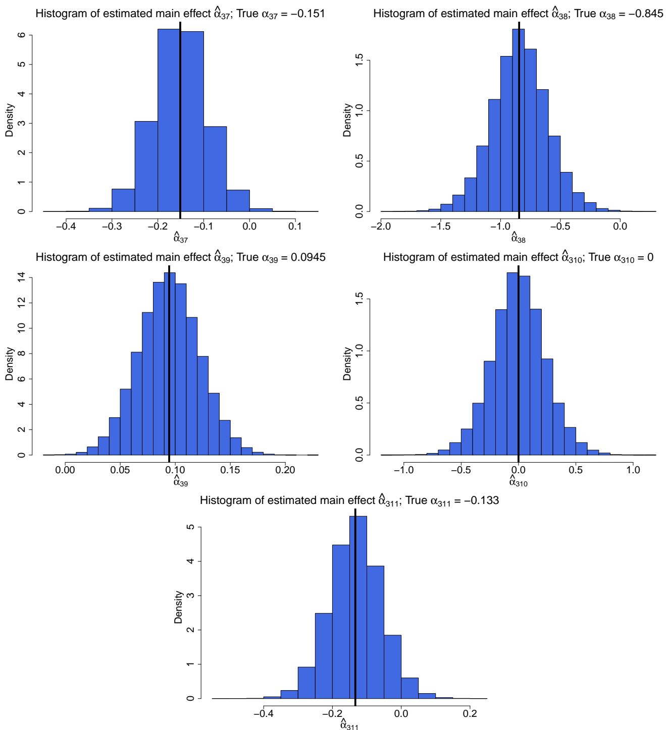
Web Figure 2: Histograms of estimated rare variants main effects \hat{\alpha}_3 from iSKAT, for continuous outcome when there are rare variants main effects, for n = 1945 . True rare variants main effect sizes \alpha_3 are indicated with vertical lines. This figure gives \hat{\alpha}_{3j} for j = 7 - 11 while Web Figure 1 gives \hat{\alpha}_{3j} for j = 1 - 6 . Datasets were generated by sampling the genotypes and covariates jointly with replacement from the CoLaus dataset to preserve the association between \mathbf{G} and E . Note that the p-value for the association between \mathbf{G} and E in the CoLaus dataset was 0.042, which suggests plausible \mathbf{G} - E dependence. Estimated rare variants main effects \hat{\alpha}_3 are similar to the true rare variants main effects \alpha_3 .
