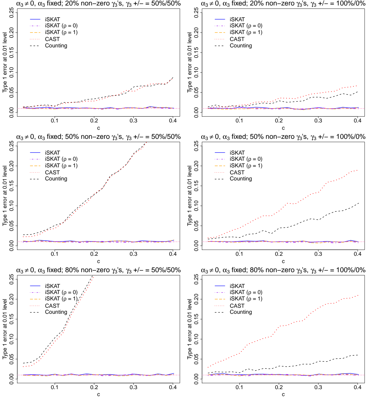
Web Figure 15: Empirical Type 1 error rates at \alpha = 0.01 nominal level for continuous outcome when \mathbf{G} and E are dependent and there are main effects for n = 2000 - iSKAT (solid line), iSKAT with \rho = 0 (dashed-and-dotted line), iSKAT with \rho = 1 (long dashed line), CAST (dotted line) and Counting (short dashed line). Top panel - 20% non-zero \gamma_{3j} 's; Middle panel - 50% non-zero \gamma_{3j} 's; Bottom panel - 80% non-zero \gamma_{3j} 's. Left panel - 50% of \gamma_{3j} 's are positive; Right panel - 100% of \gamma_{3j} 's are positive. \alpha_{3j} = 0.4\text{sgn}(\gamma_{3j})|\log_{10}\text{MAF}_j| . \alpha_3 controls the association between \mathbf{G} and Y . \gamma_3 controls the association between \mathbf{G} and E . As c increases, the \mathbf{G} - E association increases but \mathbf{G} - Y association remains fixed. Since there are main effects for rare variants, iSKAT gives a correct Type 1 error rate but burden tests can have inflated Type 1 error rates. Bias of burden tests increase with increasing \mathbf{G} - E association when \mathbf{G} and Y are associated.
