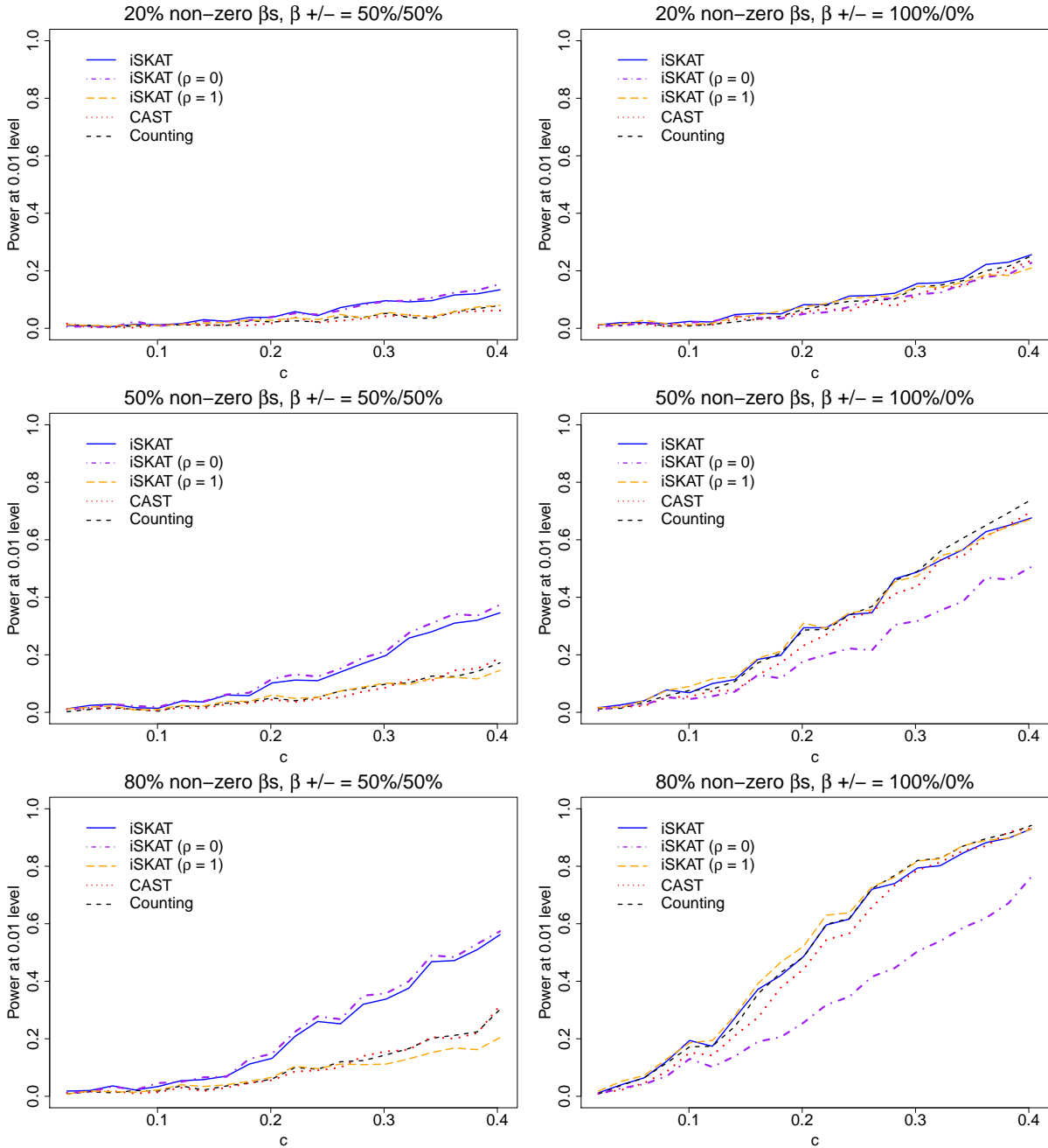
Web Figure 30: Empirical power curves at n = 4000 for \alpha = 0.01 level of significance for binary outcome when \mathbf{G} and E are independent and there are no main effects (i.e. \alpha_3 = \gamma_3 = \mathbf{0} ) - iSKAT (solid line), iSKAT with \rho = 0 (dashed-and-dotted line), iSKAT with \rho = 1 (long dashed line), CAST (dotted line) and Counting (short dashed line). Top panel - 20% non-zero \beta_j 's; Middle panel - 50% non-zero \beta_j 's; Bottom panel - 80% non-zero \beta_j 's. Left panel - 50% of \beta_j 's are positive; Right panel - 100% of \beta_j 's are positive.
