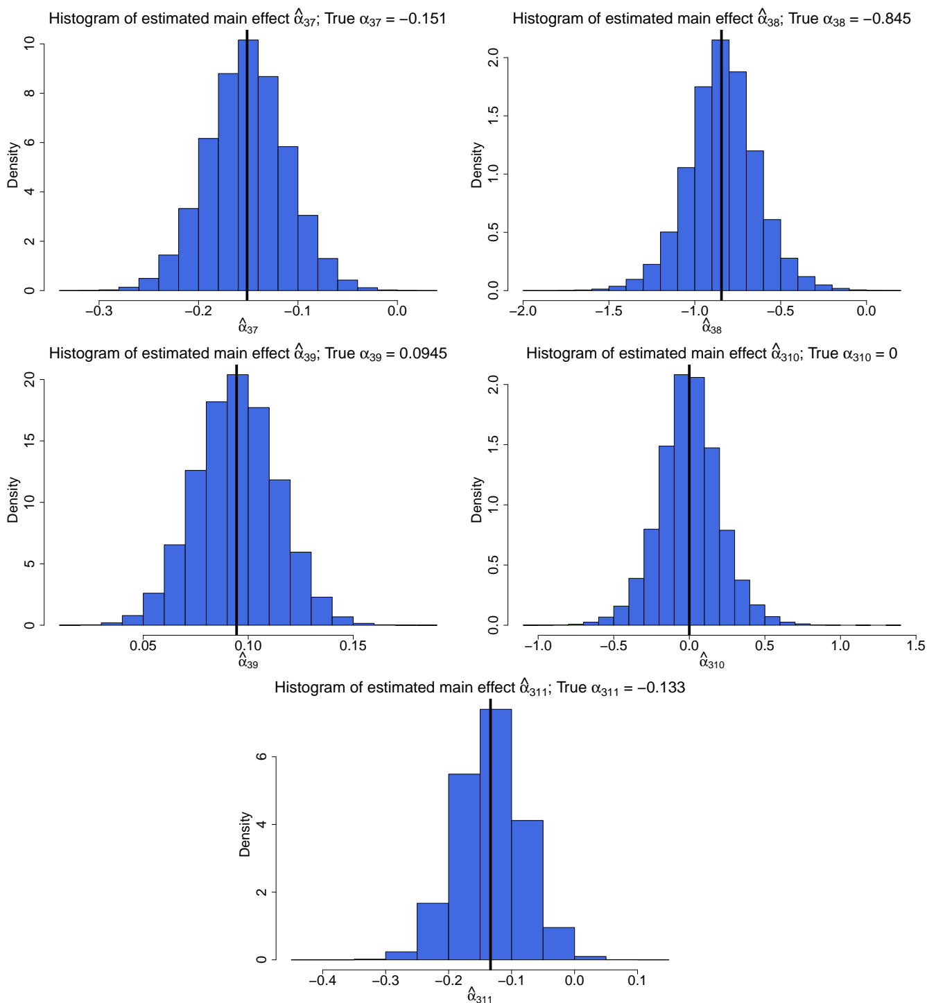
Web Figure 4: Histograms of estimated rare variants main effects \hat{\alpha}_3 from iSKAT, for continuous outcome when there are rare variants main effects for, n = 4000 . True rare variants main effect sizes \alpha_3 are indicated with vertical lines. This figure gives \hat{\alpha}_{3j} for j = 7 - 11 while Web Figure 3 gives \hat{\alpha}_{3j} for j = 1 - 6 . Datasets were generated by sampling the genotypes and covariates jointly with replacement from the CoLaus dataset to preserve the association between \mathbf{G} and E . Note that the p-value for the association between \mathbf{G} and E in the CoLaus dataset was 0.042, which suggests plausible \mathbf{G} - E dependence. Estimated rare variants main effects \hat{\alpha}_3 are similar to the true rare variants main effects \alpha_3 .
