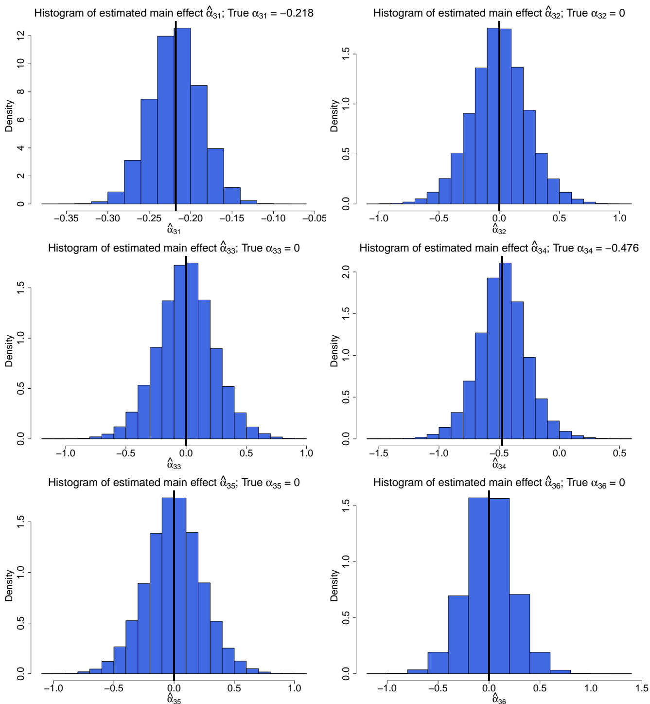
Web Figure 1: Histograms of estimated rare variants main effects \hat{\alpha}_3 from iSKAT, for continuous outcome when there are rare variants main effects, for n = 1945 . True rare variants main effect sizes \alpha_3 are indicated with vertical lines. This figure gives \hat{\alpha}_{3j} for j = 1 - 6 while Web Figure 2 gives \hat{\alpha}_{3j} for j = 7 - 11 . Datasets were generated by sampling the genotypes and covariates jointly with replacement from the CoLaus dataset to preserve the association between \mathbf{G} and E . Note that the p-value for the association between \mathbf{G} and E in the CoLaus dataset was 0.042, which suggests plausible \mathbf{G} - E dependence. Estimated rare variants main effects \hat{\alpha}_3 are similar to the true rare variants main effects \alpha_3 .
