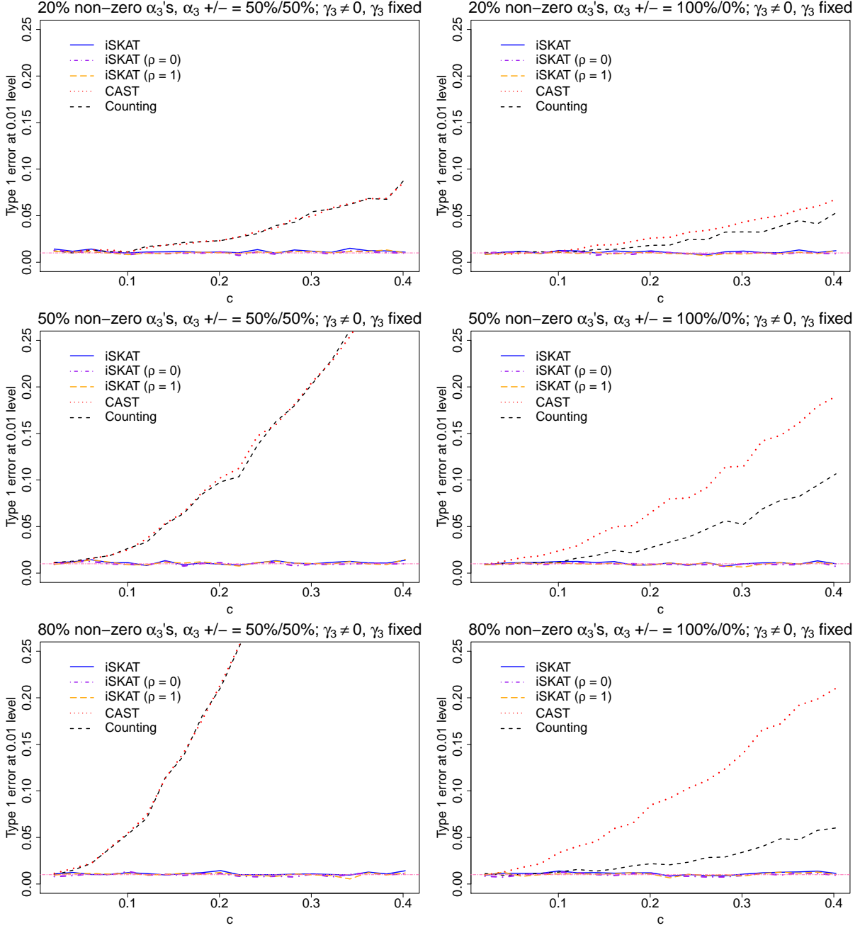
Web Figure 13: Empirical Type 1 error rates at \alpha = 0.01 nominal level for continuous outcome when \mathbf{G} and E are dependent and there are main effects for n = 2000 - iSKAT (solid line), iSKAT with \rho = 0 (dashed-and-dotted line), iSKAT with \rho = 1 (long dashed line), CAST (dotted line) and Counting (short dashed line). Top panel - 20% non-zero \alpha_{3j} 's; Middle panel - 50% non-zero \alpha_{3j} 's; Bottom panel - 80% non-zero \alpha_{3j} 's. Left panel - 50% of \alpha_{3j} 's are positive; Right panel - 100% of \alpha_{3j} 's are positive. \gamma_{3j} = 0.4 \text{sgn}(\alpha_{3j}) |\log_{10} \text{MAF}_j| . \alpha_3 controls the association between \mathbf{G} and Y . \gamma_3 controls the association between \mathbf{G} and E . As c increases, the \mathbf{G} - Y association increases but \mathbf{G} - E association remains fixed. Since there are main effects for rare variants, iSKAT gives a correct Type 1 error rate but burden tests can have inflated Type 1 error rates. Bias of burden tests increase with increasing \mathbf{G} - Y association when \mathbf{G} and E are dependent.
