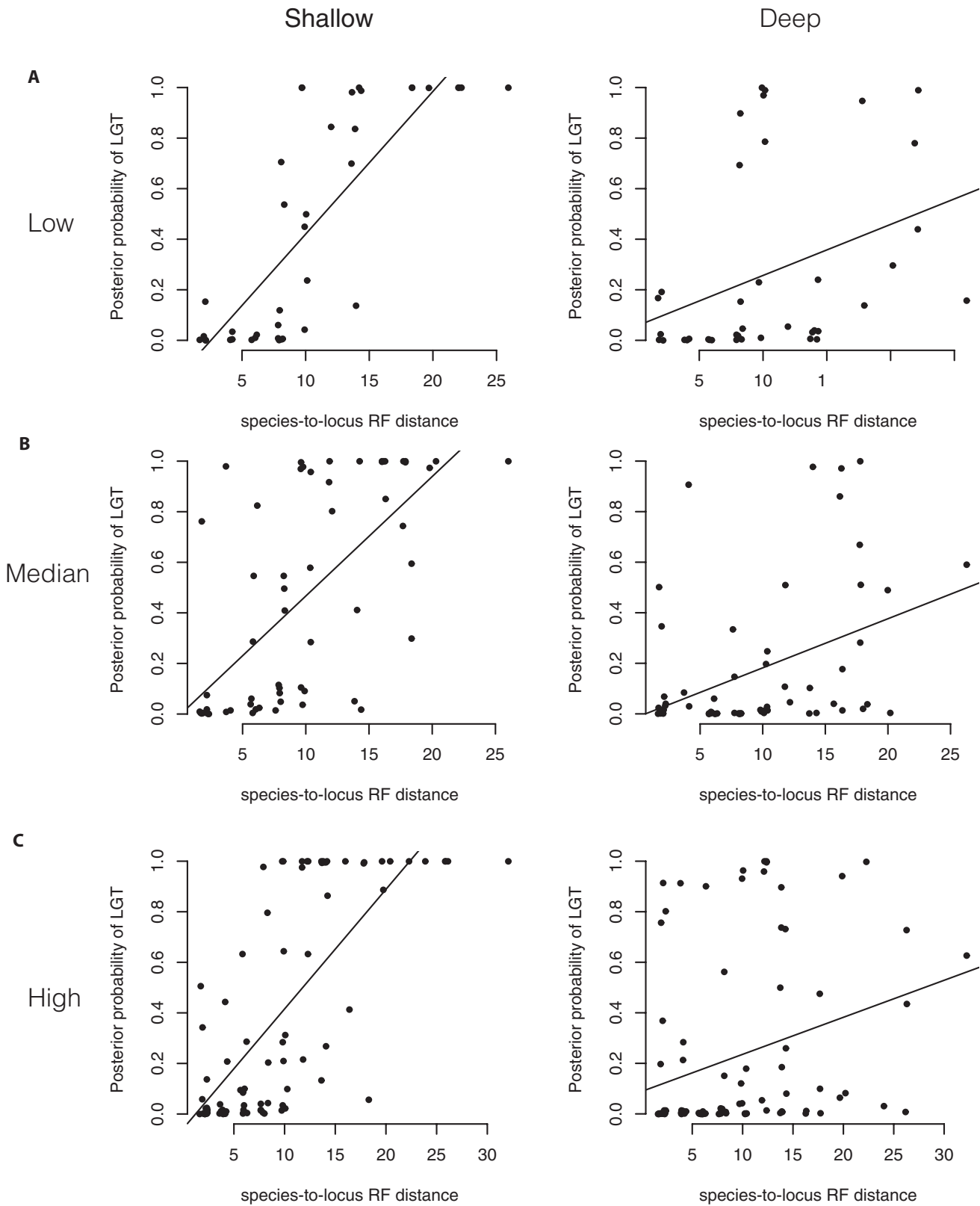
FIGURE 3. Variation in the classification performance among gene trees as a function of the Robinson-Fould's distance between each gene tree and the species tree (i.e., each dot shows the posterior probability of lateral gene transfer [LGT]) when species divergence is relatively recent (shown on the left) compared to deeper divergence times (show on the right), for (A) low, (B) medium, and (C) high relative proportions of LGT loci.
