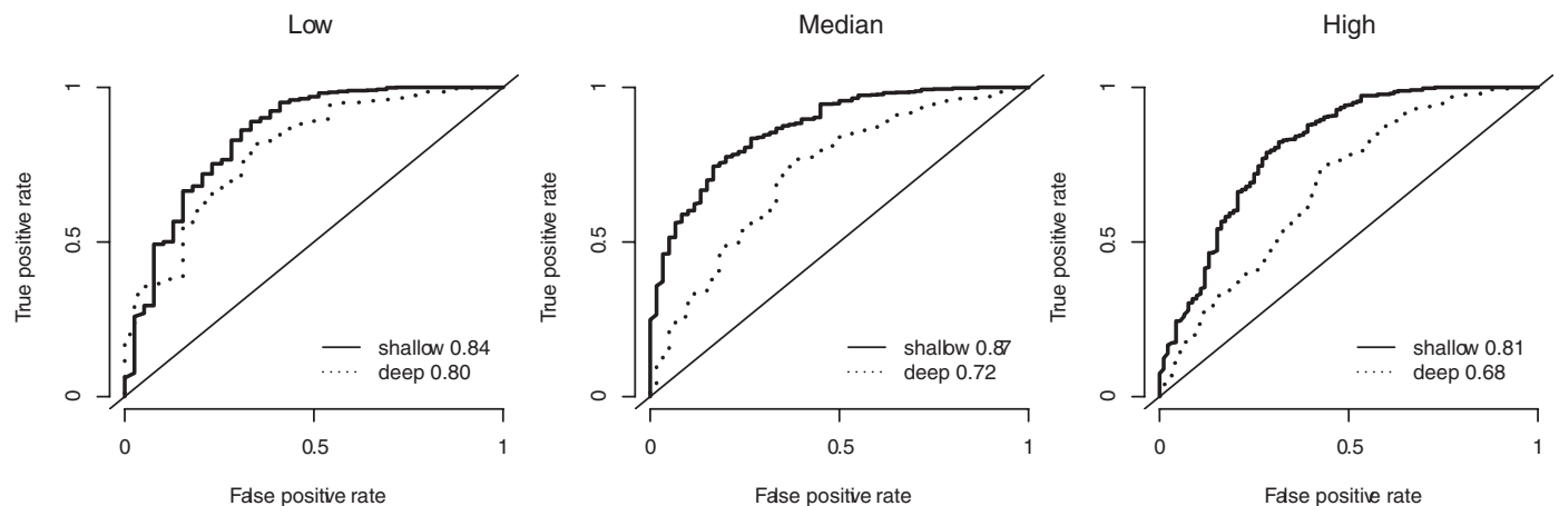
FIGURE 2. Classification performance when species divergence is relatively recent (i.e., shallow; shown in the solid line) compared to deeper divergence times (shown in the dotted line) for different contributions of lateral gene transfer (LGT) to gene tree discord, ranging from low, medium, and high relative proportions of LGT loci, as characterized by the receiver operating characteristic (ROC) curve. A classifier with no power will sit on the diagonal (i.e., essentially random guessing, 0.5, whether a locus is an incomplete lineage sorting [ILS] versus LGT locus). The area under the curve (AUC) scores (with a maximum value of 1) are also shown for comparison of the accuracy of the classifier in distinguishing ILS versus LGT loci (presented next to the solid and dashed lines) for shallow versus deep histories.
