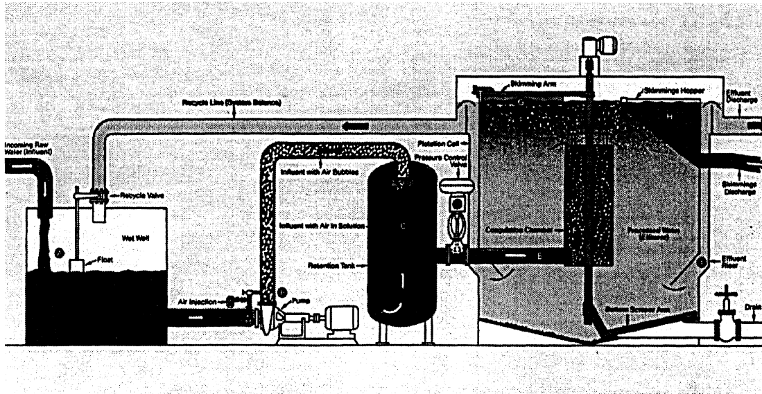
Figure 3. Sample DAF System
