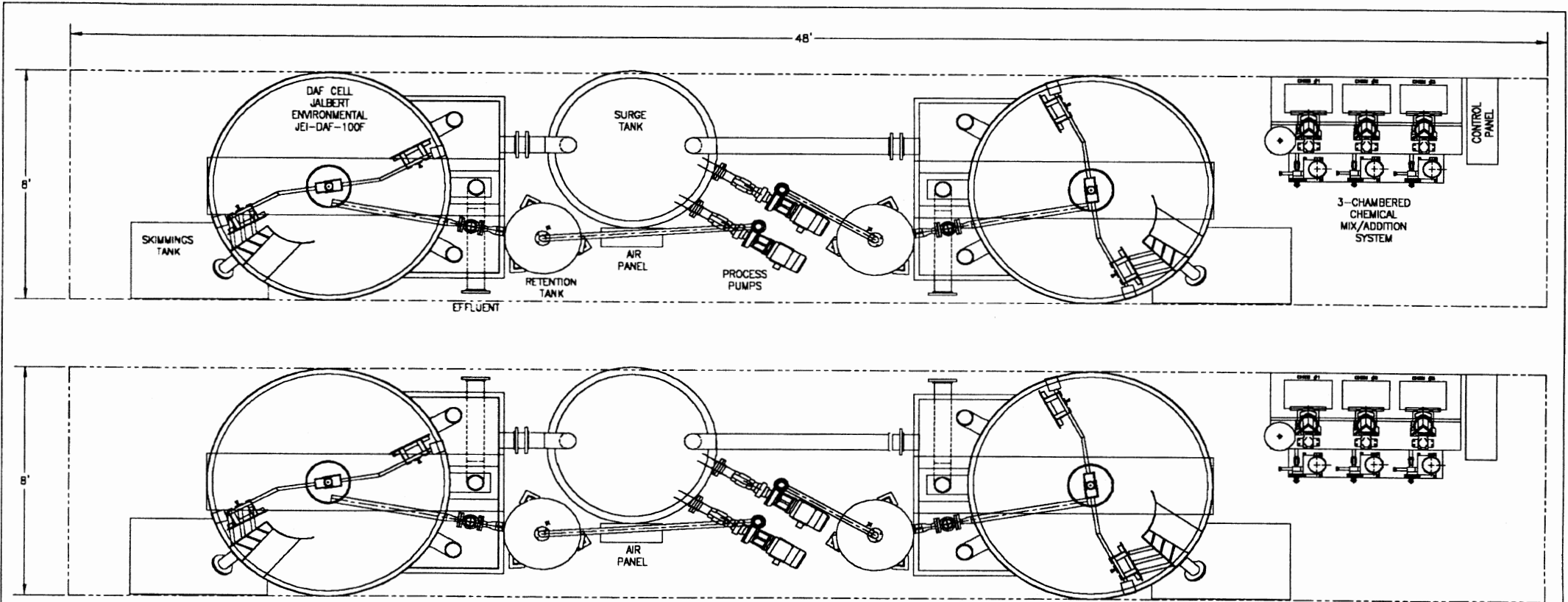
CONCEPTUAL 400 GPM (500 GPM MAX.) FULL FLOW DAF SYSTEM TWIN 200 GPM (250 GPM MAX. SEE NOTE) FULL FLOW DAF WITH INTEGRAL CHEMICAL MIX/FEEED SYSTEM
