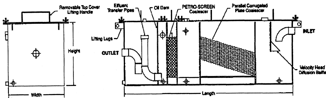
Figure 2. Sample Coalescing Tank
