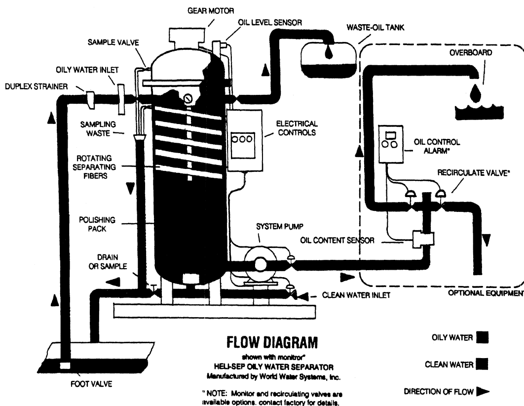
Figure 1. Sample Oil/Water Separator
