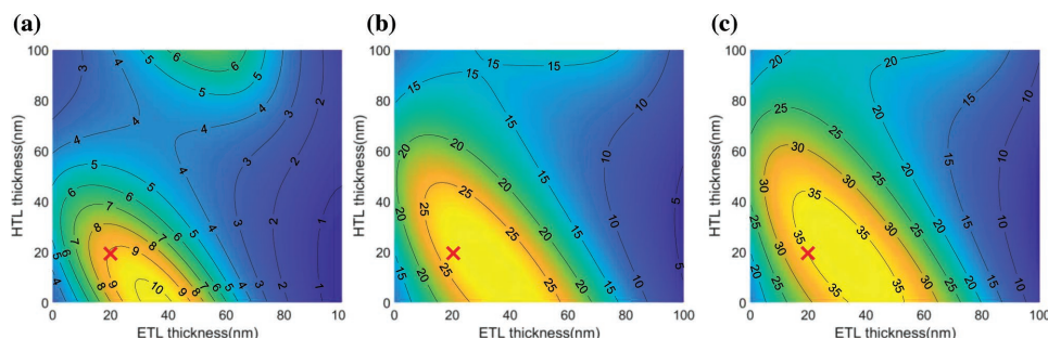
Figure 5. Simulations of the external quantum efficiencies of a) CzTrz, b) BCzTrz, and c) TCzTrz, versus hole (HTL) and electron transport layer (ETL) thicknesses of the OLEDs. The experimental OLEDs are indicated by "X."
