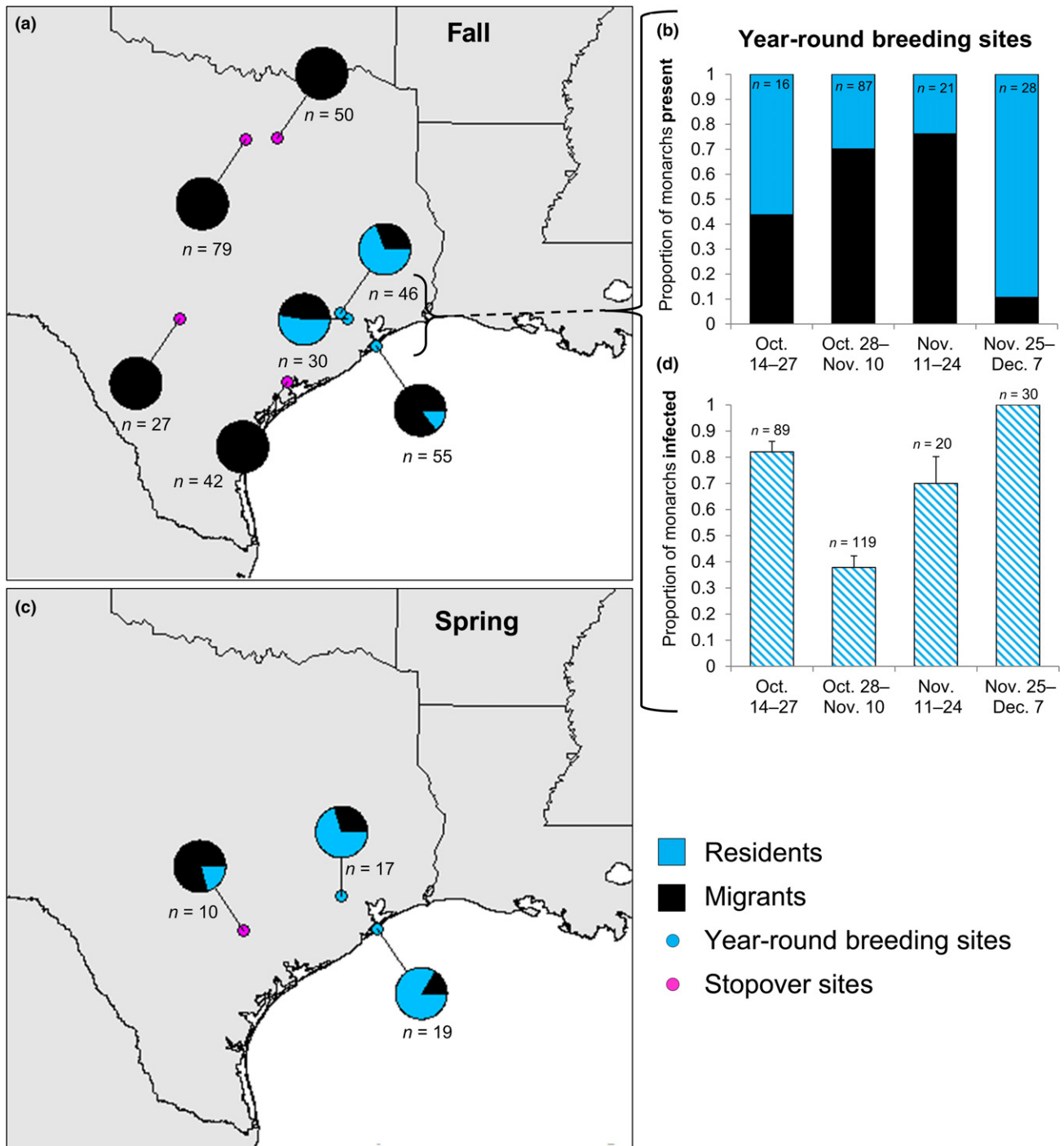
Figure 1 Map of sampling locations in Texas, USA from (a) fall 2014 and (c) spring 2015, with the proportion of sampled adult monarchs that were assigned migrant status (black) or resident status (blue) at year-round breeding sites (blue points) and seasonal stopover sites (pink points). (b) Temporal changes in the proportion of migrants vs. residents at year-round breeding sites during the fall. (d) Temporal changes in infection prevalence of adult monarchs at year-round breeding sites during the fall.
