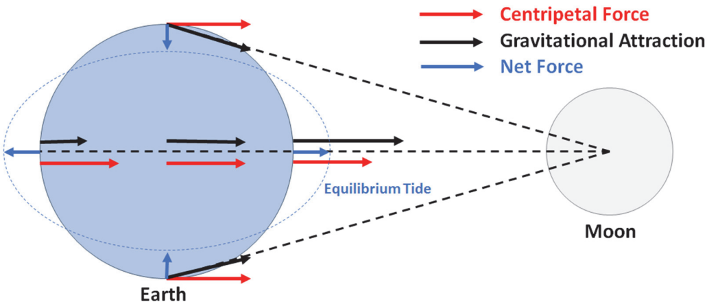
Figure 13.10. Tide-producing forces.
