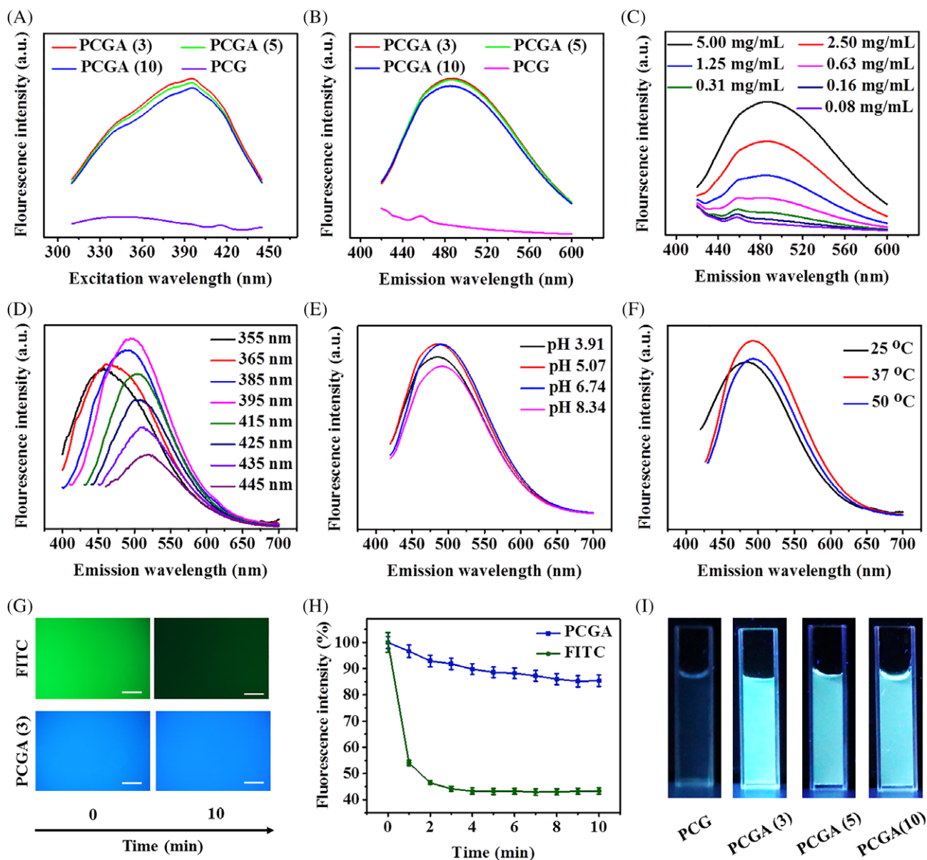
FIGURE 3. Intrinsically photoluminescent ability of PCGA polymers. (A) Excitation spectra of PCG and PCGA polymers in deionized water under the emission wavelength of 490 nm; (B) Emission spectra of PCG and PCGA polymers in deionized water under the excitation wavelength of 395 nm; (C–F) Emission spectra of PCGA (3) polymer in deionized water under different concentrations (C), excitation wavelengths (D), pH values (E), temperatures (F); (G) Fluorescent images of PCGA (3) polymer irradiated for different time intervals by an inverted fluorescent microscope under 405 nm excitation (scale bar:100 \mu m); (H) Fluorescent stability after irradiated for various times by a high pressure mercury lamp (365 nm); (I) Fluorescent images of PCG and PCGA polymers in deionized water (1.25 mg/mL) under 365 nm excitation by a UV lamp.
