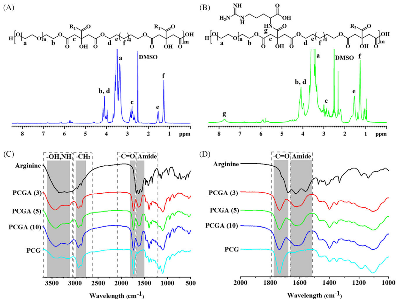
FIGURE 2. Chemical structure characterization of PCG and PCGA polymers. (A, B) ^1\text{H} NMR spectra of PCG prepolymer (A) and PCGA polymer (B); (C, D) FT-IR spectra of arginine, PCG and PCGA polymers between 3800\text{--}500\text{ cm}^{-1} (C) and 2000\text{--}1000\text{ cm}^{-1} (D).
