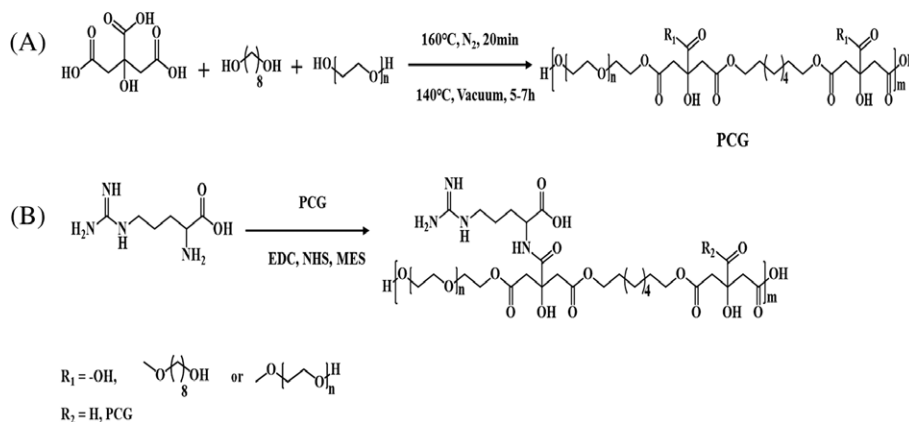
FIGURE 1. Schematic illustrations for synthesizing PCG and PCGA polymers. (A) Polymerization routine of PCG prepolymer; (B) Polymerization process of PCGA polymer through a representative EDC/NHS reaction.
