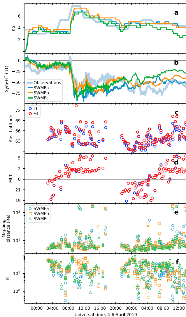
Figure 4. Isotropic boundary (IB) parameters and geomagnetic indices as a function of time. (a) Kp index, observed and simulated, (b) Sym-H^* index, observed and simulated, (c) absolute value of magnetic latitude of the IB observations, (d) magnetic local time of the IB observations, (e) maximum downtail distance of the field lines mapped from the IB locations, for each of the three magnetohydrodynamic simulations, and (f) K computed from the magnetohydrodynamic solution at the farthest point of each field line.
