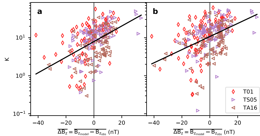
Figure 6. K as a function of \overline{\Delta B_z} for the empirical models, computed for locations mapped from isotropic boundary observations in the high-latitude data set (a) and low-latitude data set (b). The black lines show a linear fit (in log space) to the data.
