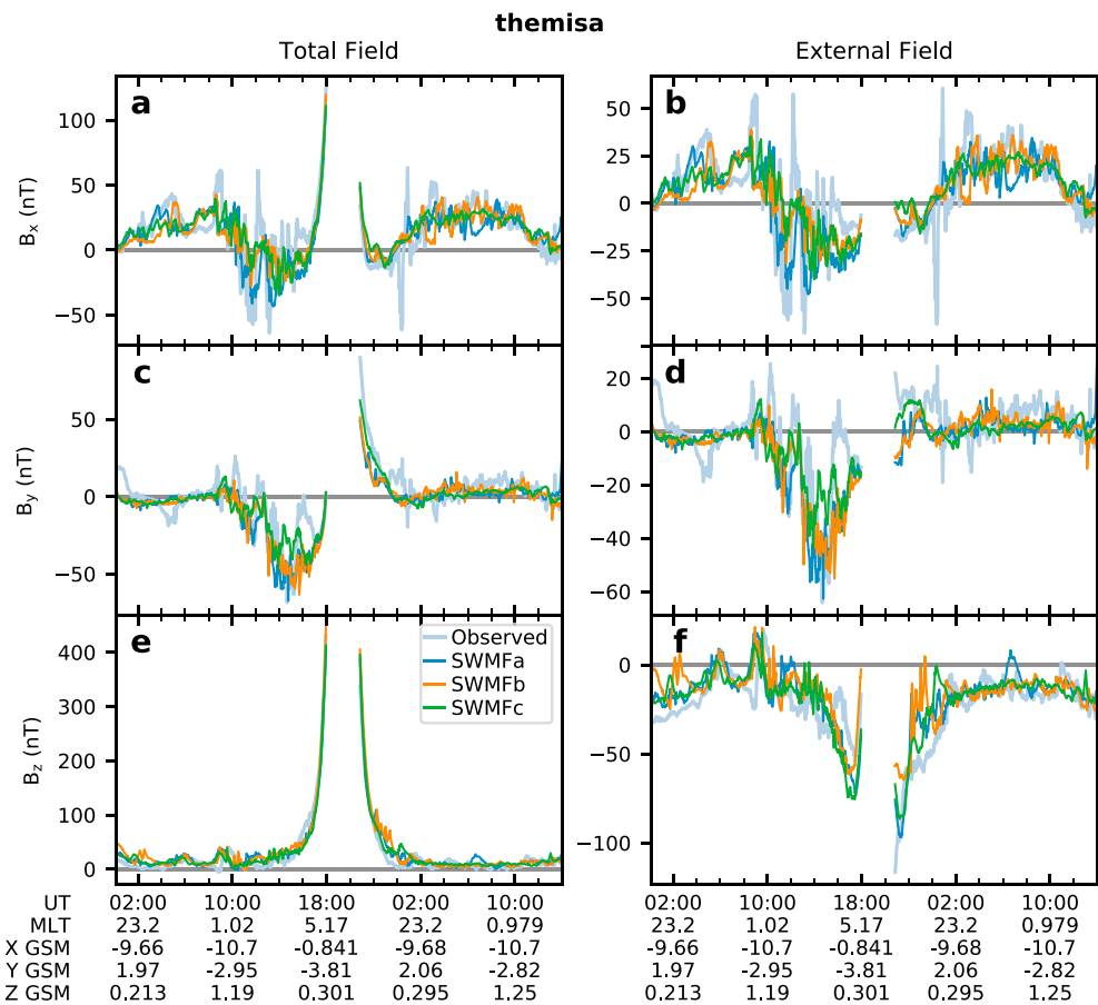
Figure 3. Magnetic field components of the total field in GSM coordinates at the THEMIS A satellite, observed and simulated, from 0009 UT on 5 April to 1400 UT on 6 April 2010. MLT = magnetic local time; GSM = geocentric solar magnetospheric; SWMF = Space Weather Modeling Framework.
