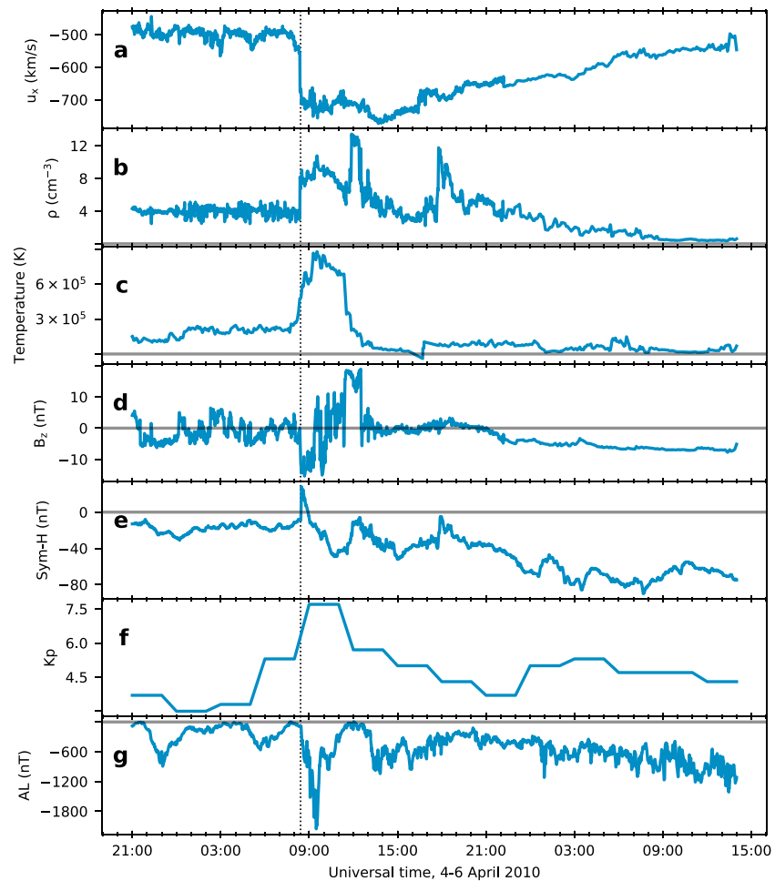
Figure 1. Solar wind driving parameters used in the study, along with geomagnetic indices parameterizing the magnetospheric response. (a) u_x component of bulk velocity, in geocentric solar magnetospheric coordinates, (b) proton density \rho , (c) temperature, (d) interplanetary magnetic field B_z , (e) Sym-H , and (f) Kp , (g) AL . The beginning of the storm is marked with a vertical line.
