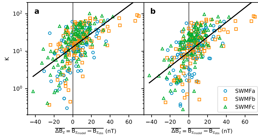
Figure 5. K as a function of \overline{\Delta B_z} for all three magnetohydrodynamic simulations, computed for locations mapped from isotropic boundary observations in the high-latitude data set (a) and the low-latitude data set (b). Black lines show linear fits (in log space) to the data.
