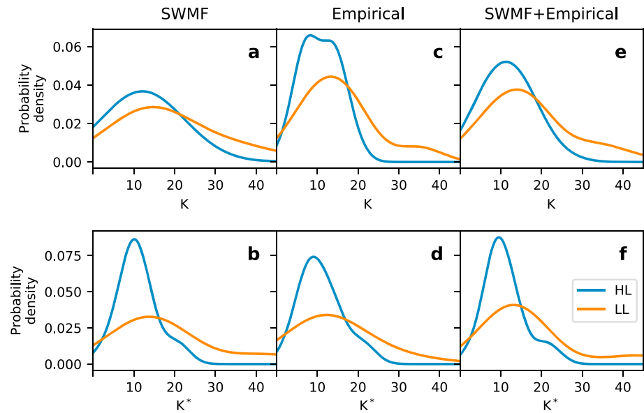
Figure 7. Distributions of (a) K and (b) K^* for all three magnetohydrodynamic simulations, and distributions of (c) K and (d) K^* for all empirical models. (e and f) Space Weather Modeling Framework (SWMF) and empirical models together. The distributions have been separated according to whether the observations came from the high-latitude (HL) or the low-latitude (LL) edge of the isotropic boundary.
