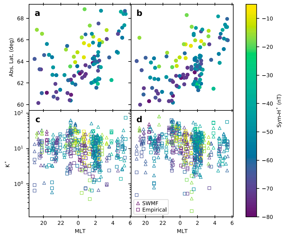
Figure 8. (a) HL IB latitude as a function of MLT, (b) LL IB latitude as a function of MLT, (c) HL K^* as a function of MLT, (d) LL K^* as a function of MLT. All points are colored by Sym-H^* . Shapes in (c) and (d) denote the class of model (SWMF or empirical). SWMF = Space Weather Modeling Framework; HL = high-latitude; LL = low-latitude; IB = isotropic boundary; MLT = magnetic local time.
