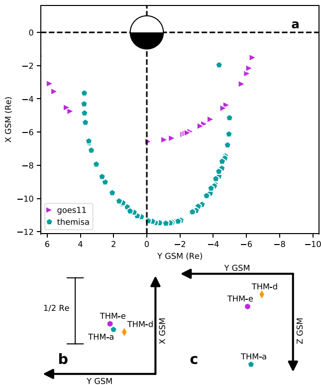
Figure 2. (a) Locations of THEMIS A and GOES 11 at the times of all the isotropic boundary observations. (b and c) Relative positions of THEMIS A, THEMIS D, and THEMIS E at 0700 UT on 5 April.
