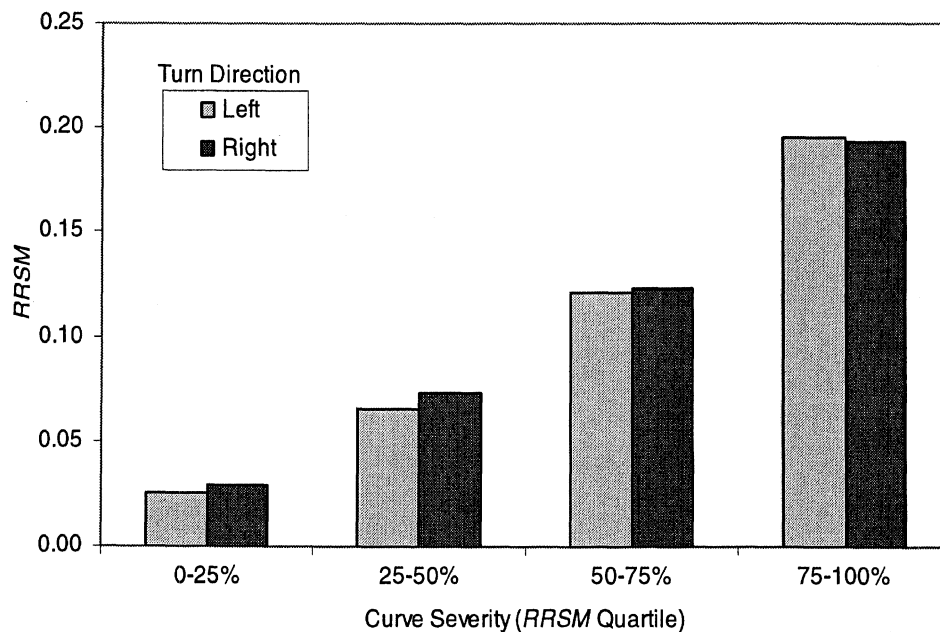
Figure 8-26. The interaction between turn direction and curve severity
