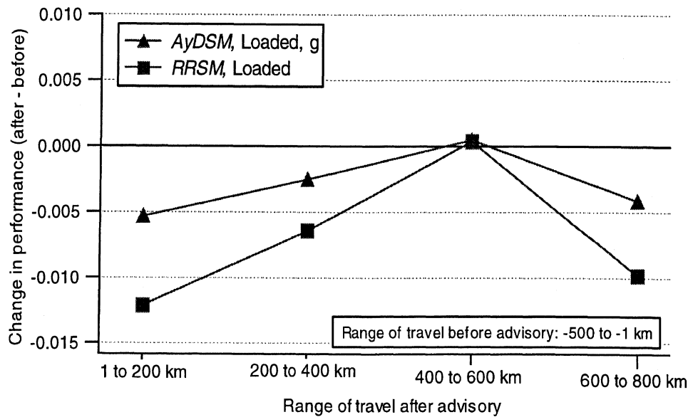
Figure 8-55. Significant changes in performance by interval after advisory
