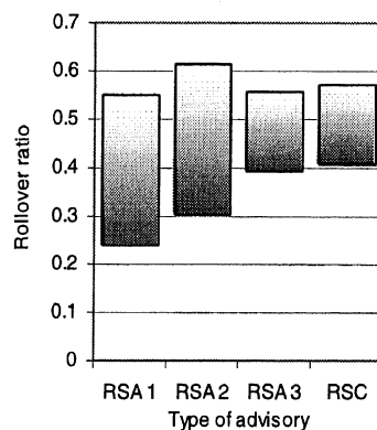
Ranges of peak lateral acceleration and rollover ratio associated with RSA/C advisories in the field test
