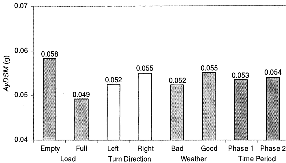
Figure 8-32. Main effects of load, turn direction, weather, and phase on AyDSM
