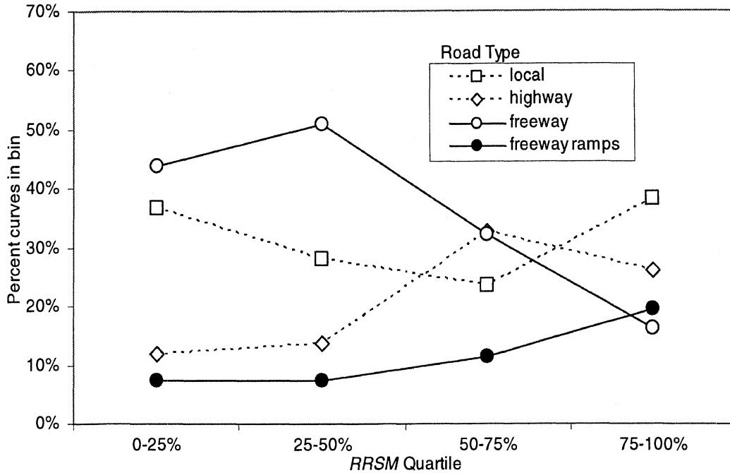
Figure 8-18. Distribution of curve types among the RRSM quartiles
