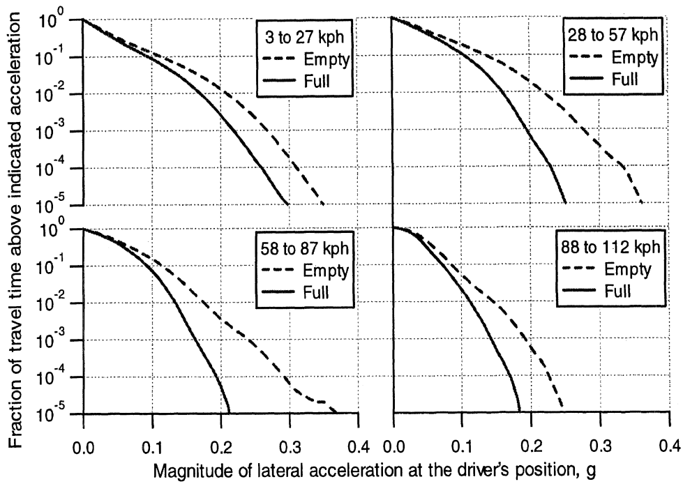
Figure 6-12. Cumulative histograms of travel time in curves for lateral acceleration by speed and load
