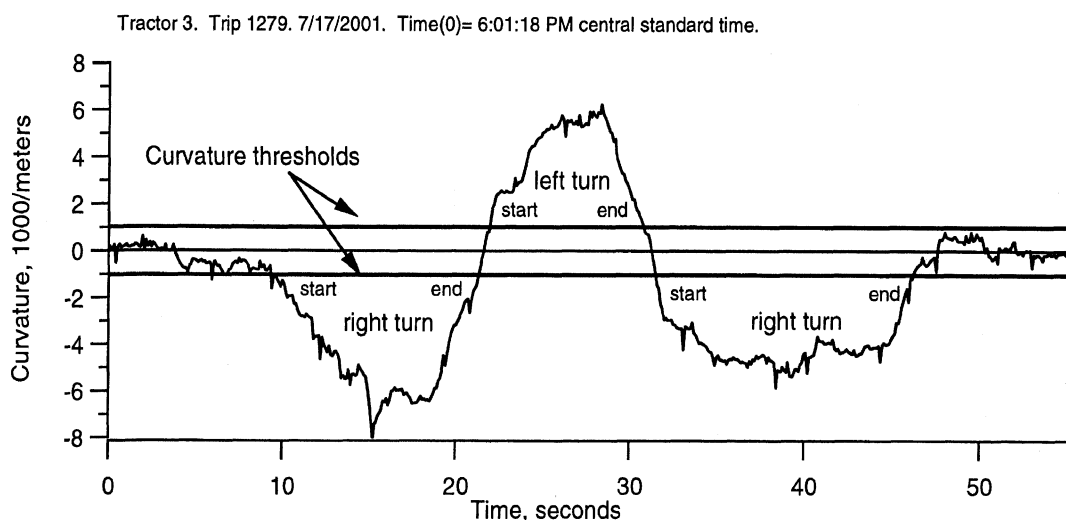
Figure 4-10. Curvature thresholds to define a turn
