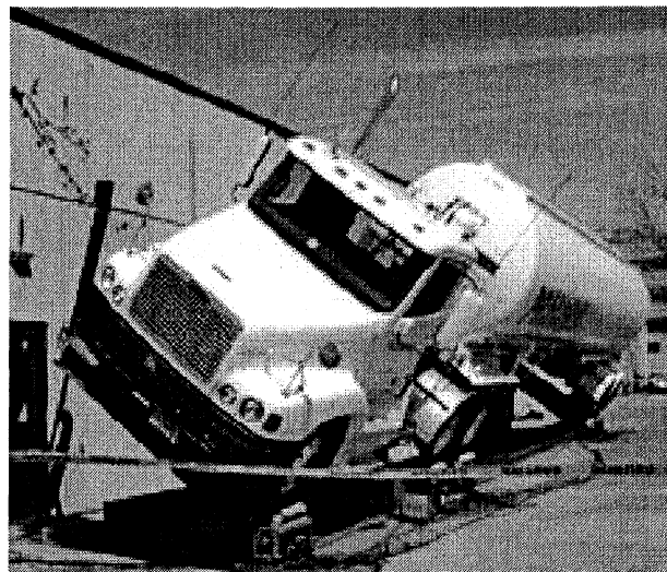
Figure A-C1. RA&C test vehicle on the UMTRI tilt table
