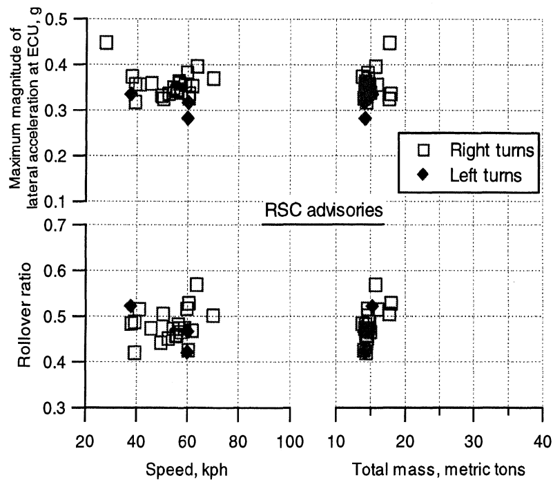
Figure 7-12. Maximum lateral acceleration at the ECU and maximum rollover ratio by speed and load for RSC episodes
