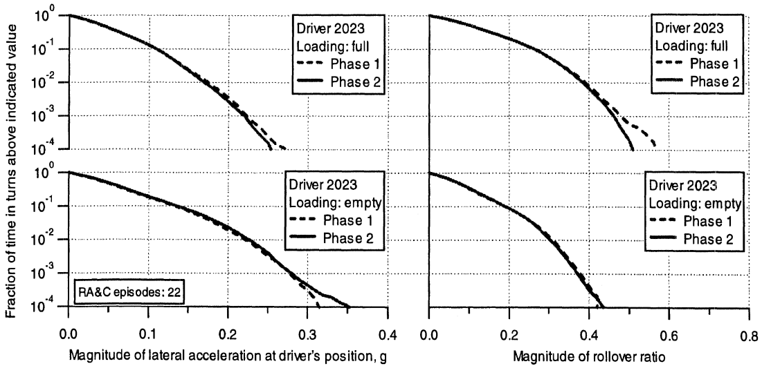
Figure 8-4. Comparison of phase-1 and phase-2 lateral performance in turns of driver 2023
