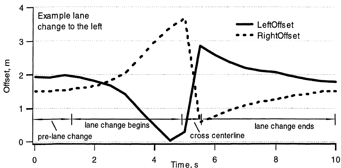
Figure A-E8. An example of the left- and right-offset values characteristic of a lane change
