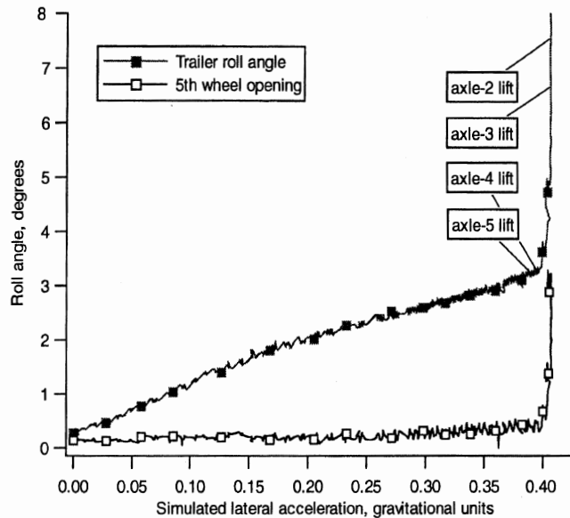
Figure A-C2. Example data from tilt-table test; ¼ load.
