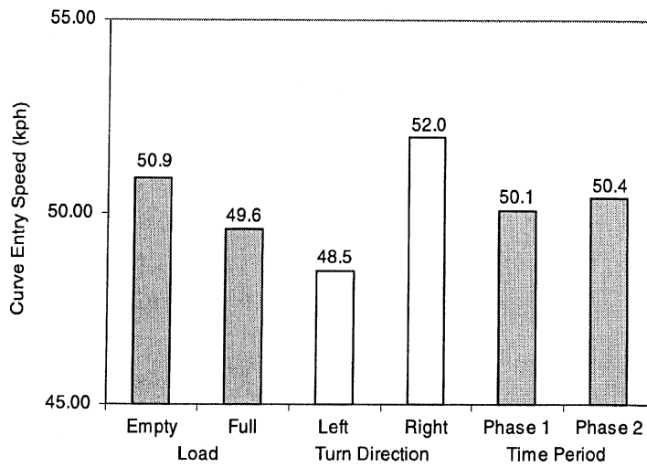
Figure 8-41. The main effects of load, turn and phase on curve-entry speed
