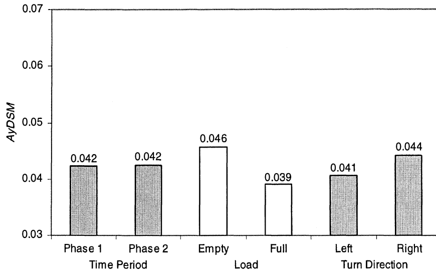
Figure 8-47. Main effects of phase, load and turn direction on AyDSM
