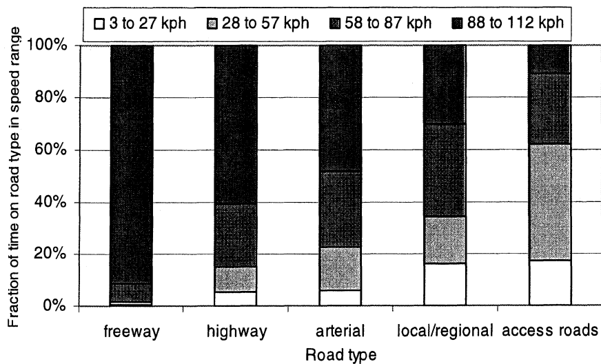
Figure 5-5. Distribution of travel time by speed for each road classification
