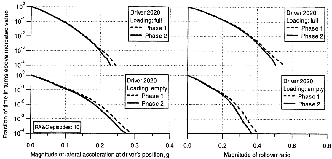
Figure 8-1. Comparison of phase-1 and phase-2 lateral performance in turns of driver 2020
