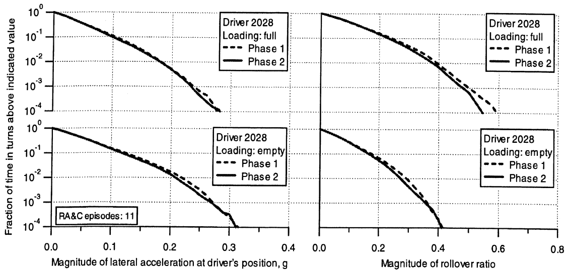
Figure 8-7. Comparison of phase-1 and phase-2 lateral performance in turns of driver 2028
