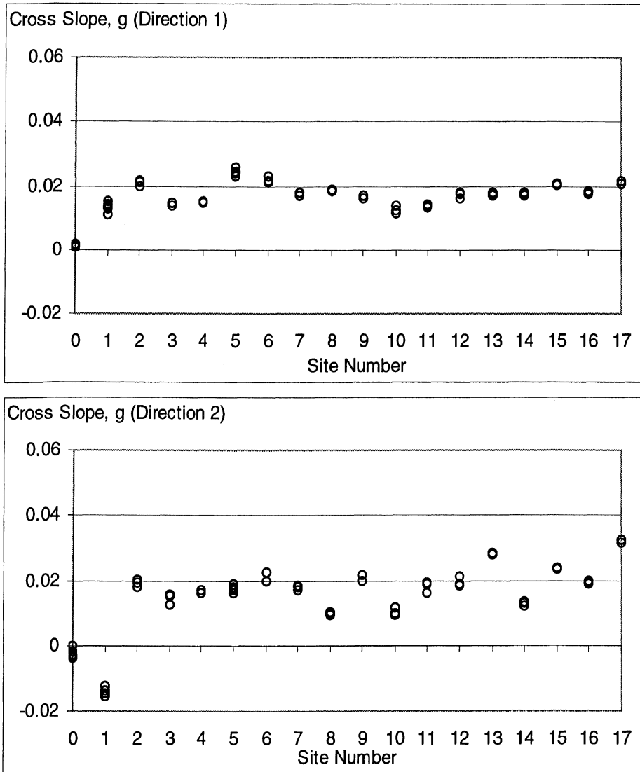
Figure A-E6. Cross slope for each site in direction 1 and 2, respectively
