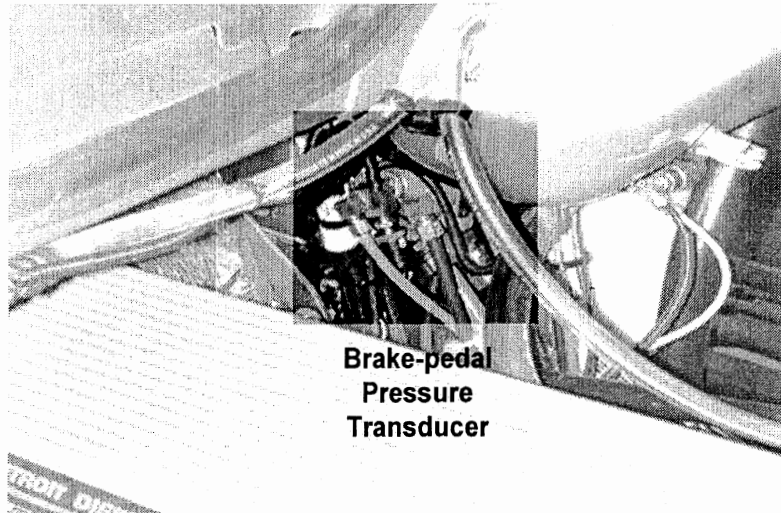
Figure 3-5. Location of brake-pedal pressure transducer
