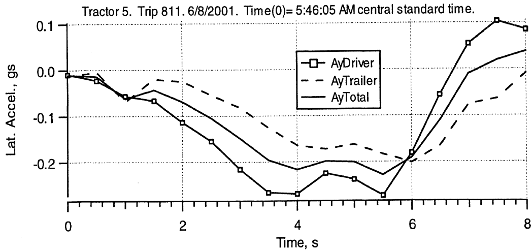
Figure 4-6. Ay_{Total} as a function of time
