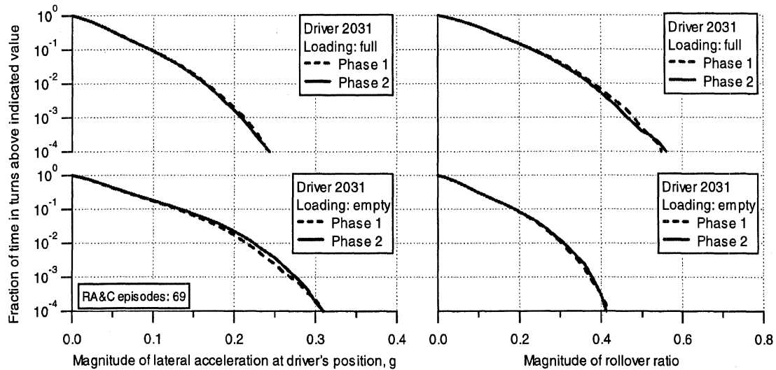
Figure 8-10. Comparison of phase-1 and phase-2 lateral performance in turns of driver 2031
