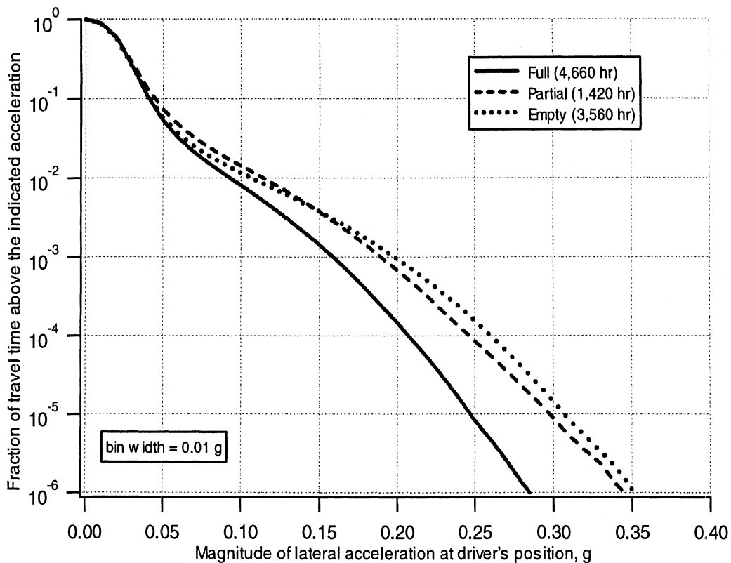
Figure 6-2. Cumulative histogram of travel time by magnitude of lateral acceleration for three load ranges
