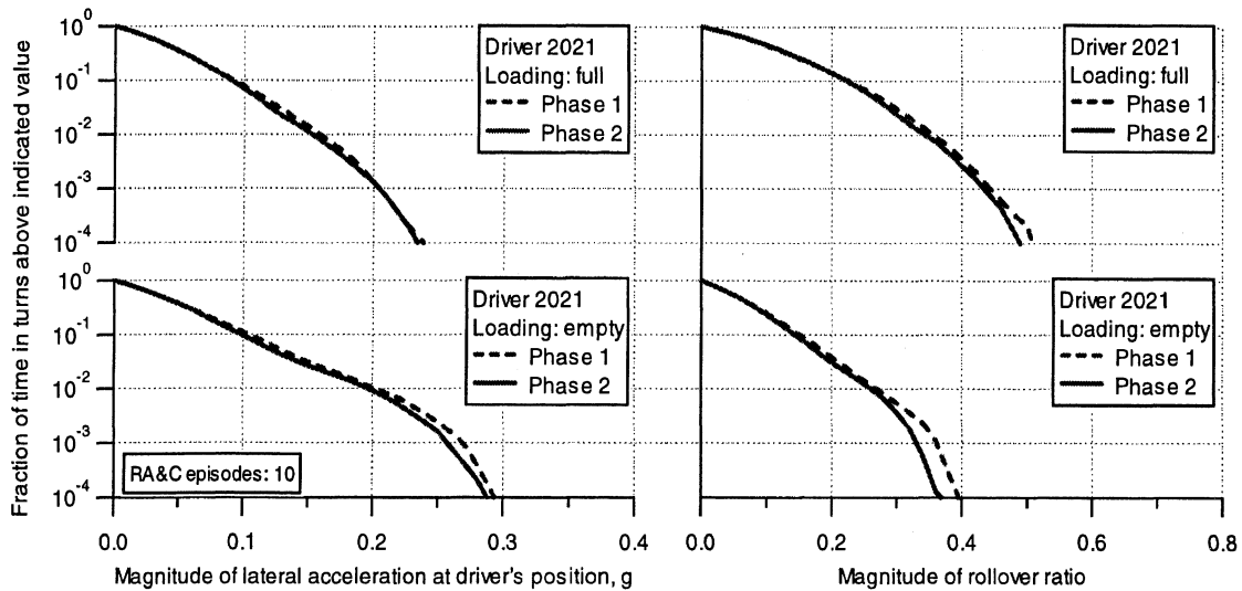
Figure 8-2. Comparison of phase-1 and phase-2 lateral performance in turns of driver 2021
