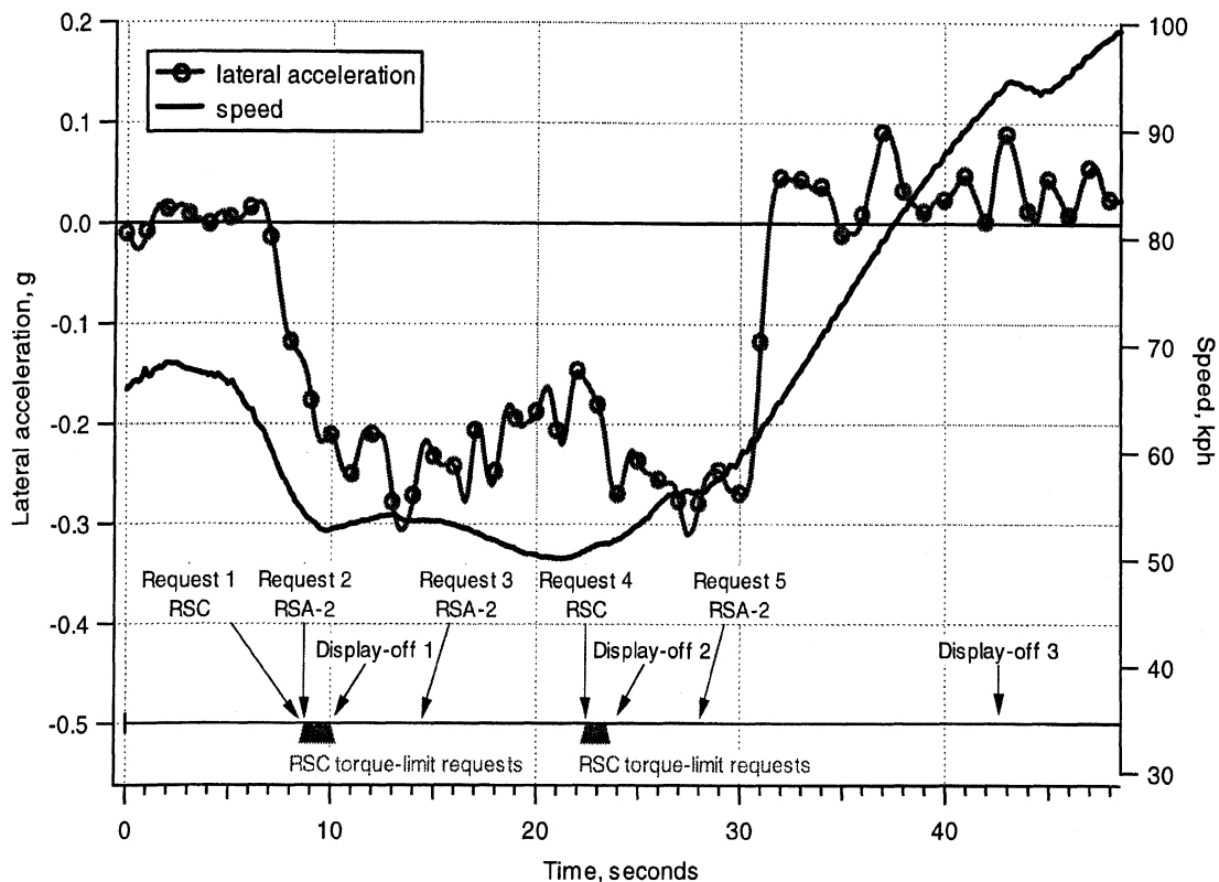
Figure 7-4. Time history of a complex RSA/C episode with five advisory requests
