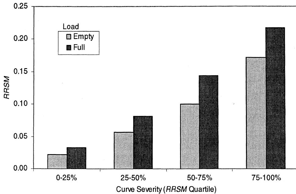
Figure 8-25. The interaction between load and curve severity
