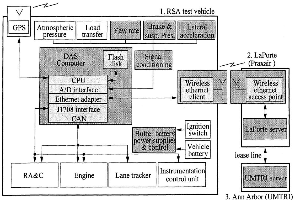
Figure 3-11. The DAS system including vehicle, La Porte, and Ann Arbor components
