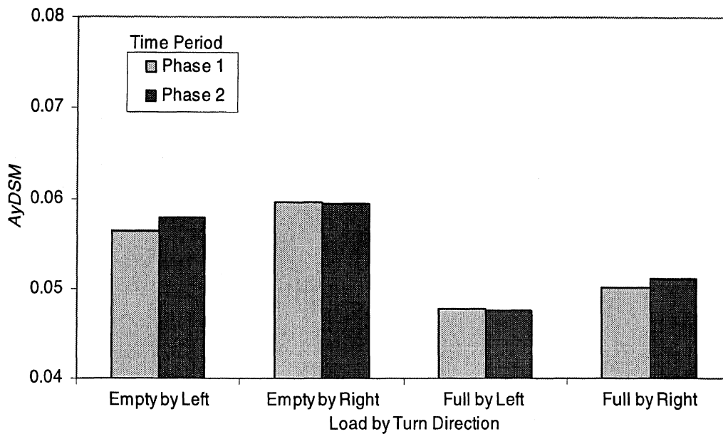
Figure 8-37. Three way interaction between load, phase and turn direction
