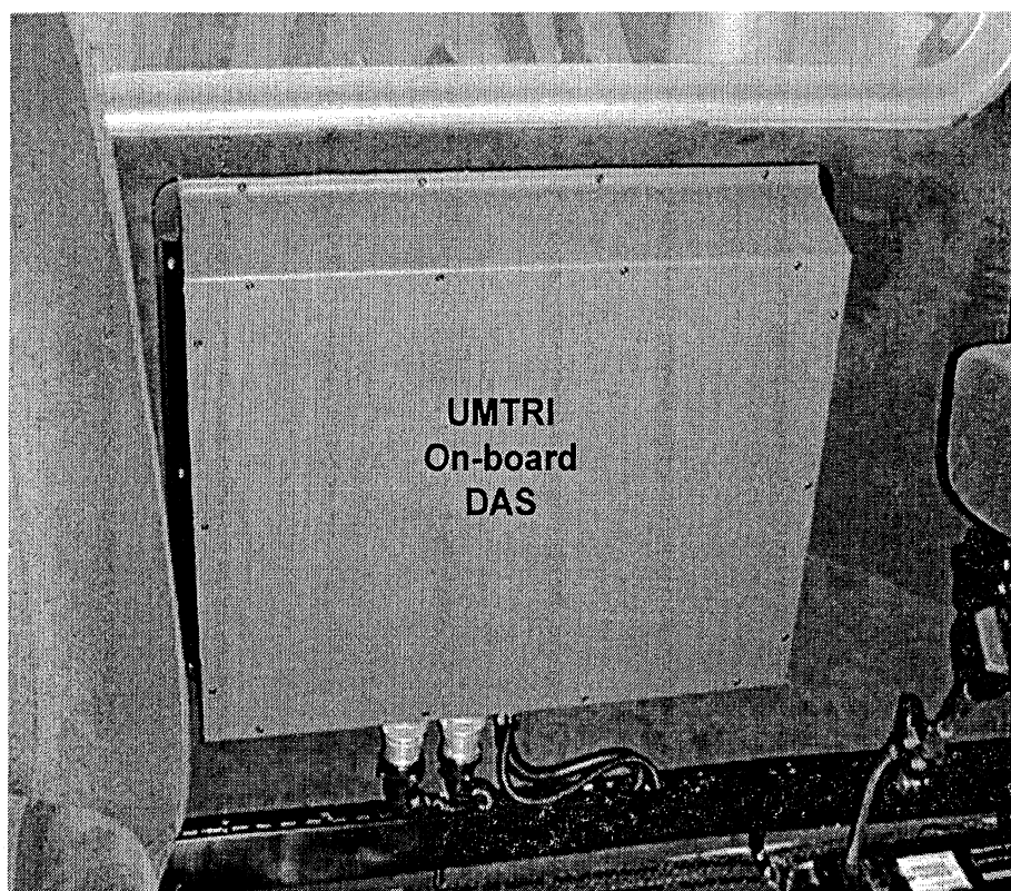
Figure 3-12. Installed UMTRI on-board data acquisition system
