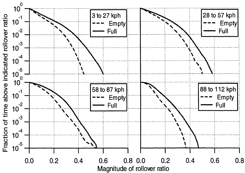
Figure 6-13. Cumulative histograms of travel time in curves for rollover ratio by speed and load
