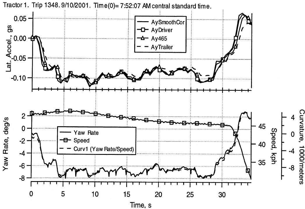
Figure 4-8. Time-history plot of a 180 degree right-hand turn
