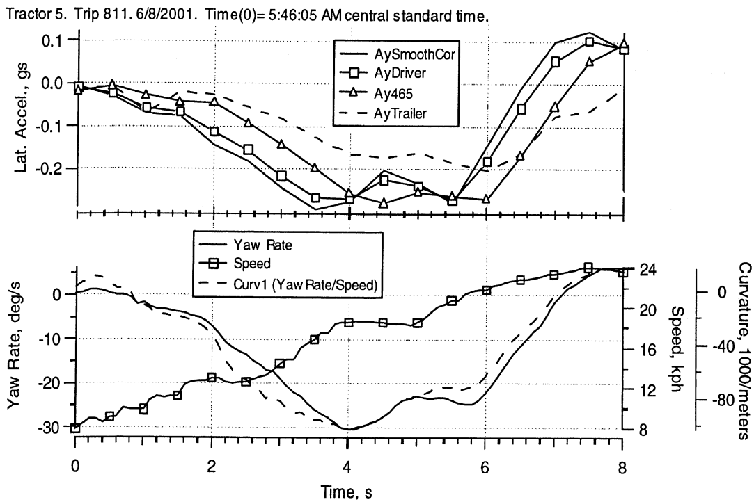
Figure 4-5. Time-history plot of a 90 degree right-hand turn
