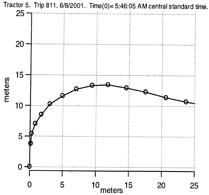
Figure 4-4. Path of the tractor in a 90 degree small radius turn
