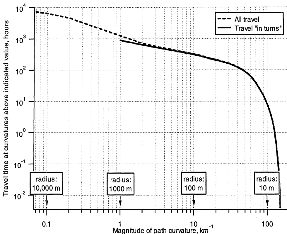
Figure 5-9. Cumulative histograms of path curvature
