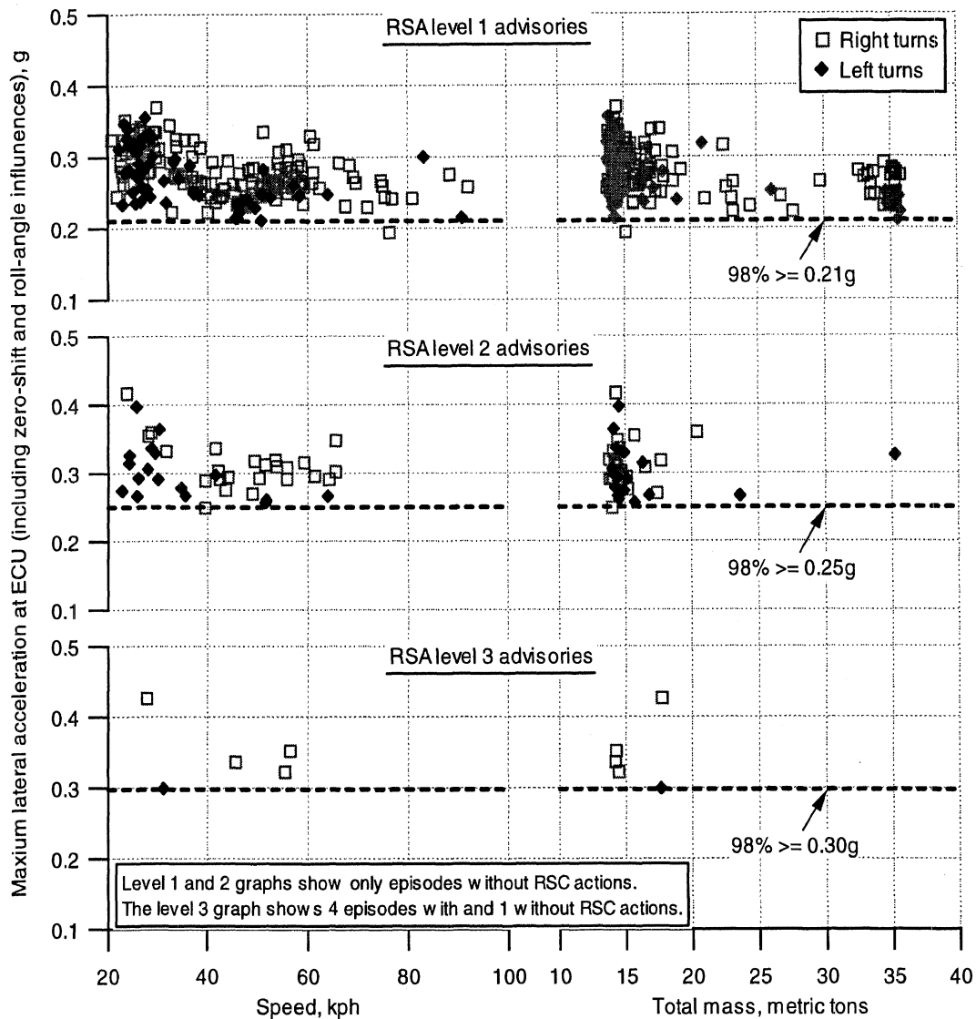
Figure 7-9. Maximum lateral acceleration at the ECU by speed and load for RSA episodes
