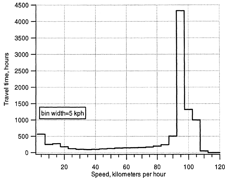
Figure 5-6. Histogram of travel time by speed
