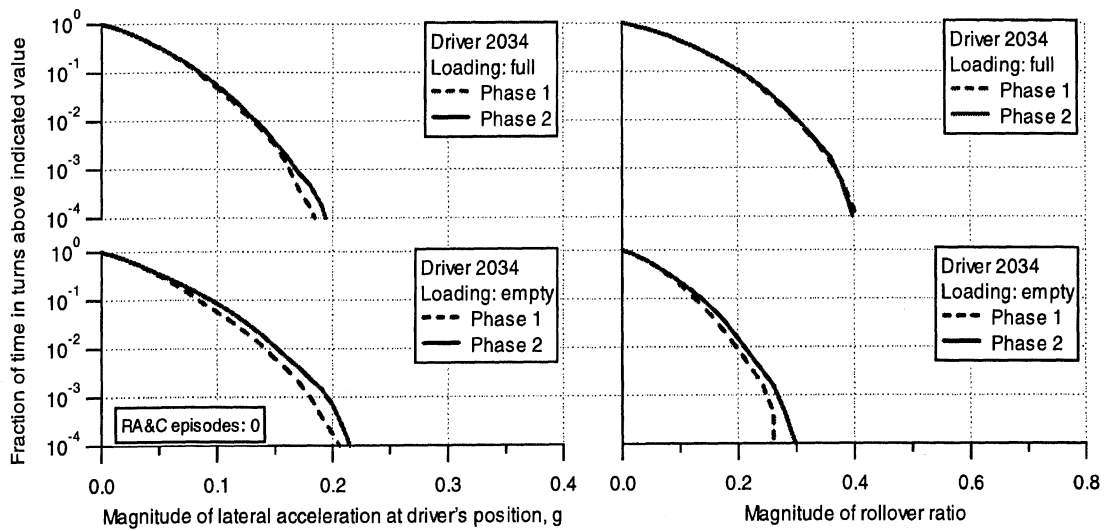
Figure 8-13. Comparison of phase-1 and phase-2 lateral performance in turns of driver 2034
