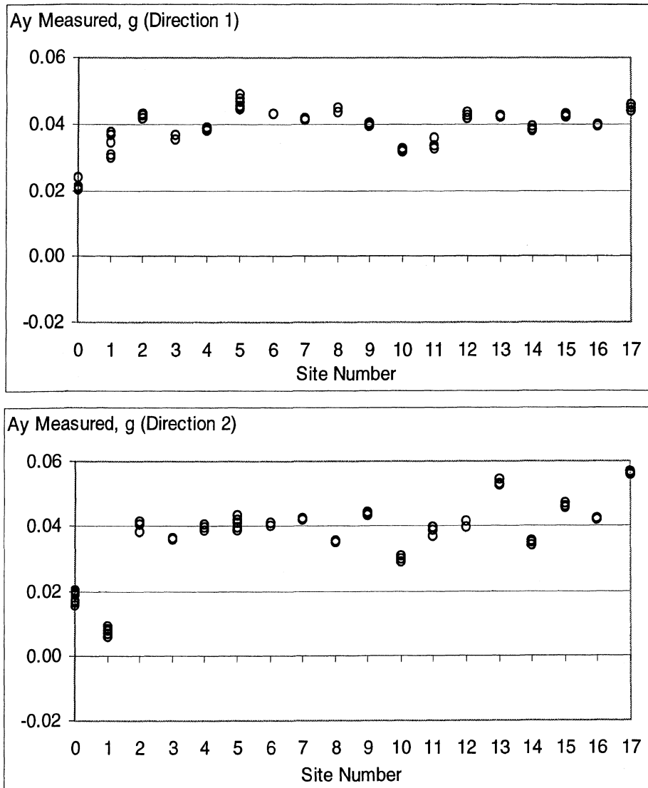
Figure A-E5. Direction 1 and direction 2 measured-lateral acceleration for each site
