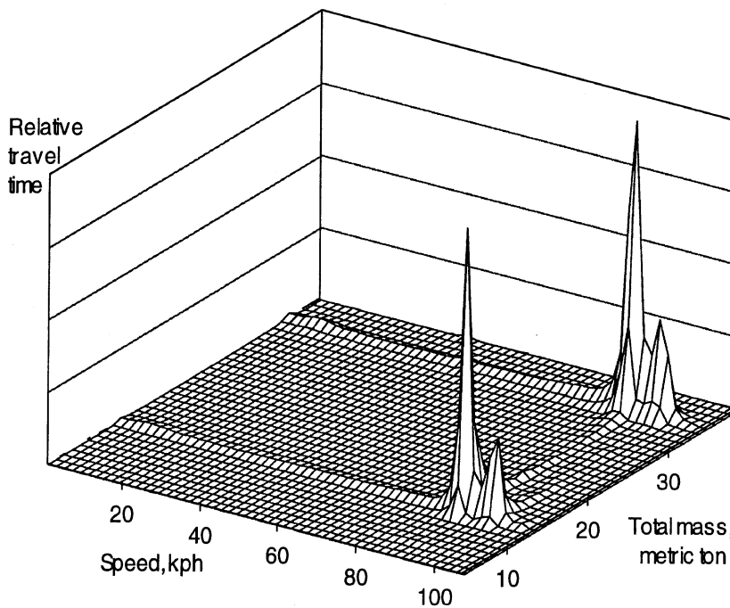
Figure 5-8. A two-dimensional histogram of travel time by mass and speed
