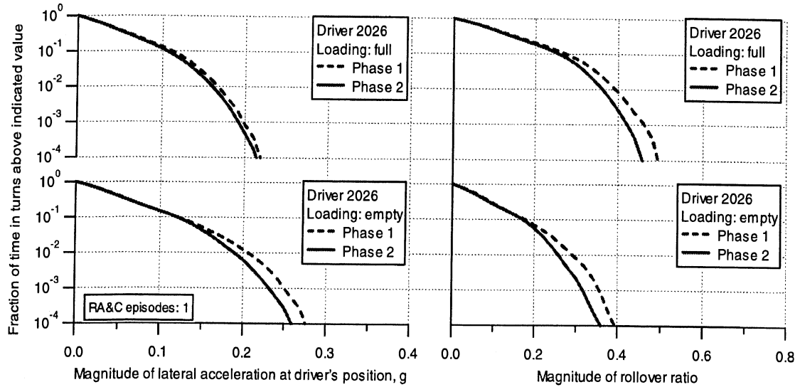
Figure 8-6. Comparison of phase-1 and phase-2 lateral performance in turns of driver 2026
