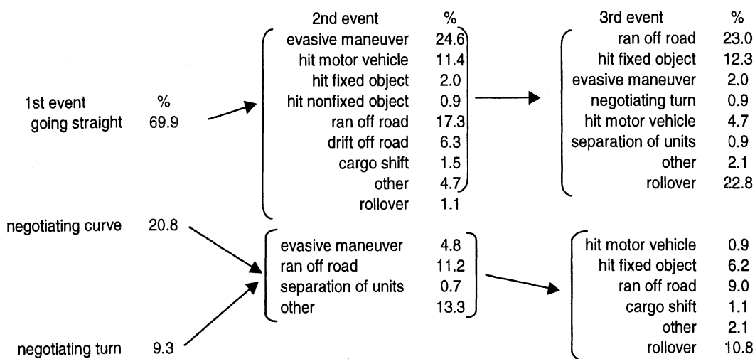
Figure A-A6 Event tree for rollovers not addressable by RSA
