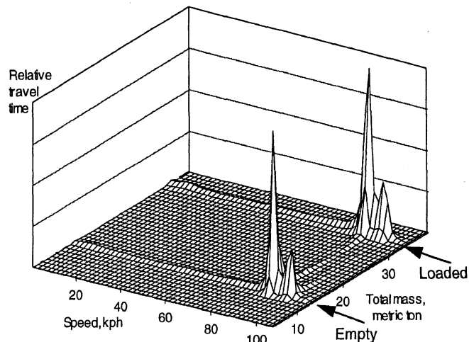
Two-dimensional histogram of fleet travel by mass and speed
