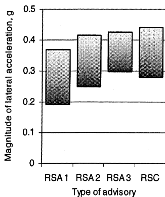
Ranges of peak lateral acceleration and rollover ratio associated with RSA/C advisories in the field test
