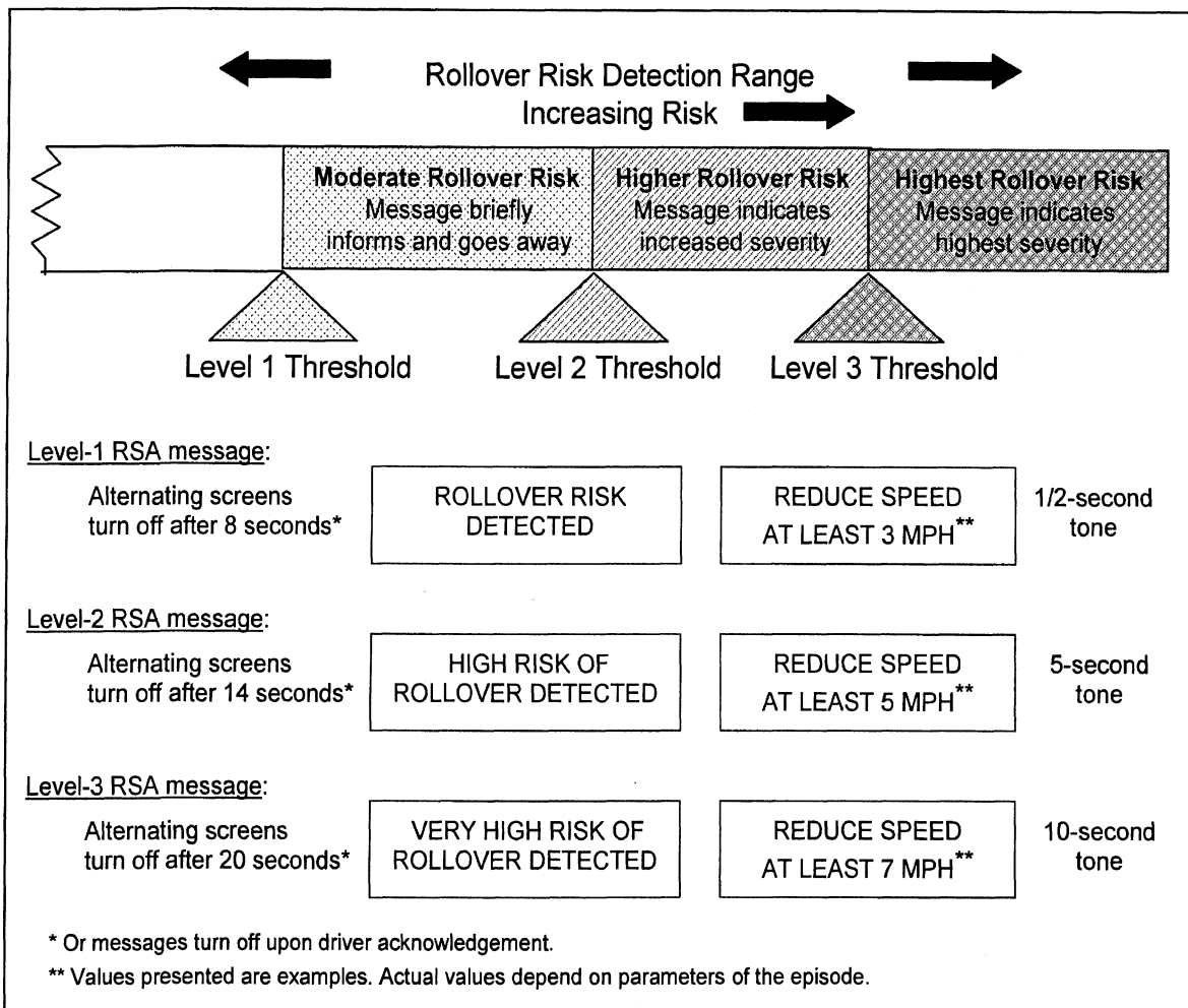
Figure 2-3. RSA concept and advisory messages.
