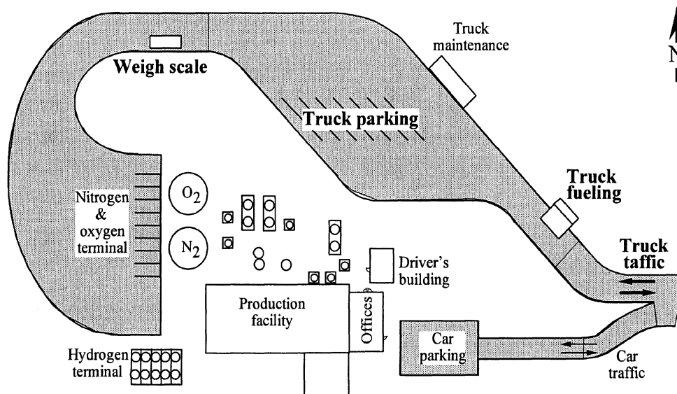
Figure 3-1. Praxair's La Porte, Indiana production and distribution facility
