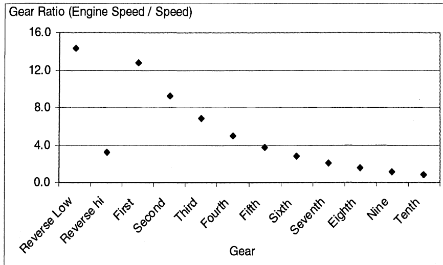
Figure 4-1. Gear versus gear ratio
