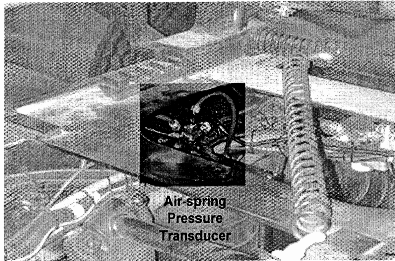
Figure 3-4. Location of air-spring pressure transducer
