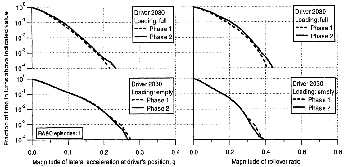
Figure 8-9. Comparison of phase-1 and phase-2 lateral performance in turns of driver 2030
