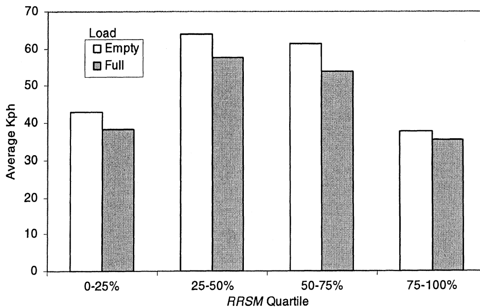
Figure 8-17. Average speed within each curve-severity quartile (by RRS) for full and empty trailers
