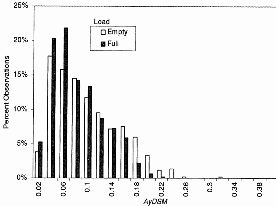
Figure 8-19. Normalized distributions of AyDSM observed on curves among non-comparable drivers
