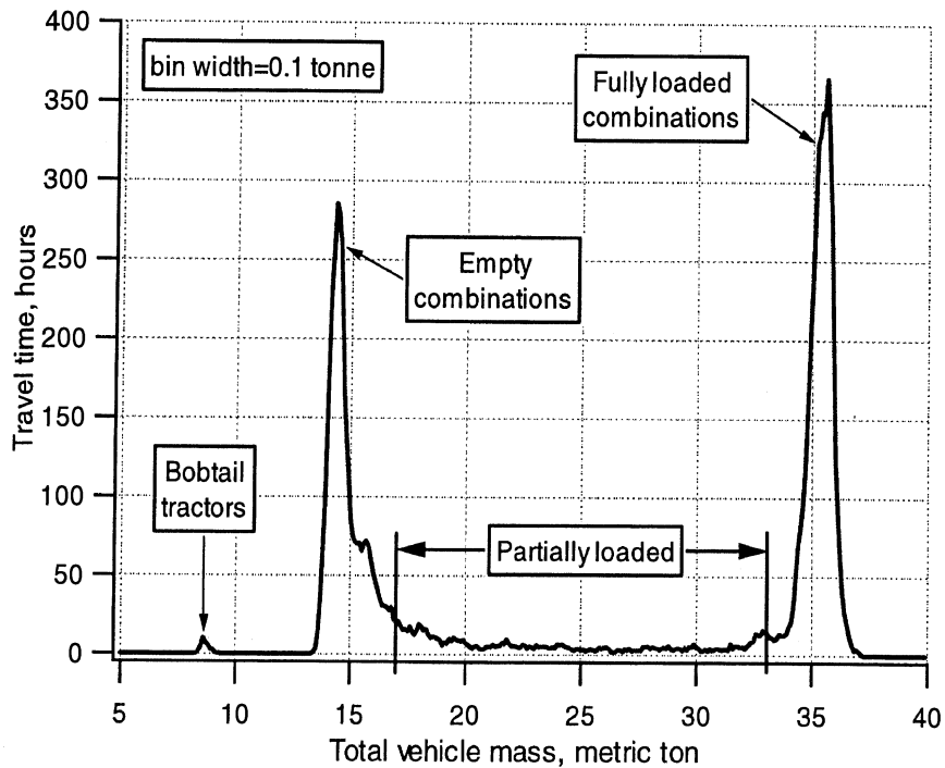
Figure 5-7. Histogram of travel time by total vehicle mass
