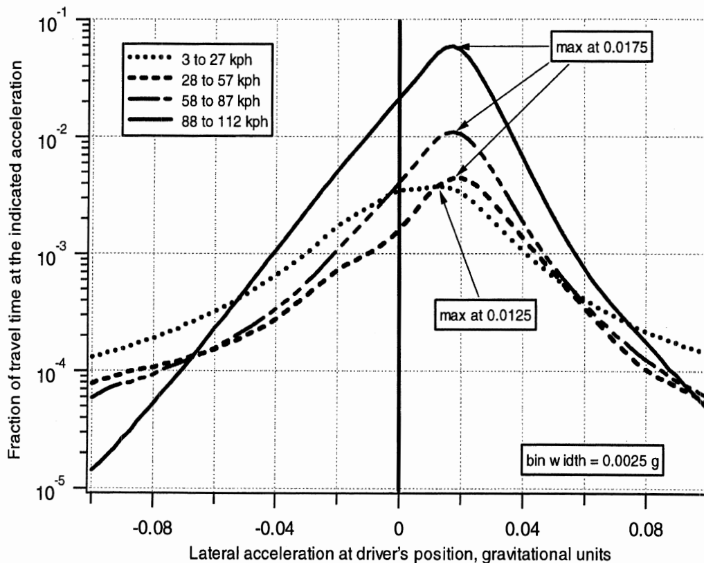
Figure 6-5. Histogram of travel time at small lateral accelerations for four speed ranges
