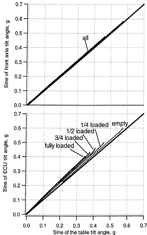
Figure A-C4. Sin(component tilt angle) versus sin(table tilt angle); five loading conditions
