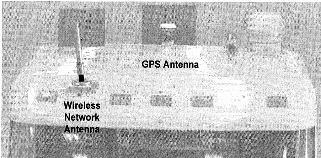
Figure 3-7. Location of wireless network and GPS antennas
