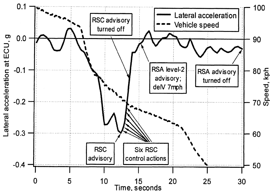
Figure 2-8. Time histories from an episode involving RSC and RSA advisories
