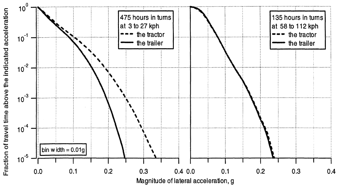
Figure 6-8. Cumulative histogram of travel time in curves by magnitude of lateral acceleration of the tractor ( AyDriver ) and the trailer ( AyTrailer ) for low and high speed ranges
