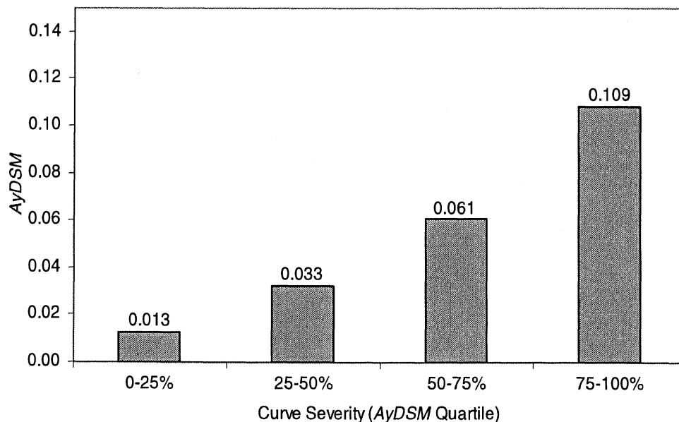
Figure 8-33. Main effect of curve severity indexed by AyDSM quartile
