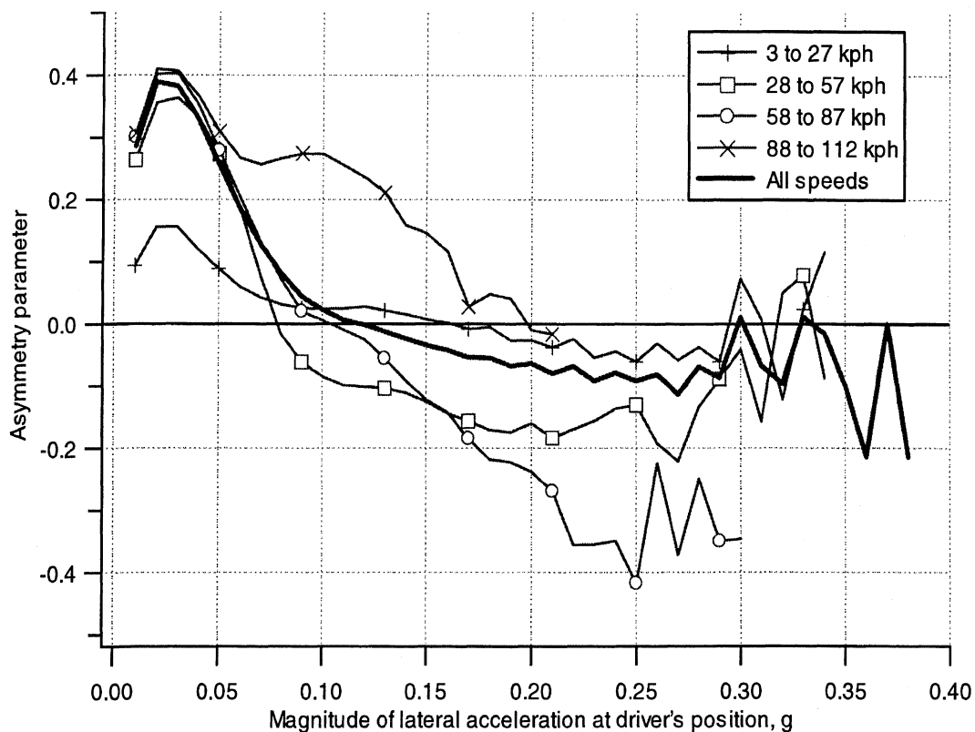
Figure 6-6. The asymmetry parameter for travel time as a function of lateral accelerations for four speed ranges and all speeds
