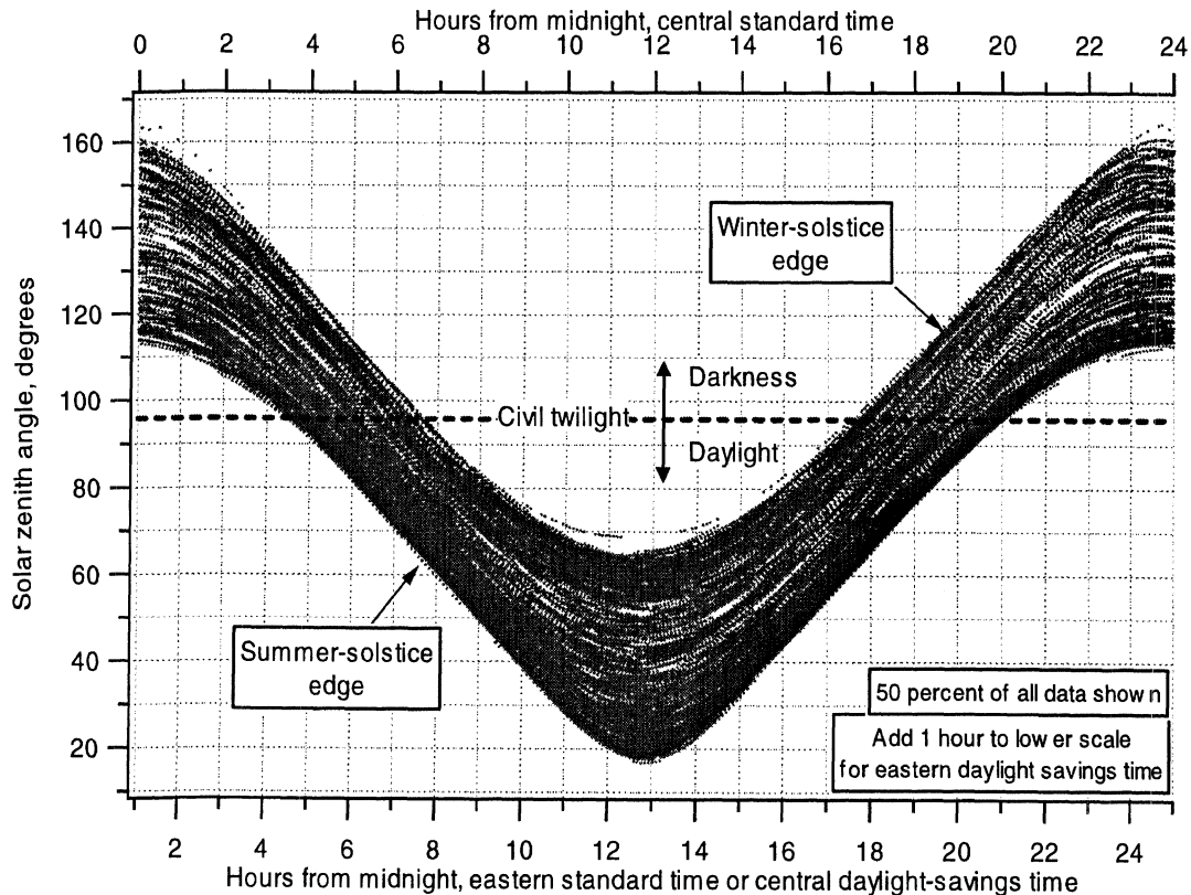
Figure A-D1. Solar zenith angle
