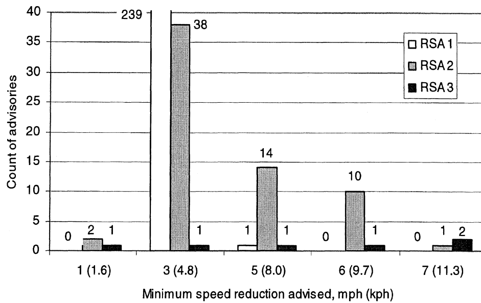
Figure 7-7. Counts of speed-change advisories by speed and RSA advisory level
