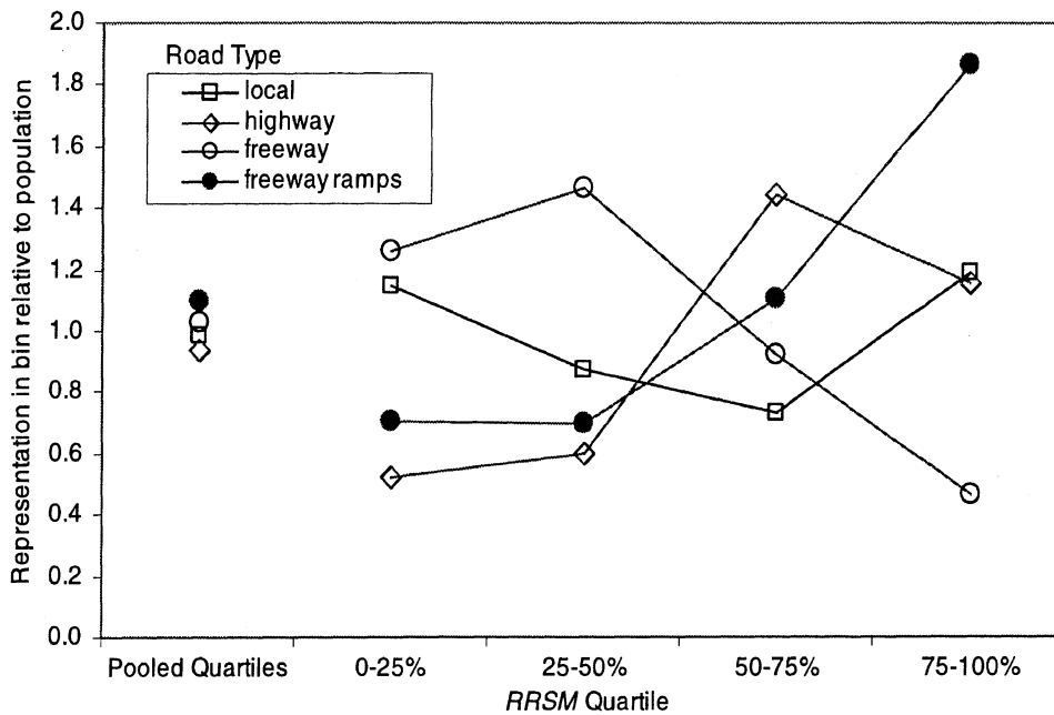
Figure 8-16. Relationship of sampled curves to the population of curves
