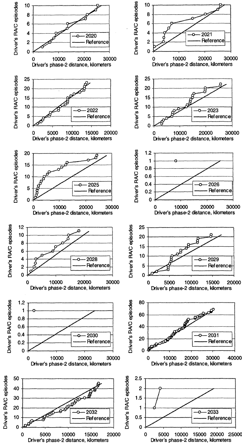
Figure 7-18. The accumulation of RSA/C episodes by individual drivers
