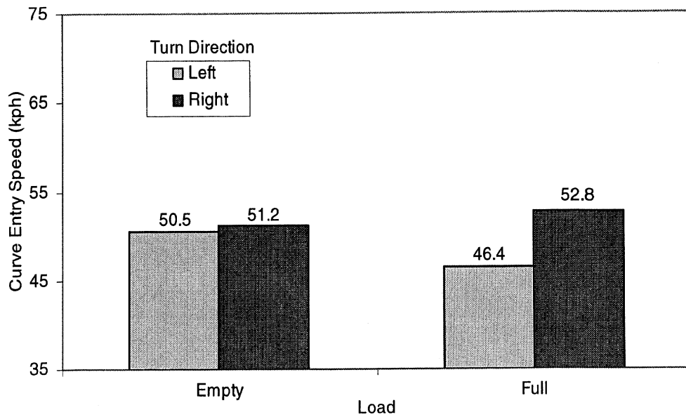
Figure 8-43. Interaction between turn direction and trailer load
