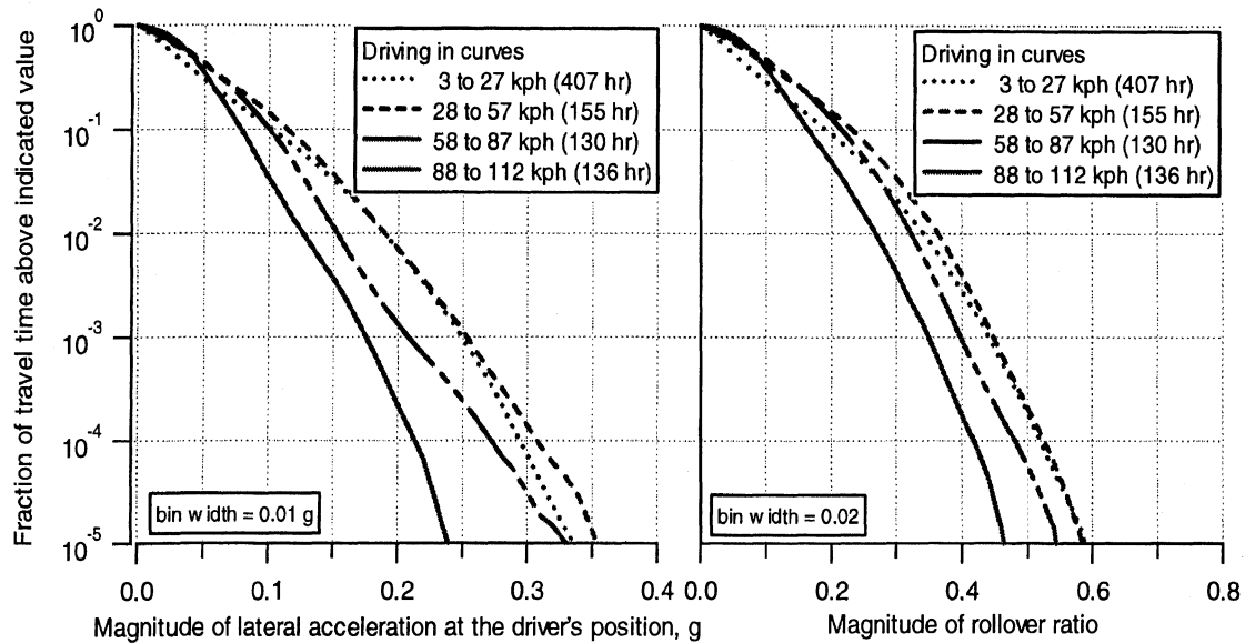
Figure 6-11. Cumulative histograms of travel time in curves for lateral acceleration and rollover ratio by speed range
