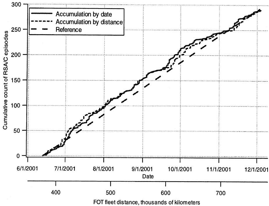
Figure 7-17. The accumulation of RSA/C episodes during phase 2
