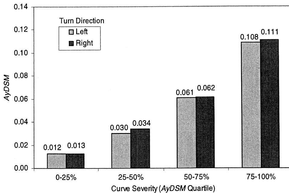
Figure 8-36. Interaction between turn direction and curve severity
