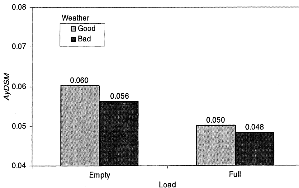
Figure 8-34. Interaction between vehicle load and weather
