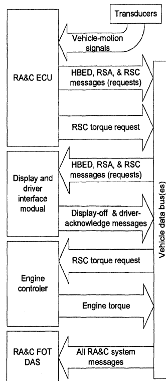
Figure 7-1. Simplified flow diagram of the messages of the RA&C system
