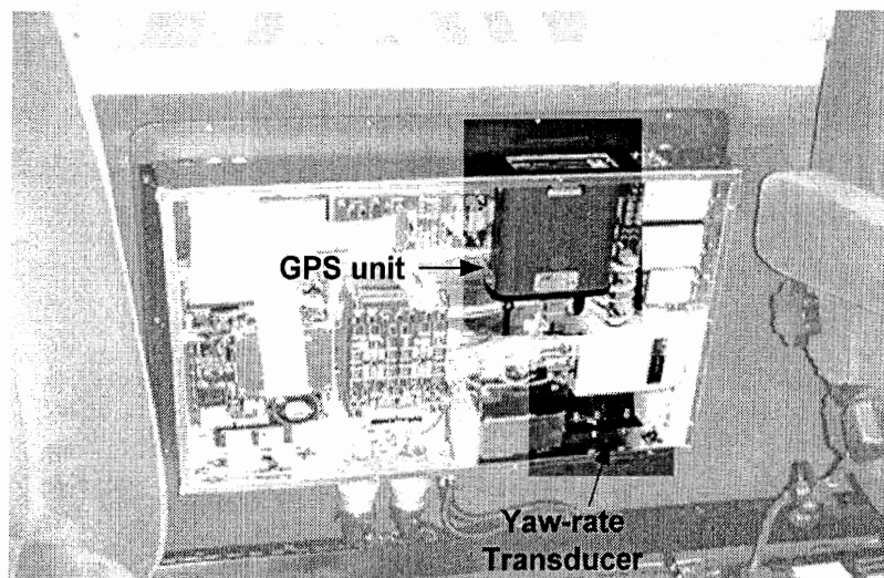
Figure 3-6. Location of GPS and yaw-rate transducer
