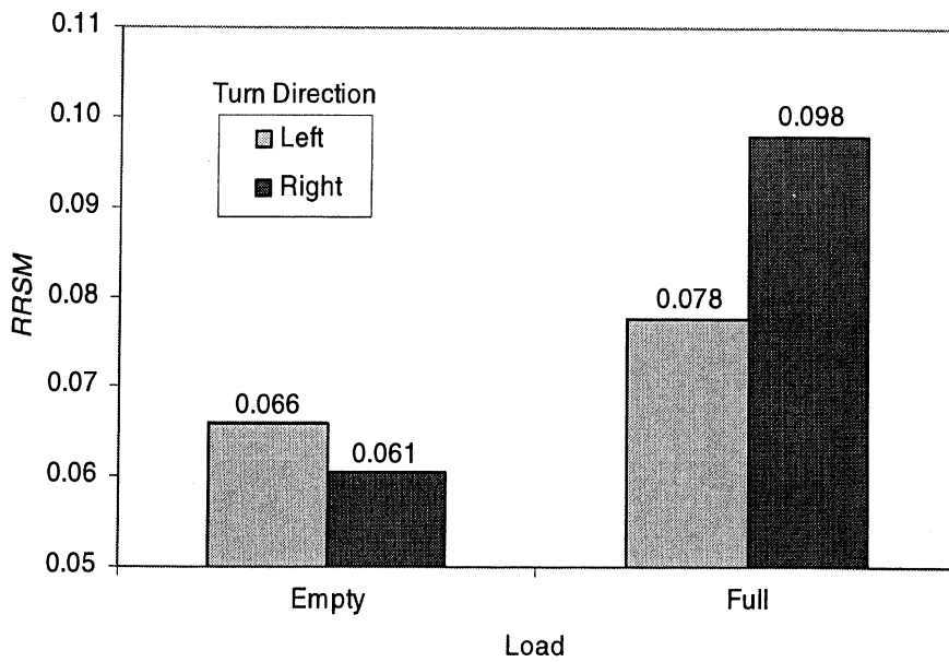
Figure 8-46. Two-way interaction for turn direction and load on RRSM
