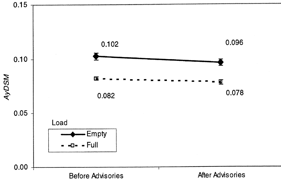
Figure 8-49. Main effects of exposure to advisory messages and load on AyDSM in the interval 250 km before and after an advisory
