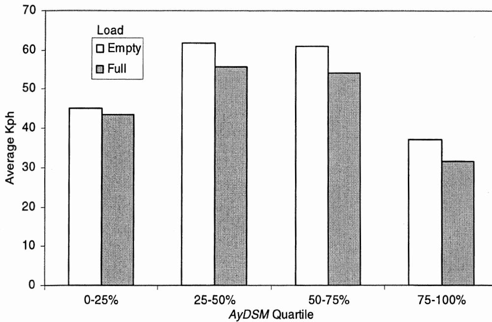
Figure 8-20. Average speed within each curve-severity quartile (by AyDSM) for full and empty trailers
