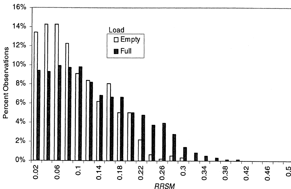
Figure 8-15. Normalized distributions of RRSM observed among non-comparable drivers on selected curves
