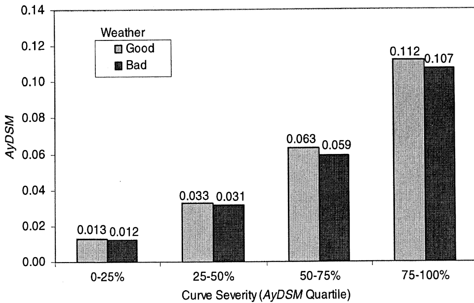
Figure 8-35. Interaction between weather and curve severity
