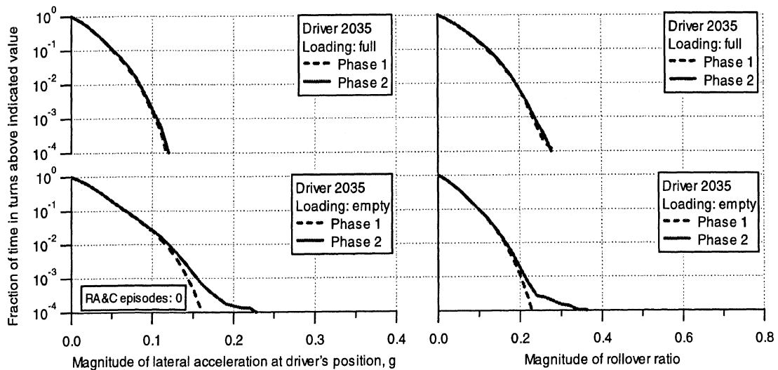
Figure 8-14. Comparison of phase-1 and phase-2 lateral performance in turns of driver 2035
