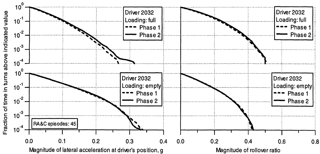
Figure 8-11. Comparison of phase-1 and phase-2 lateral performance in turns of driver 2032
