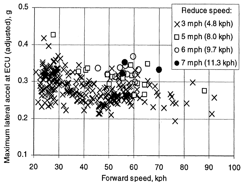
Figure 7-13. Speed-reduction advisories as a function of lateral acceleration and forward speed
