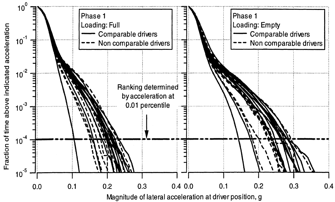
Figure 6-15. Cumulative histograms of travel time by magnitude of lateral acceleration comparing all drivers in phase 1
