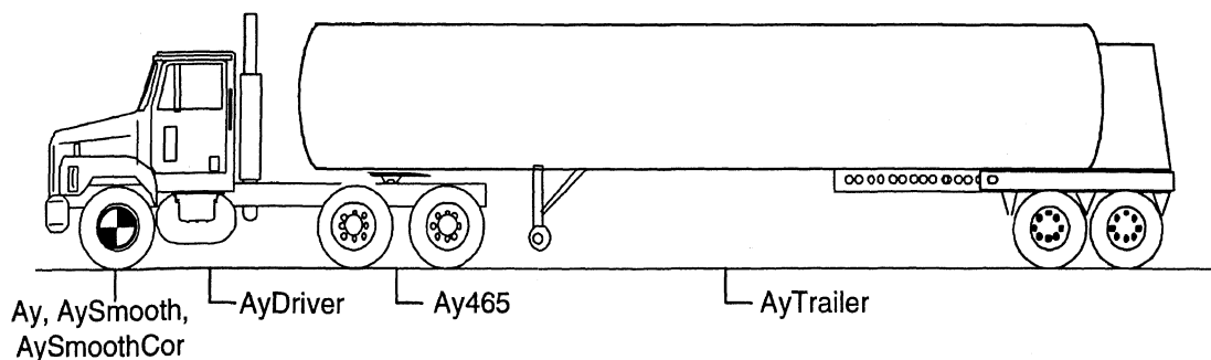
Figure 4-2. Locations of calculated lateral accelerations
