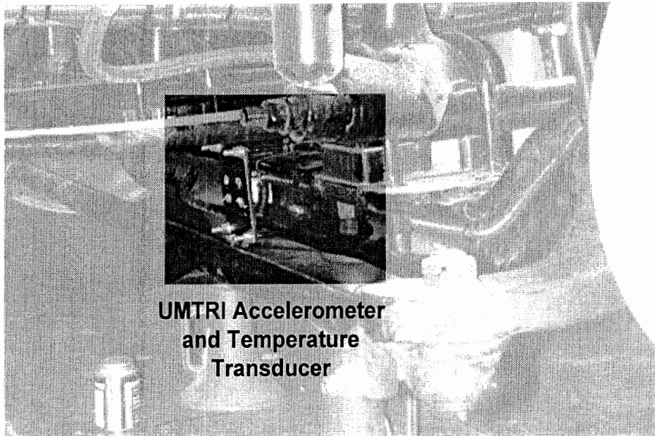
Figure 3-9. Location of the lateral acceleration and temperature transducer
