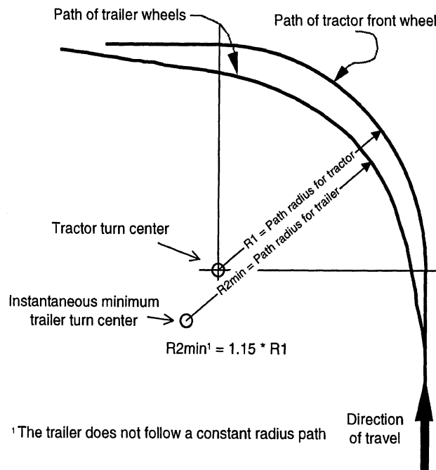
Figure 4-3. Example of low-speed off-tracking
