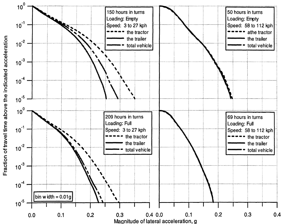
Figure 6-9. Cumulative histogram of travel time in curves by magnitude of lateral acceleration of the tractor ( A_{yDriver} ), the trailer ( A_{yTrailer} ), and for the total vehicle ( A_{yTotal} ) at two loads and at high and low speeds
