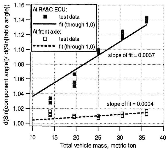
Figure A-C5. d(\sin(\text{component tilt angle}) / d(\sin(\text{table tilt angle})) for the front axle and the ECU as a function of total mass
