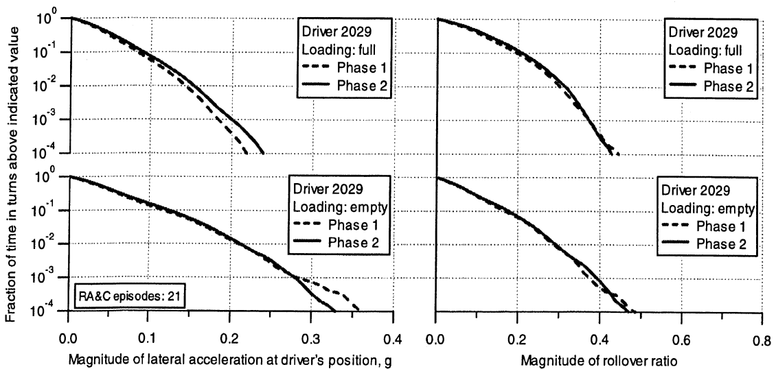
Figure 8-8. Comparison of phase-1 and phase-2 lateral performance in turns of driver 2029
