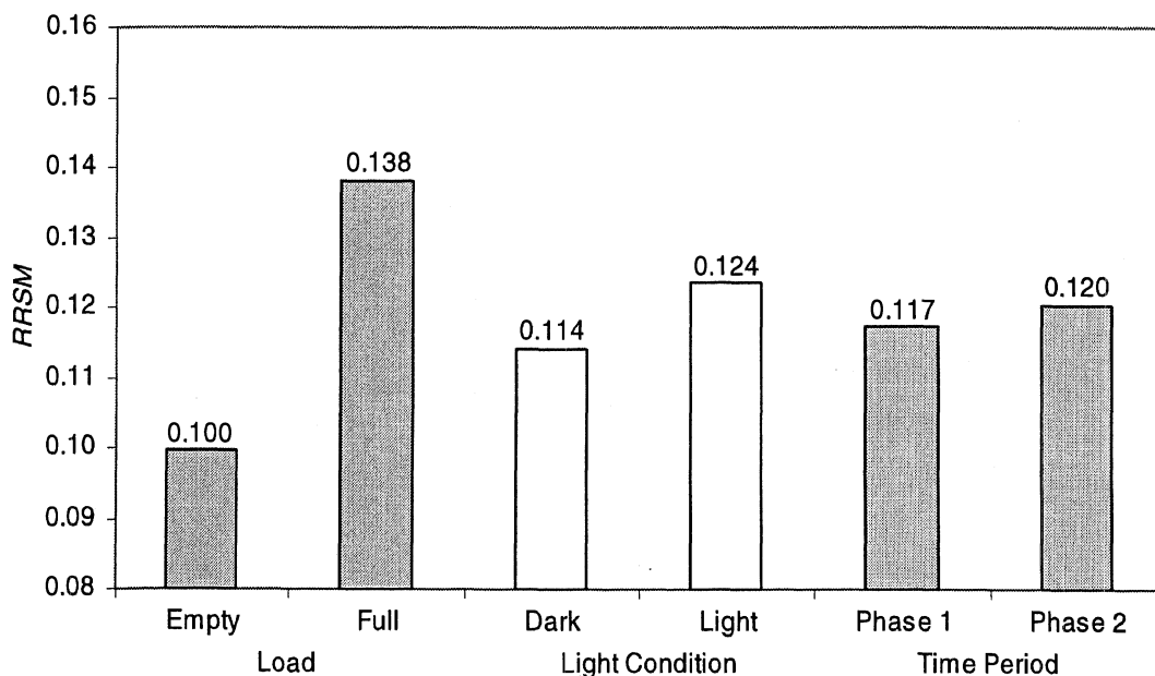
Figure 8-31. Main effects of light condition and trailer load on RRSM
