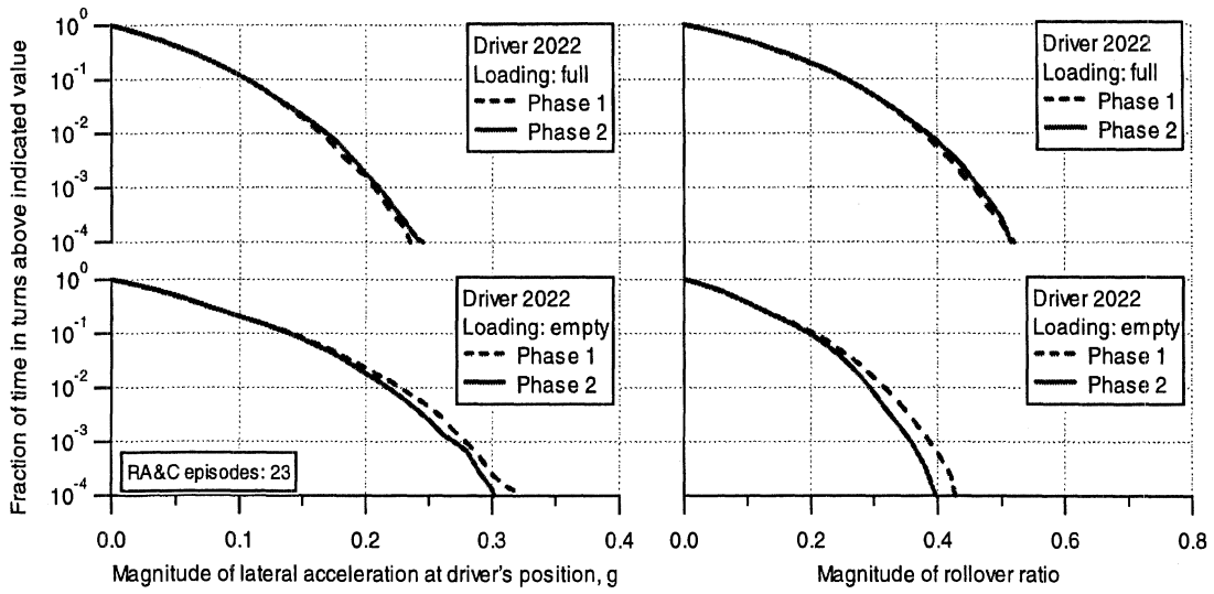
Figure 8-3. Comparison of phase-1 and phase-2 lateral performance in turns of driver 2022
