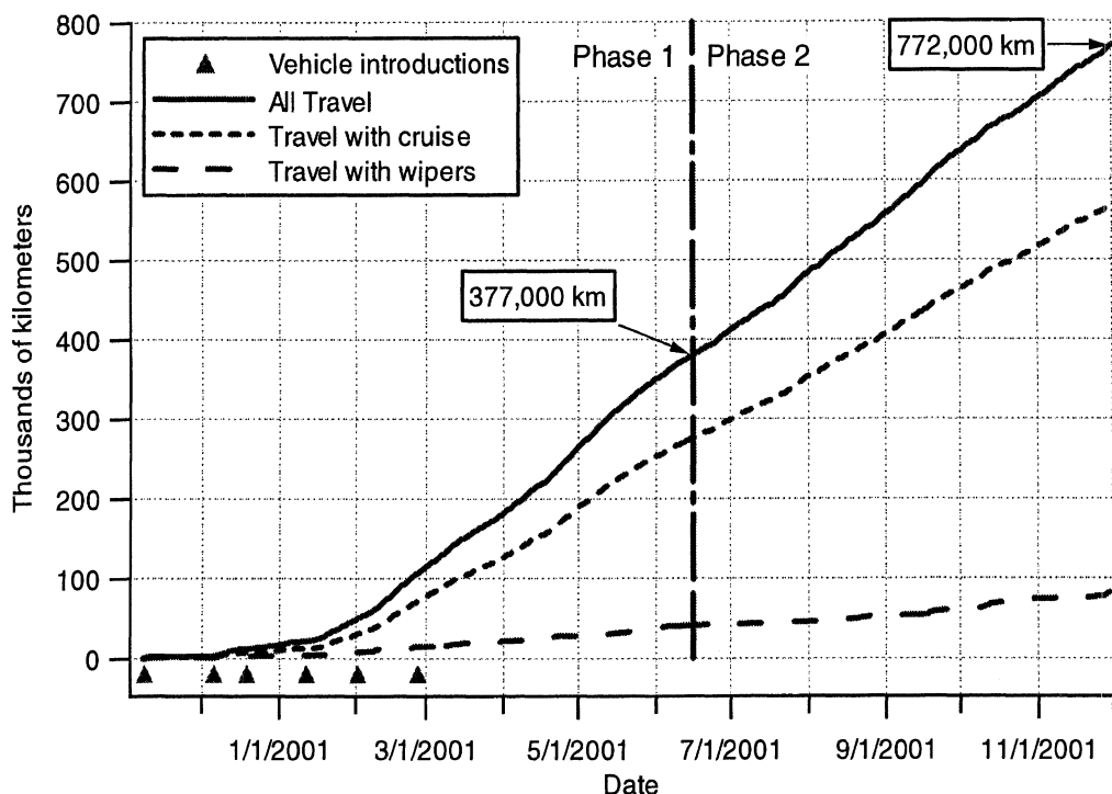
Figure 5-1. Accumulation of FOT travel distance in time
