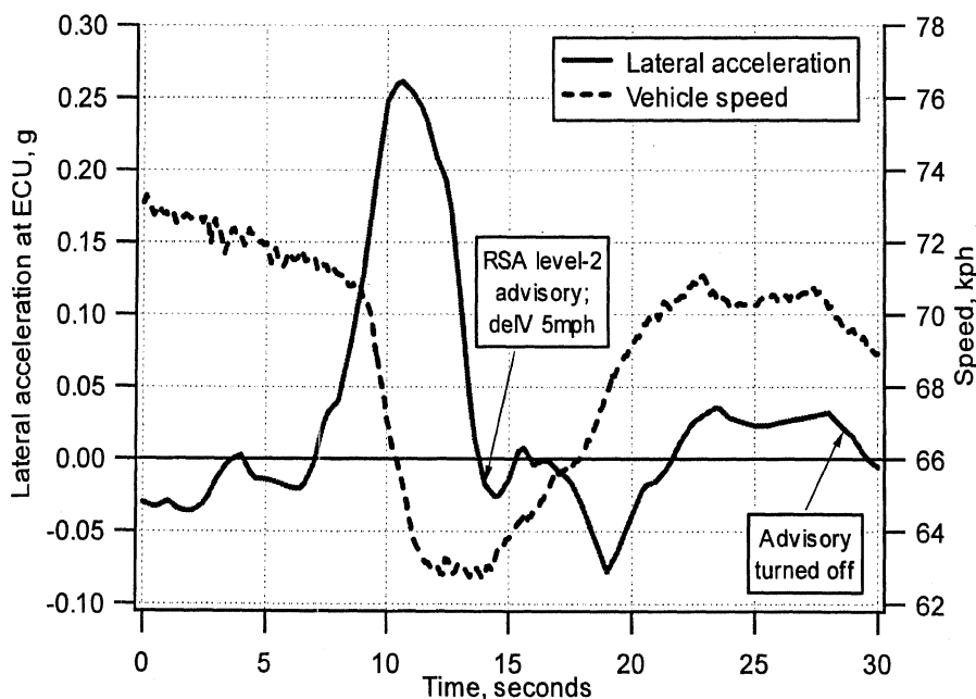
Figure 2-7. Time histories from an episode involving an RSA advisory
