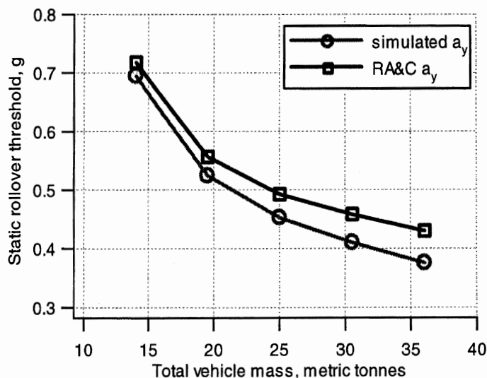
Figure A-C3. Results from the tilt-table tests (averages)
