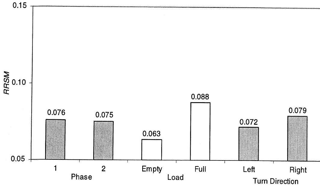
Figure 8-45. Main effects of phase, load, and turn direction on RRSM in off-roadway turns
