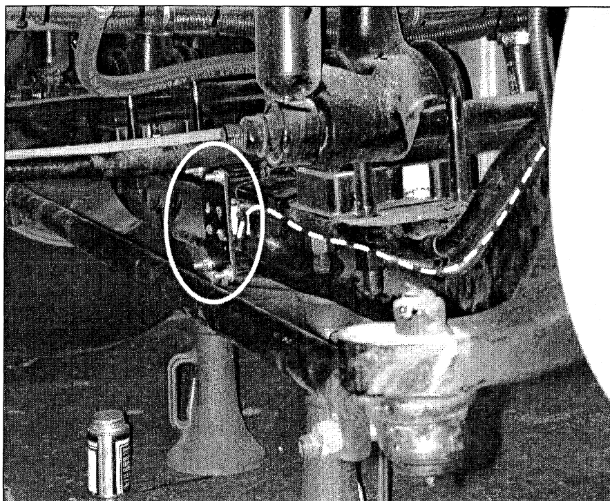
Figure A-E1. Front-axle lateral accelerometer housing, mount, wiring path and location.
