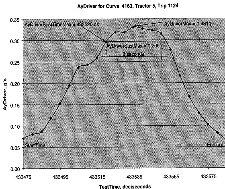
Figure 4-14. Example calculation of maximum and sustained maximum for curve performance
