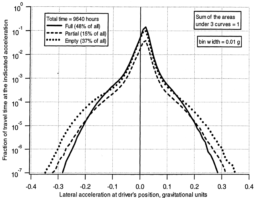
Figure 6-1. Histogram of travel time by lateral acceleration for three load ranges
