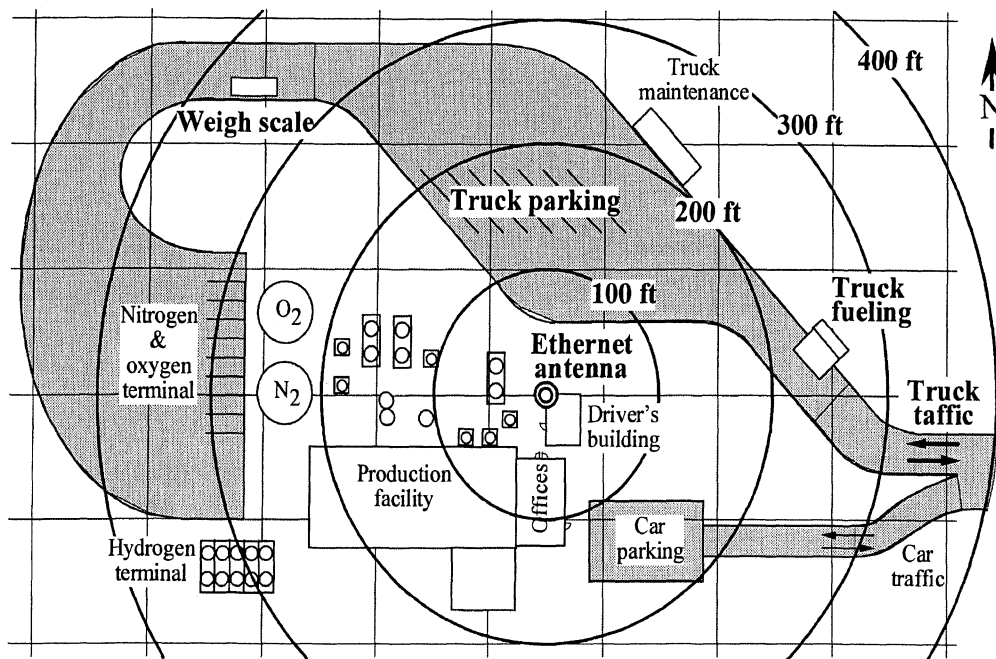
Figure 3-14. Plane view of the Praxair facility at La Porte
