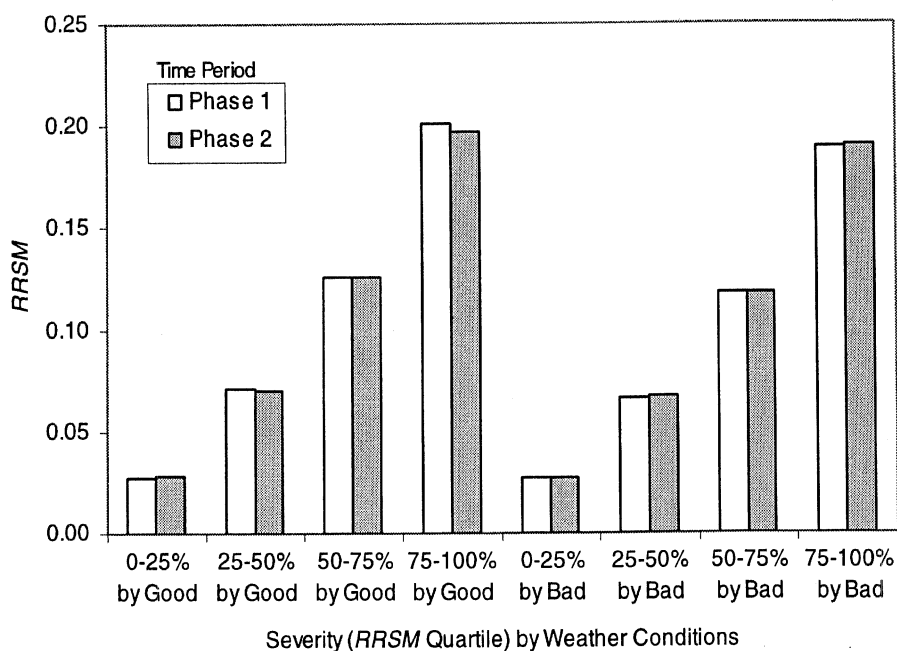
Figure 8-29. Three way interaction between weather, phase, and curve severity
