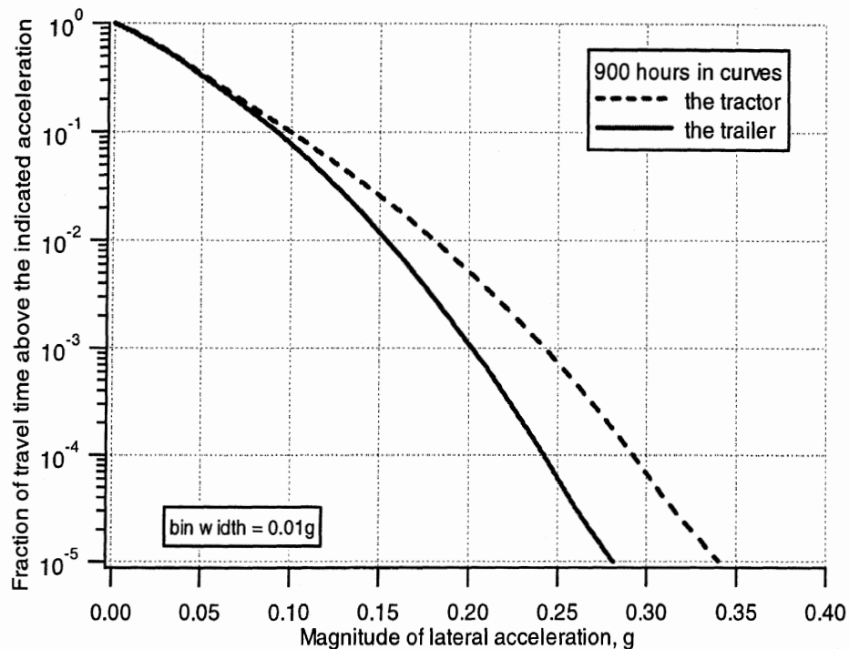
Figure 6-7. Cumulative histogram of travel time in curves by magnitude of lateral acceleration of the tractor ( AyDriver ) and the trailer ( AyTrailer )
