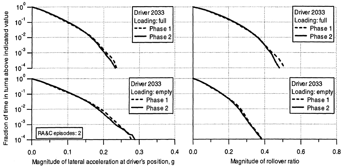
Figure 8-12. Comparison of phase-1 and phase-2 lateral performance in turns of driver 2033
