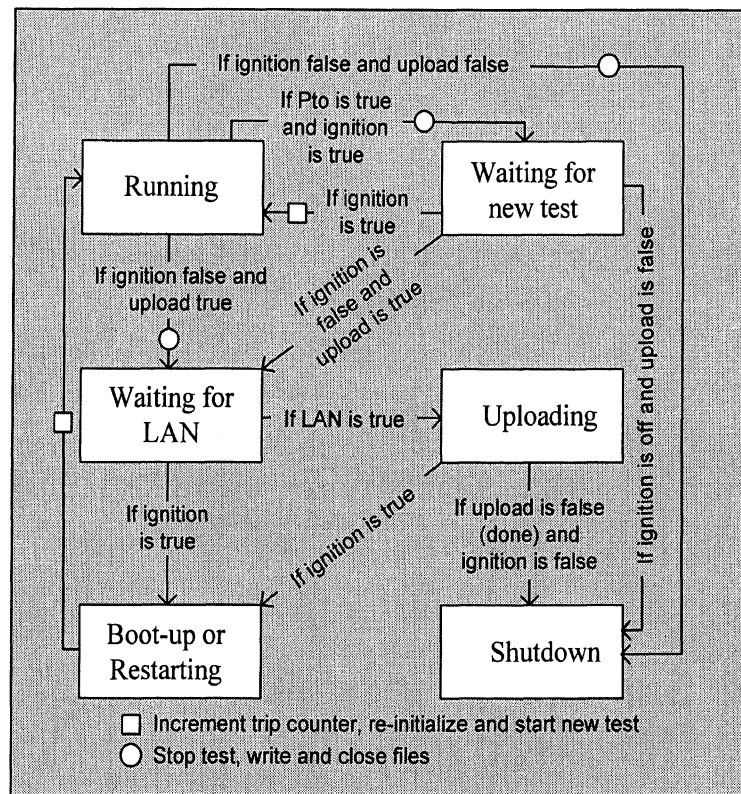
Figure 3-13. Control modes and logic for the FOT DAS
