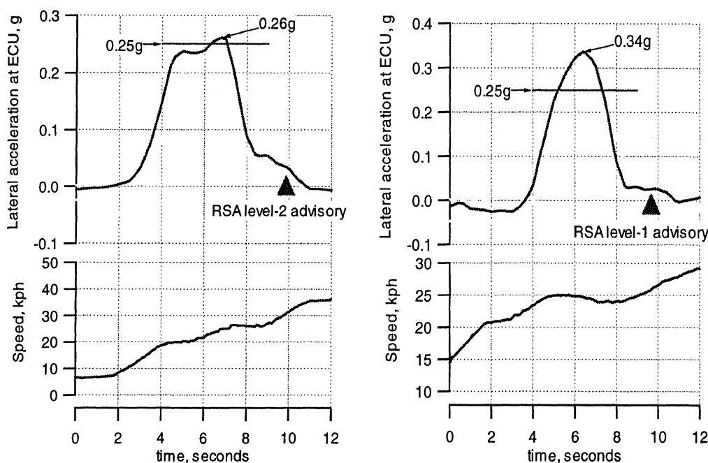
Figure 7-10. Time histories from a simple RSA-2 and a simple RSA-1 episode
