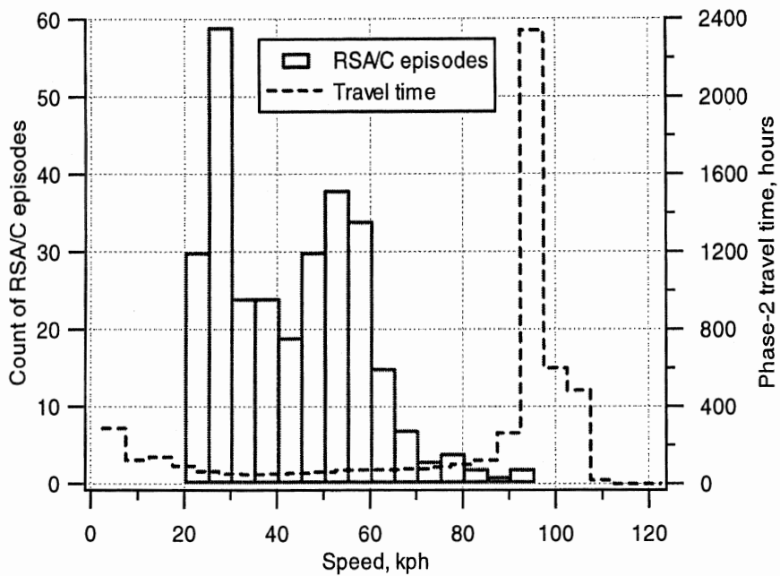
Figure 7-5. Comparing distributions by speed of RSA/C episodes and travel time
