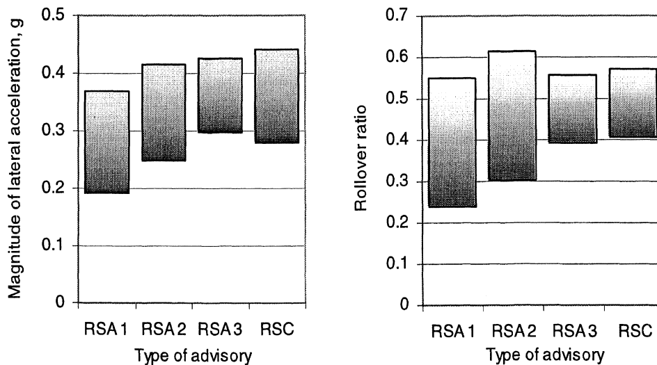
Figure 10-2. Ranges of the maximum magnitude of lateral acceleration and rollover ratio associated with RSA/C advisory messages
