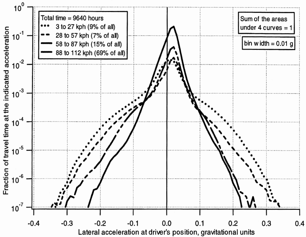
Figure 6-3. Histogram of travel time by lateral acceleration for four speed ranges
