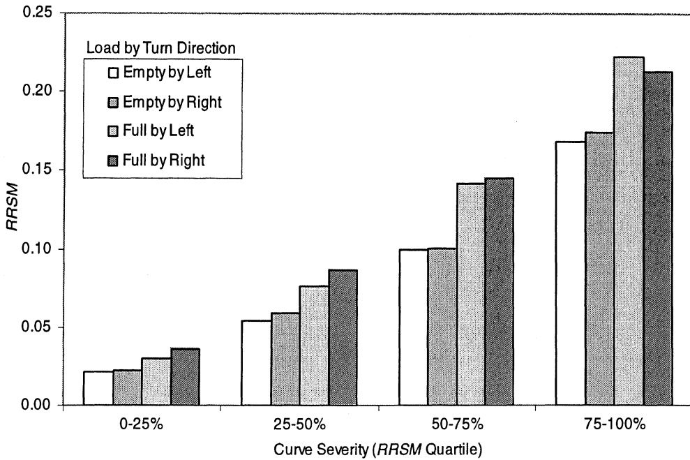
Figure 8-27. Three way interaction between load, turn direction, and curve severity
