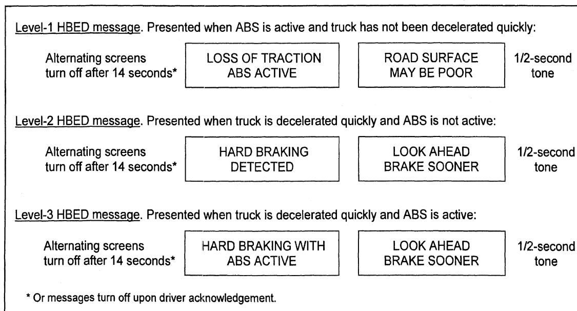
Figure 2-5. HBED advisory messages
