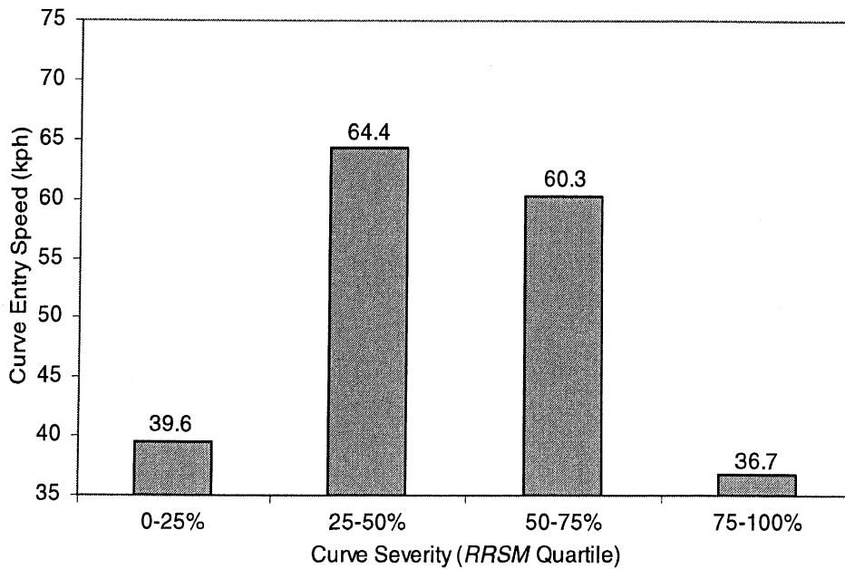
Figure 8-42. Curve-entry speed by curve severity bin
