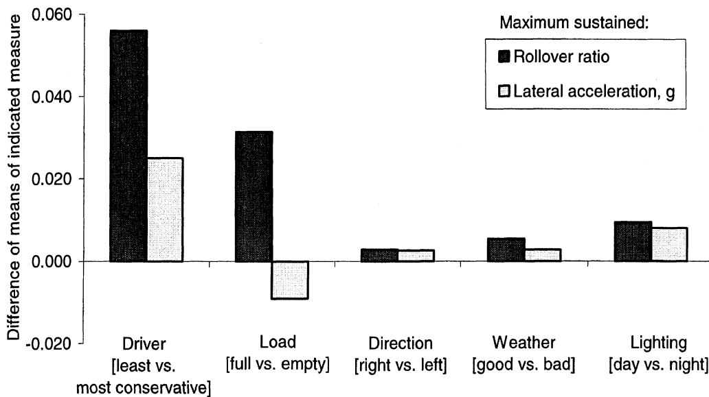
Figure 10-1. Relative strengths of different factors on turning performance 38
