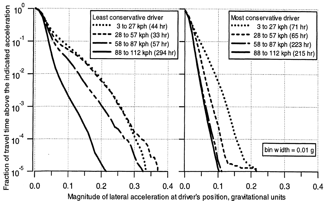
Figure 6-14. Cumulative histograms of travel time in turns by magnitude of lateral acceleration comparing the most and least conservative drivers
