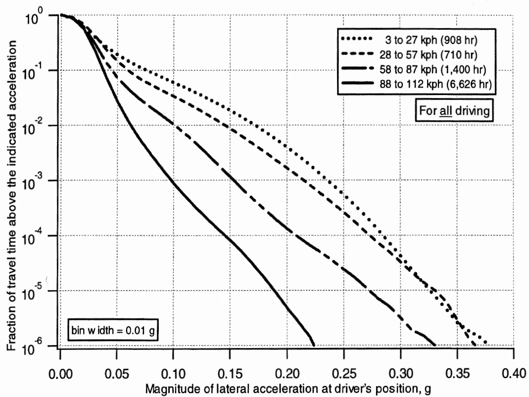
Figure 6-4. Cumulative histogram of travel time by magnitude of lateral acceleration for four speed ranges
