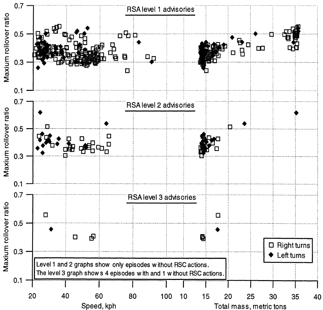
Figure 7-11. Maximum rollover ratio by speed and load for RSA episodes
