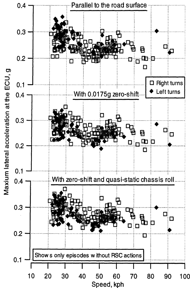
Figure 7-8. Progressive treatments of maximum lateral acceleration signal from RSA level-1 episodes
