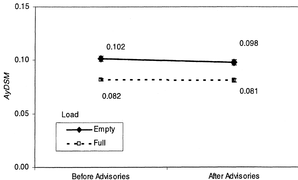
Figure 8-51. Main effects of exposure to advisory messages and load on AyDSM in the interval 500 km before and after an advisory
