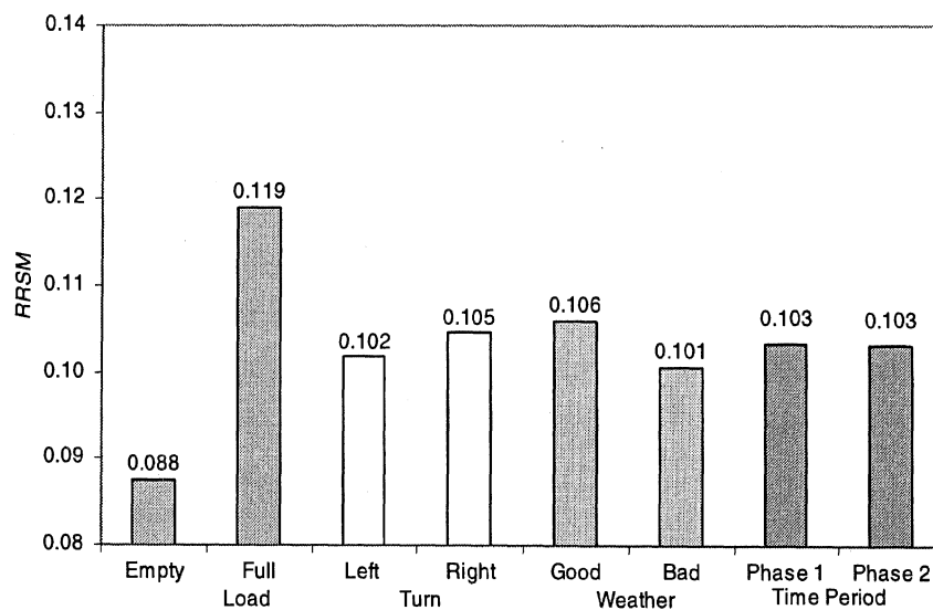
Figure 8-22. Main effects of load, turn direction, and weather on RRSM
