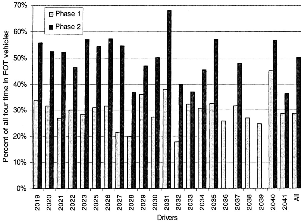
Figure 5-11. Percentage of all driving time spent in RA&C FOT tractors, driver by driver
