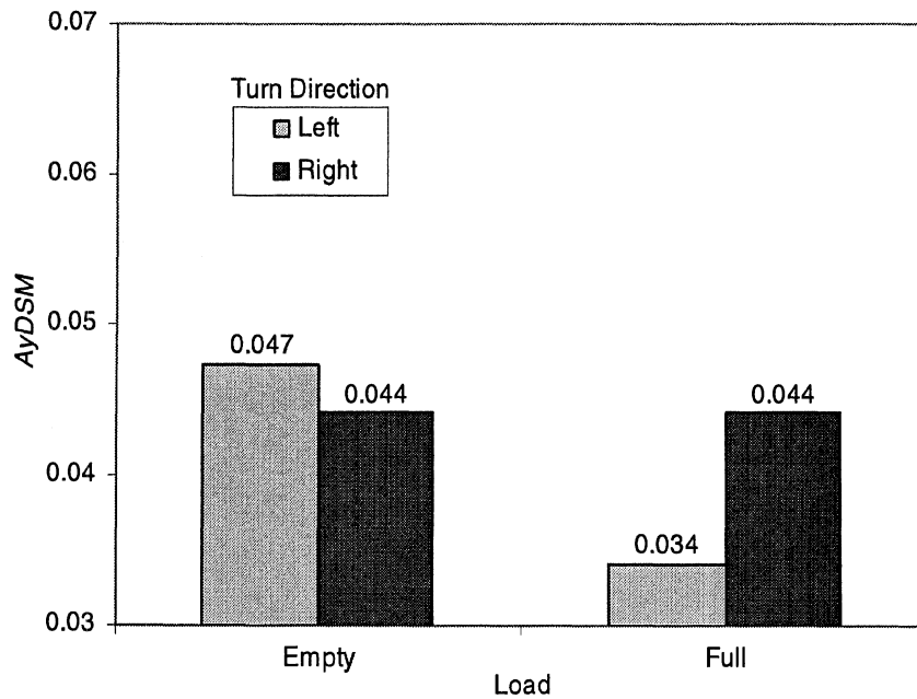
Figure 8-48. Interaction between load and turn direction on AyDSM
