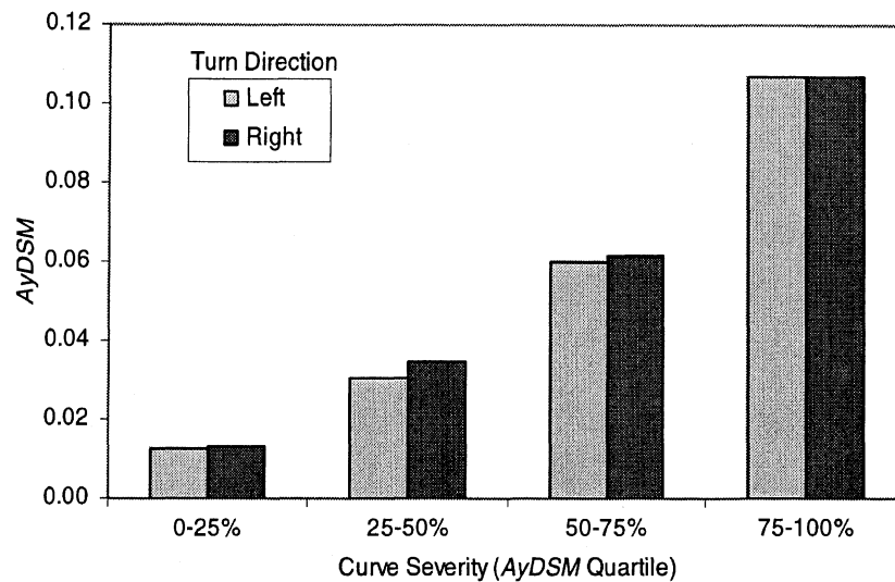
Figure 8-40. Two-way interaction between turn direction and curve severity on AyDSM quartile
