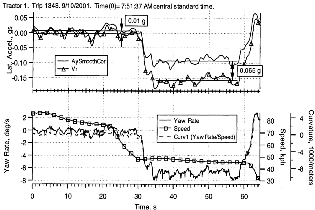
Figure 4-9. Lateral acceleration based on yaw rate and speed
