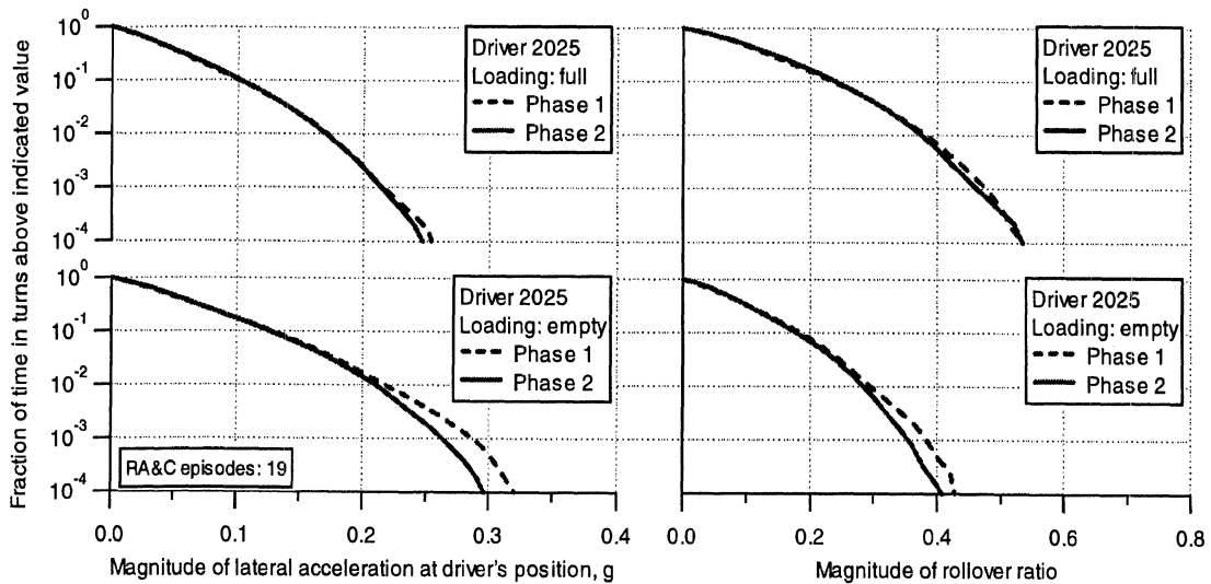
Figure 8-5. Comparison of phase-1 and phase-2 lateral performance in turns of driver 2024
