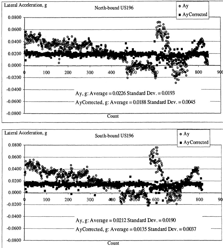
Figure A-E7. Distribution of corrected and uncorrected lateral acceleration at a validation site
