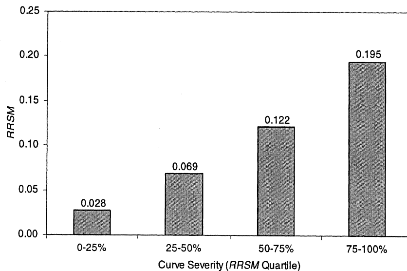
Figure 8-23. RRSM observed among the comparable drivers over curve severity derived from the RRSM performance of non-comparable drivers
