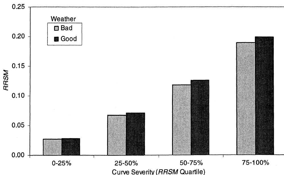
Figure 8-24. The interaction between weather and curve severity
