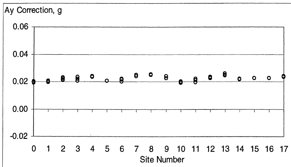
Figure A-E4. Lateral acceleration correction for transducer drift and instrument offset
