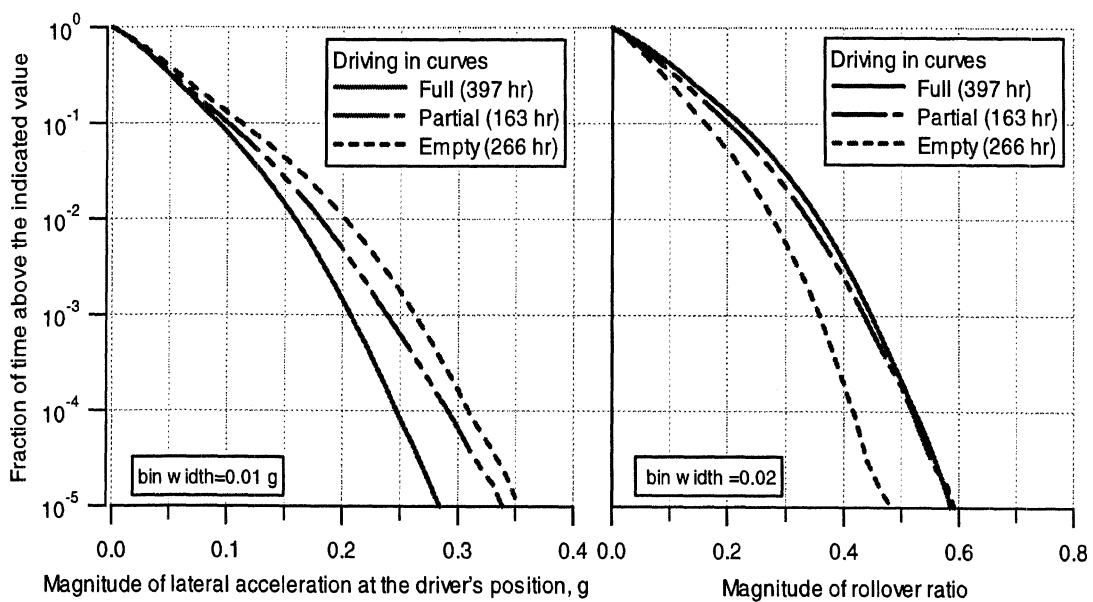
Figure 6-10. Cumulative histograms of travel time in curves for lateral acceleration ( A_{yDriver} ) and rollover ratio by loading condition
