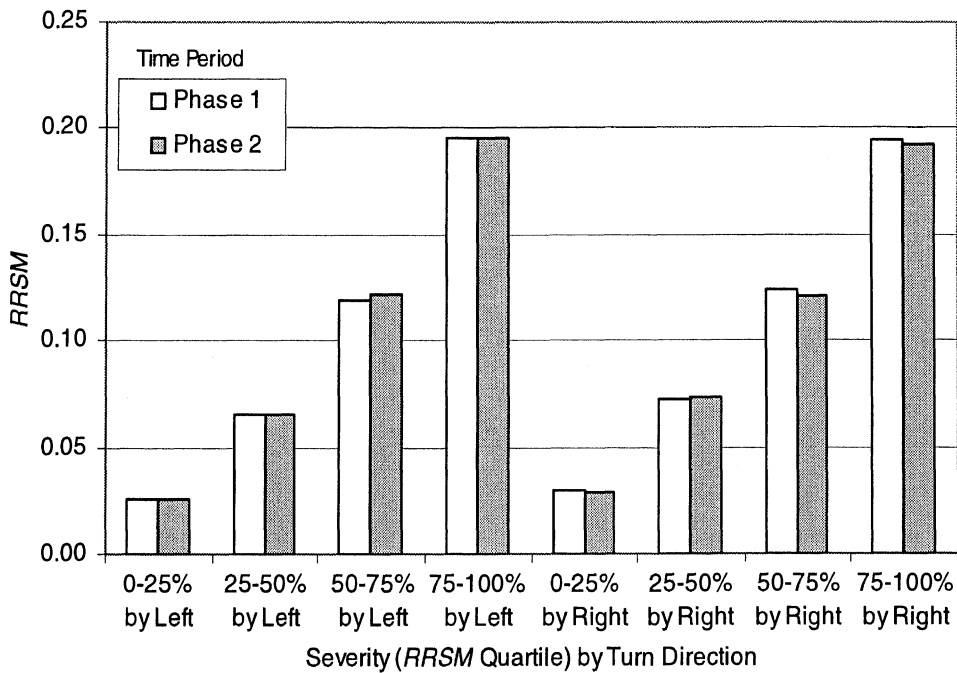
Figure 8-28. Three way interaction between phase, turn direction, and curve severity
