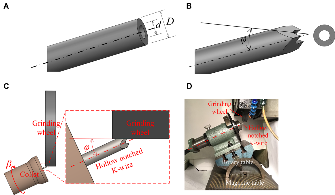
Figure 3. Bevel plane grinding of the hollow notched K-wire: (A) original hollow tube, (B) hollow tube with three bevel planes, (C) tip grinding configuration, and (D) experimental setup of the tip grinding. [Color figure can be viewed at wileyonlinelibrary.com ]
