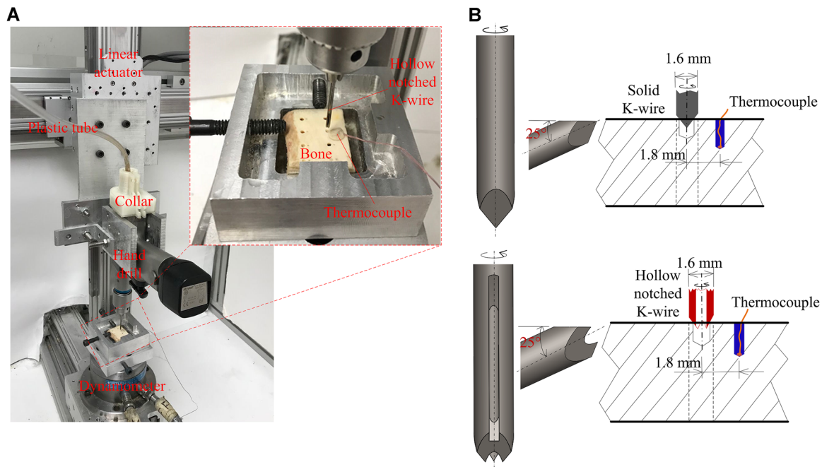
Figure 7. Bone drilling tests: (A) experimental setup and (B) drilling configurations for solid and hollow notched K-wires. [Color figure can be viewed at wileyonlinelibrary.com]
