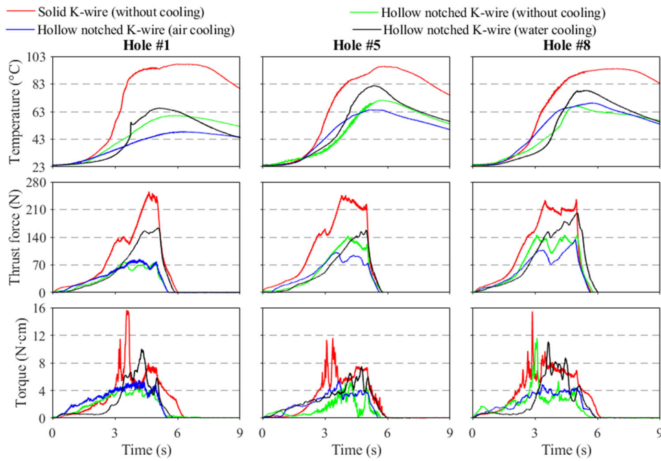
Figure 9. Comparison of temperature, thrust force, and torque in holes #1, #5, and #8. [Color figure can be viewed at wileyonlinelibrary.com]
