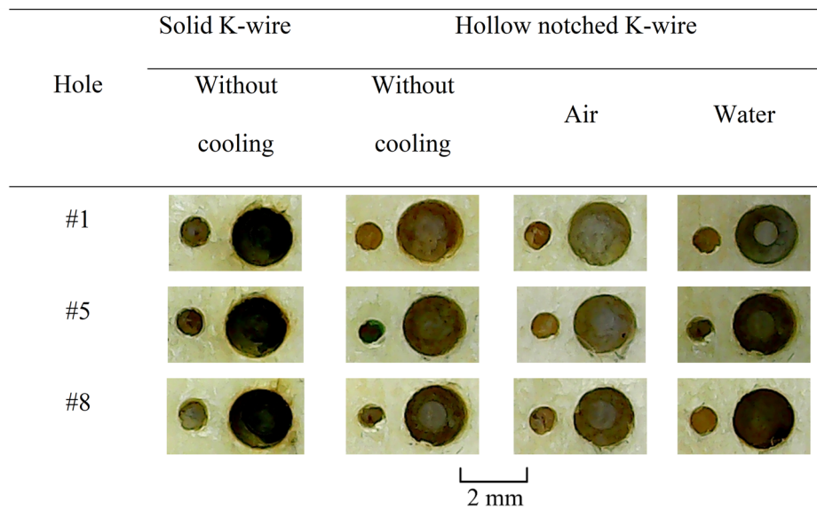
Figure 10. Comparison of drilled holes #1, #5, and #8 under four drilling conditions. [Color figure can be viewed at wileyonlinelibrary.com]
