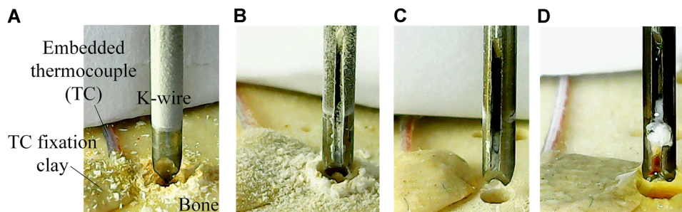
Figure 8. Bone debris after first bone drilling test under each condition: (A) solid Kirschner wire (K-wire) drilling without cooling, (B) hollow notched K-wire drilling without cooling, (C) hollow notched K-wire drilling with through-tool compressed air cooling, and (D) hollow notched K-wire drilling with through-tool water cooling. [Color figure can be viewed at wileyonlinelibrary.com]
