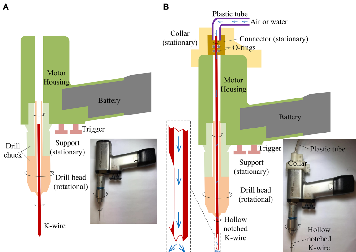
Figure 2. Surgical hand drill: (A) original configuration and (B) the collar adaptor and plastic tube for through-tool cooling. [Color figure can be viewed at wileyonlinelibrary.com ]
