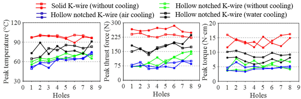
Figure 11. Change of peak bone temperature rise, thrust force, and torque along with number of holes drilled under four drilling conditions in two repeated trials. [Color figure can be viewed at wileyonlinelibrary.com]
