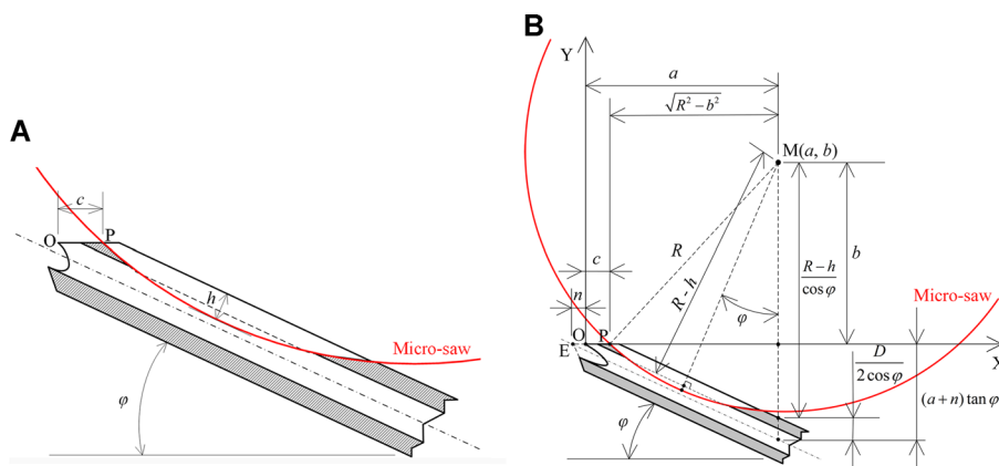
Figure 5. Notch micro-milling of the hollow notched K-wire: (A) notch configuration and (B) end position of the micro-saw. [Color figure can be viewed at wileyonlinelibrary.com]
