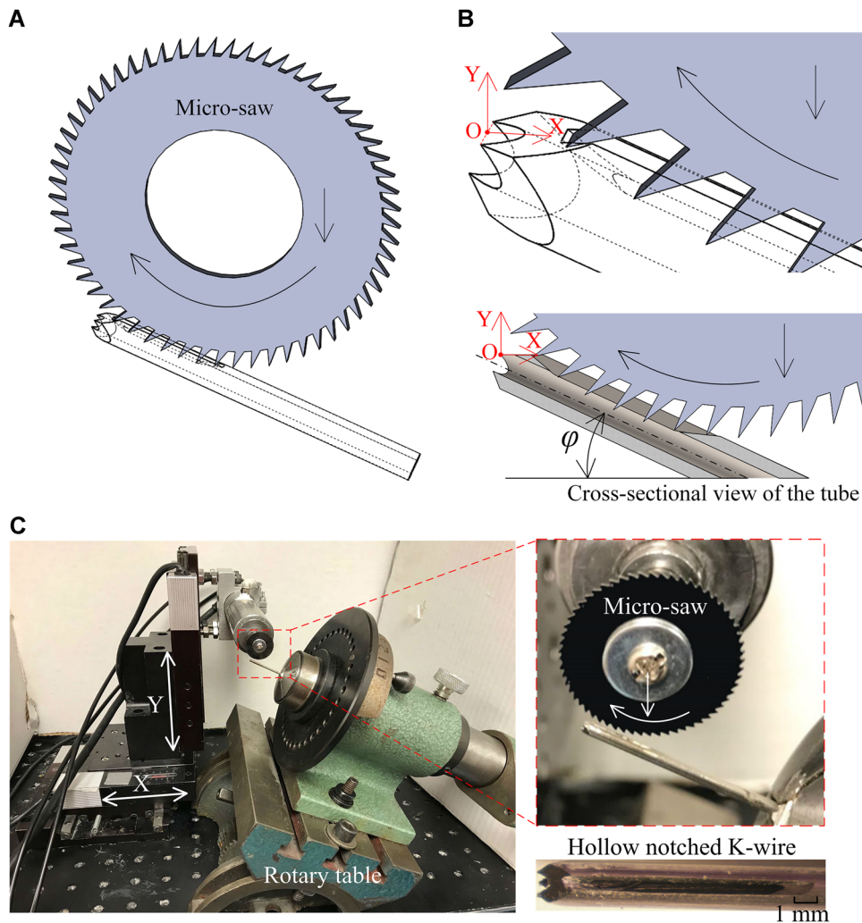
Figure 4. Notch micro-milling of the hollow notched Kirschner wire (K-wire): (A) overview and (B) close-up and cross-sectional views of the micro saw and hollow wire configuration and (C) the experimental setup. [Color figure can be viewed at wileyonlinelibrary.com ]
