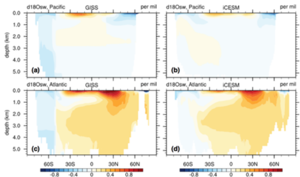
Figure 9. Model-data comparison of zonal mean seawater \delta^{18}\text{O} (unit: ‰). Pacific zonal mean in (a) the GISS data set and (b) the iCESM simulation averaged between year 1955 and 2005. (c and d) Same as in (a) and (b) but for the Atlantic zonal mean.
