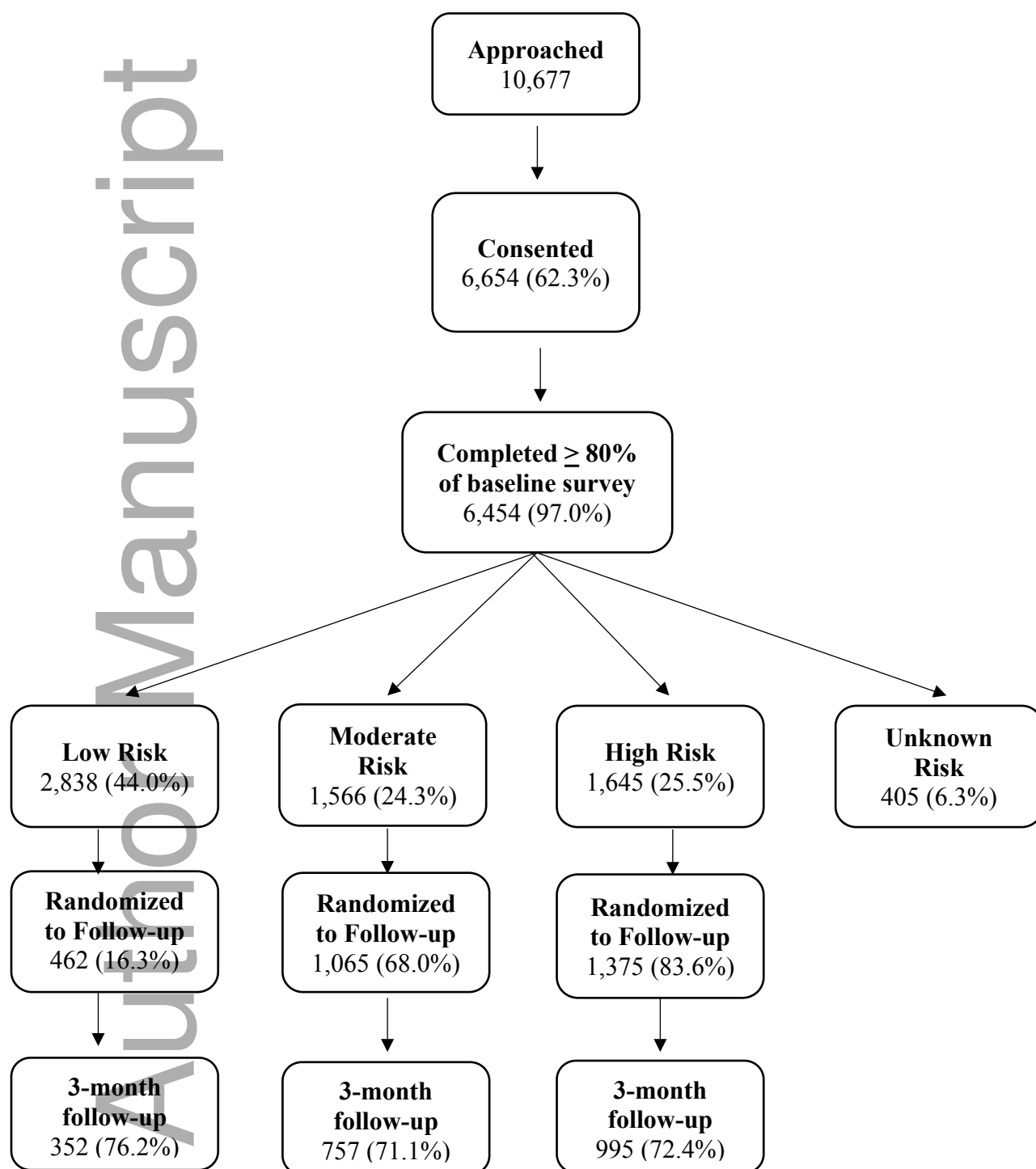
Figure 1. Participant flow
