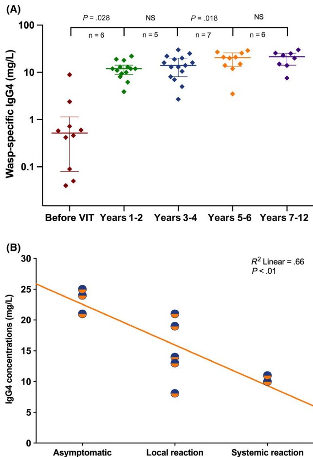
FIGURE 3 A, Dynamic of wasp-specific IgG4 levels in cMCD patients during VIT. Two outliers were identified (2.4 and 8.9 mg/L, respectively) at baseline, and both patients previously received VIT. P -values were analysed with Wilcoxon's matched pair rank sum test. A significant increase was noted between baseline and years 1-2 ( P = .028 ) and between years 3-4 and years 5-6 ( P = .018 ). n ; number of matched patients at different time points. Different colours represent different time periods. B, Correlation between wasp-specific IgG4 levels and severity of re-sting reaction. The reactions were classified as asymptomatic, local reactions (<10 cm in diameter) and mild systemic reactions (without respiratory or circulatory compromise). Correlation was quantified by using Spearman's rank correlation coefficient
