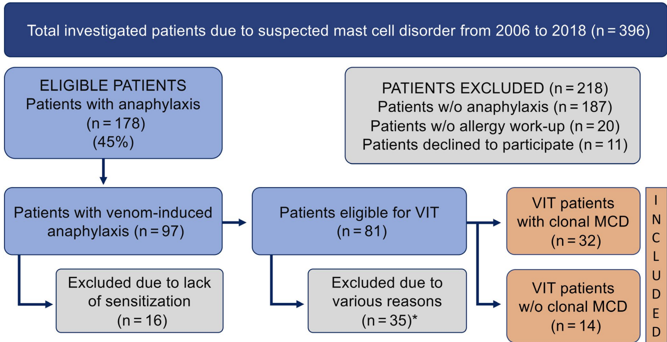
FIGURE 1 The flow chart illustrates the selection process of the study subjects. *35 patients were excluded due to various reasons (15 received VIT at other clinics, 7 had elevated baseline tryptase levels without underlying cMCD, 6 declined to undergo VIT, 4 had comorbidities with cancer, two patients were investigated during study start, and 1 patient was sensitized for honeybee only). Abbreviations: w/o, without; VIT, venom immunotherapy; MCD, mast cell disorders
