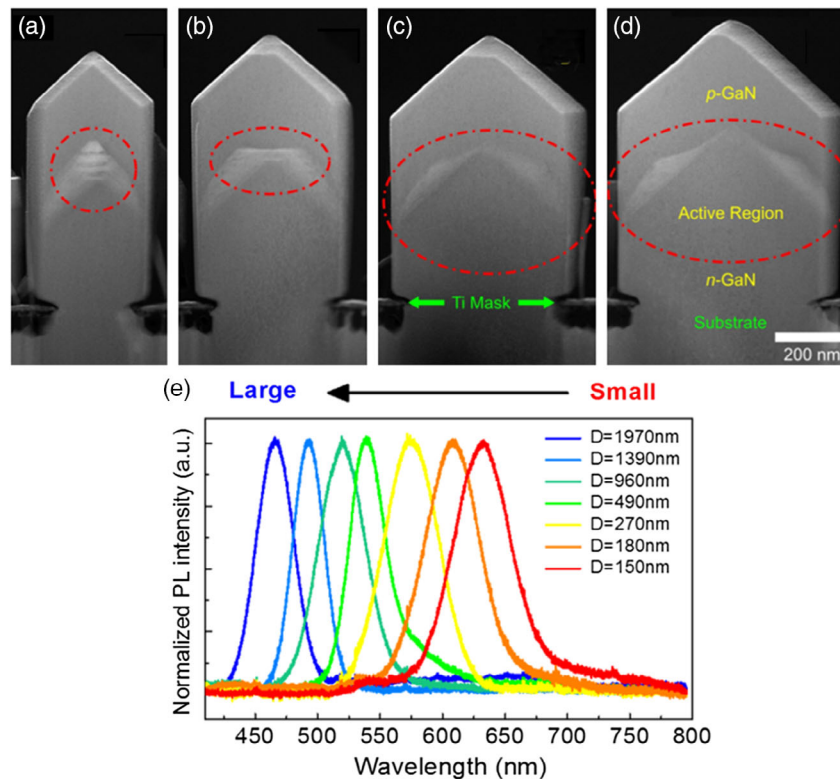
Figure 5. a–d) STEM-HAADF images for single nanocrystals with different diameters. [60] e) Normalized PL spectra for single nanocrystals with different diameters grown on the same substrate. Reproduced with permission. [60] Copyright 2016, American Chemical Society.
