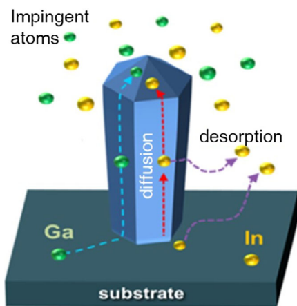
Figure 3. Schematic for the surface dynamics of In and Ga adatoms during the growth of InGaN nanocrystals. Reproduced with permission. [60] Copyright 2016, American Chemical Society.
