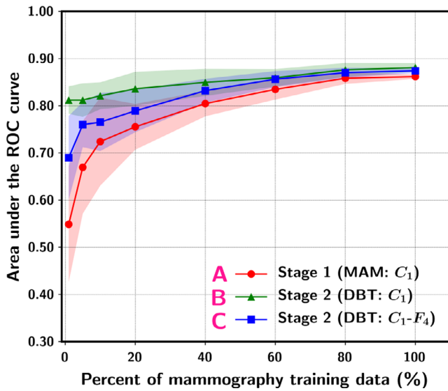
FIG. 1. Regions of interest-based area under the receiver operating characteristic curve (AUC) performance on the digital breast tomosynthesis (DBT) test set while varying the simulated mammography sample size available for training. The data point and the upper and lower range show the mean and standard deviation of the test AUC resulting from 10 random samplings of the training set of a given size from the original set. “A. Stage 1 (MAM: C_1 )” denotes single-stage training using mammography data and the C_1 -layer of the ImageNet pretrained AlexNet frozen during transfer learning without stage 2. “B. Stage 2 (DBT: C_1 )” denotes stage 2 C_1 -frozen transfer learning at a fixed (100%) DBT training set size after stage 1 transfer learning (curve A). “C. Stage 2 (DBT: C_1-F_4 )” denotes stage 2 C_1 -to- F_4 -frozen transfer learning at a fixed (100%) DBT training set size after stage 1 transfer learning (curve A). [reprint with permission 50 ].
