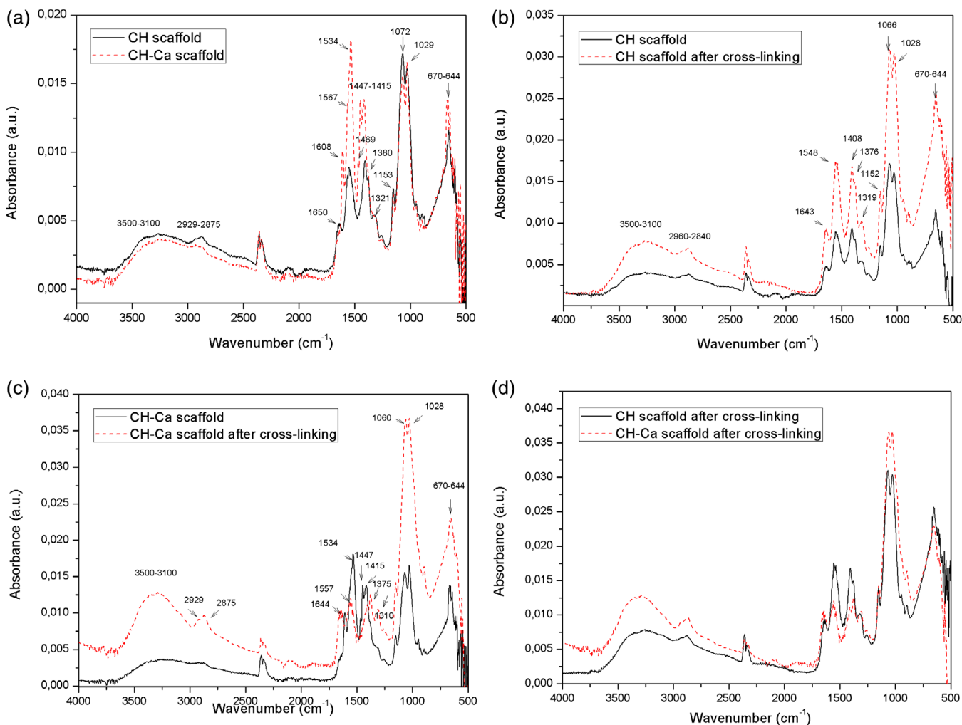
FIGURE 3 FTIR spectrum comparing (a) CH and CH-Ca scaffold before cross-linking; (b) CH before and after cross-linking; (c) CH-Ca before and after cross-linking; and (d) CH and CH-Ca scaffold after cross-linking
