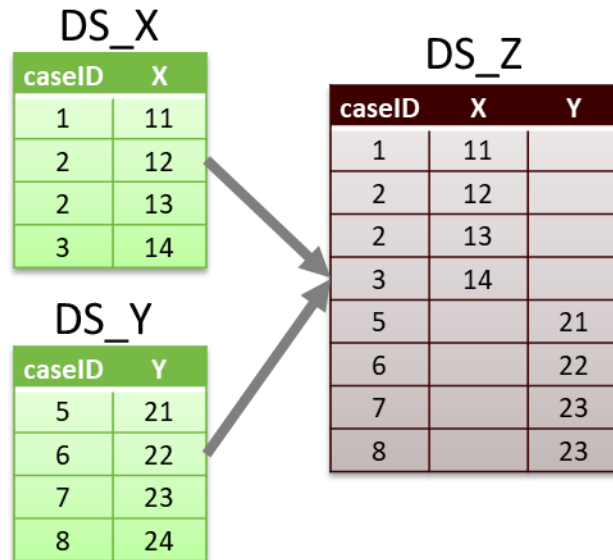
Figure 3. Appending Datasets
