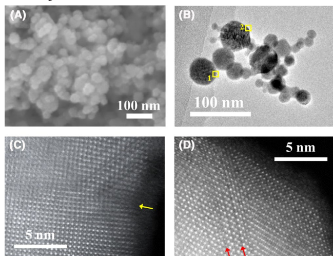
FIGURE 2 (A) SEM image and (B) STEM image of LF-FSP NP. HAADF-STEM images of (C) area 1 and (D) area 2 in image (B) [Color figure can be viewed at wileyonlinelibrary.com ]
