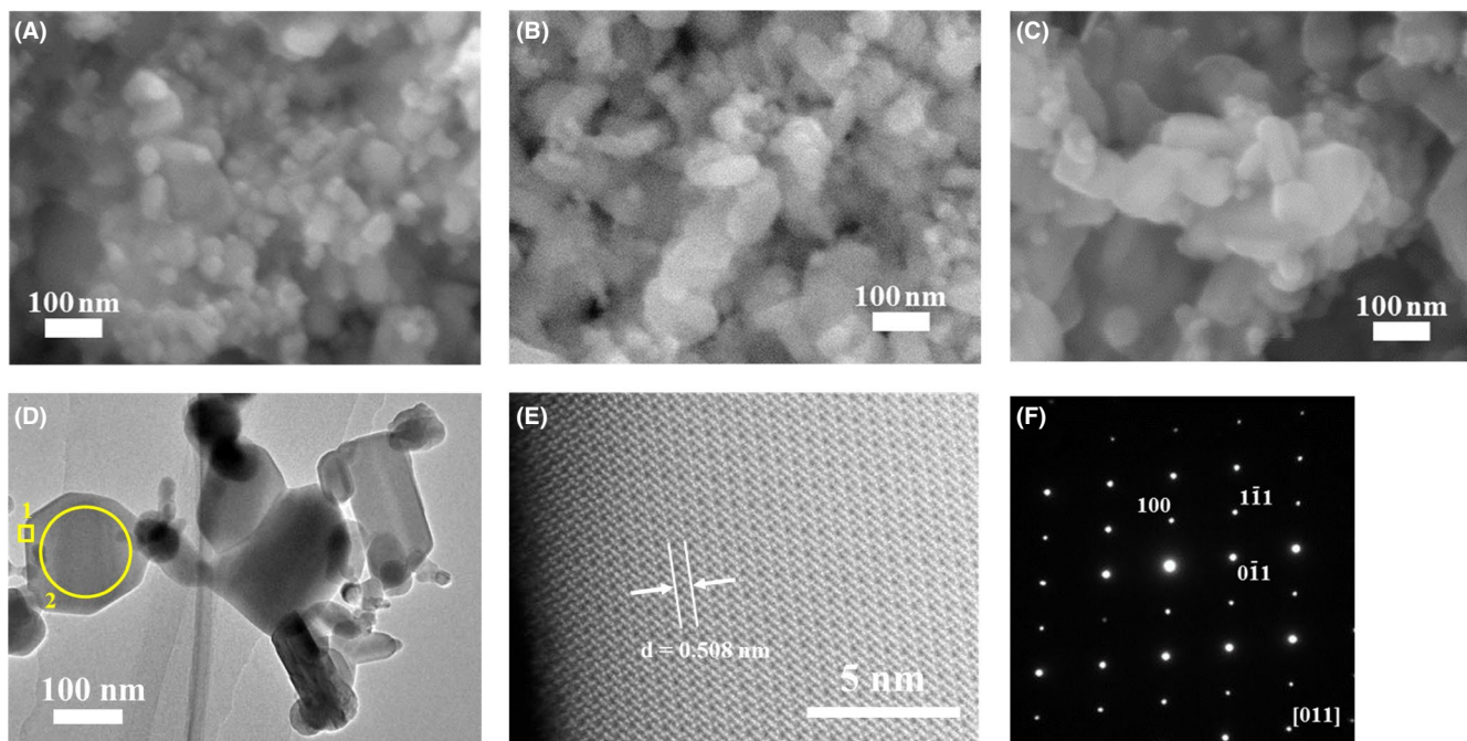
FIGURE 7 SEM images of NPs heat-treated at (A) 1000°C/1.5 h/air, (B) 1000°C/3 h/air and (C) 1000°C/6 h/air. (D) STEM image of NPs heat-treated at 1000°C/3 h/air. (E) HAADF-STEM image of area 1 in image (D) and (F) SAED of area 2 in image (D) [Color figure can be viewed at wileyonlinelibrary.com ]
