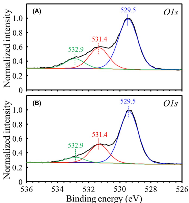
FIGURE 8 XPS of O1s region for (A) LF-FSP NPs and (B) NPs heat-treated at 1000°C/3 h/air [Color figure can be viewed at wileyonlinelibrary.com ]
