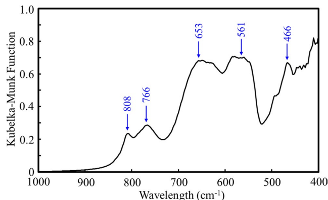
FIGURE 6 FTIR spectrum of NPs heat-treated at 1000°C/3 h/air [Color figure can be viewed at wileyonlinelibrary.com]
