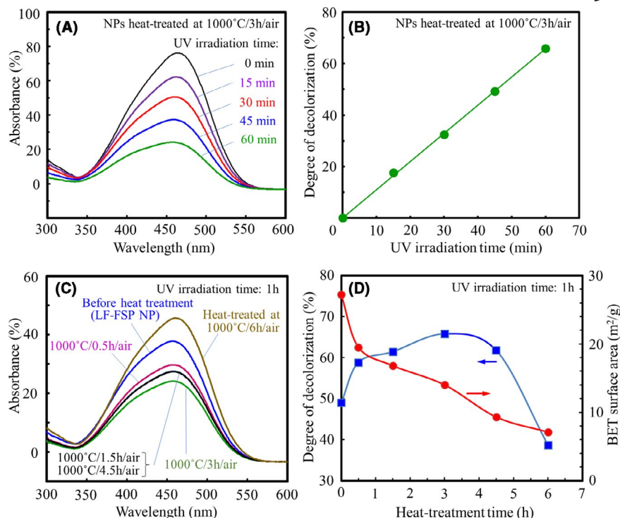
FIGURE 10 (A) Absorbance spectra of MO solution with NPs heat-treated at 1000°C/3 h/air after UV irradiation for different times. (B) Dependence of degree of decolorization on UV irradiation time for NPs heat-treated at 1000°C/3 h/air. (C) Absorbance spectra of MO solution without NPs and with NPs heat-treated at 1000°C/0-6 h/air after UV irradiation for 1 h. (D) Dependence of degree of decolorization and BET surface area on heat treatment time. Heat treatment was carried out at 1000°C/air. UV irradiation time was 60 min [Color figure can be viewed at wileyonlinelibrary.com]
