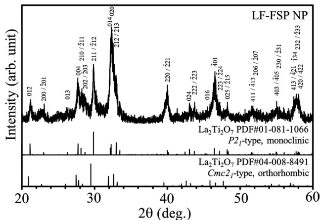
FIGURE 3 XRD pattern of LF-FSP NPs. Lattice planes corresponds to monoclinic P2_1 -type \text{La}_2\text{Ti}_2\text{O}_7
