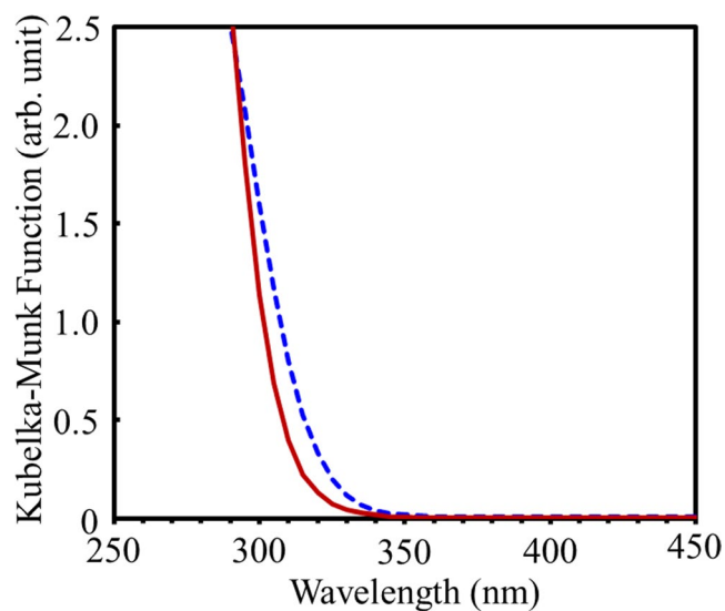
FIGURE 9 UV-vis diffused reflectance spectra of LF-FSP NP (blue dotted line) and that heat-treated at 1000°C/3 h/air (red solid line) [Color figure can be viewed at wileyonlinelibrary.com ]
