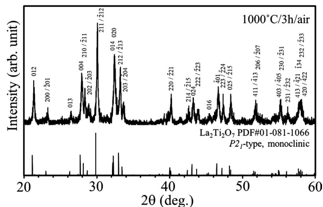
FIGURE 5 XRD pattern of NPs heat-treated at 1000°C/3 h/air
