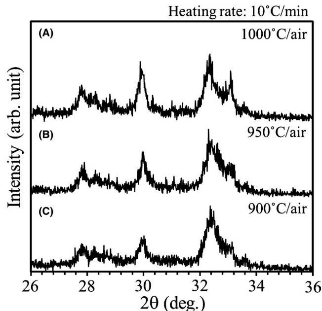
FIGURE 4 XRD patterns of heat-treated LF-FSP NPs. Heat-treat conditions; (A) 1000°C/0 h/air, (B) 950°C/0 h/air, (C) 900°C/0 h/air. Temperature raising speed: 10°C/min
