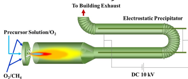
FIGURE 1 Schematic diagram of apparatus of liquid-feed flame spray pyrolysis [Color figure can be viewed at wileyonlinelibrary.com ]
