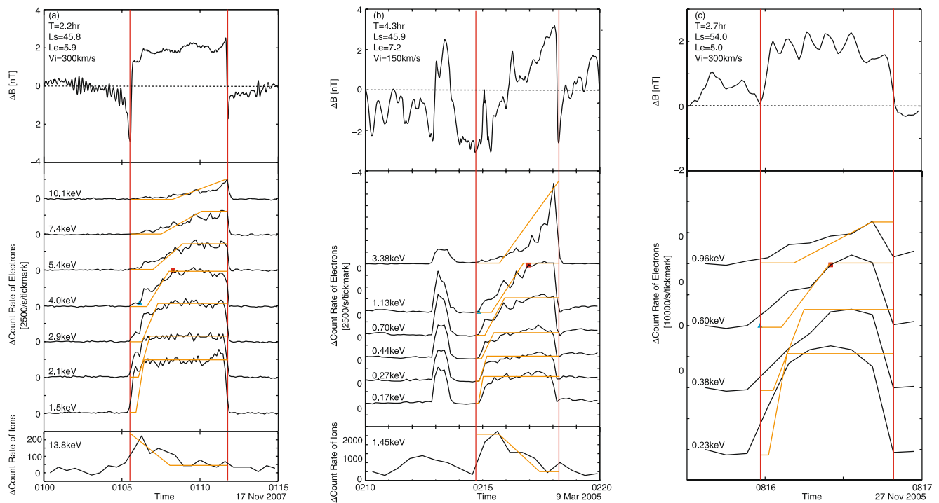
Figure 3. Comparisons of modeled distributions of electrons and ions against Cassini measurements during three flux tube events. All orange lines are modeled by assuming a constant return speed that varies from 150km/s to 300km/s.
