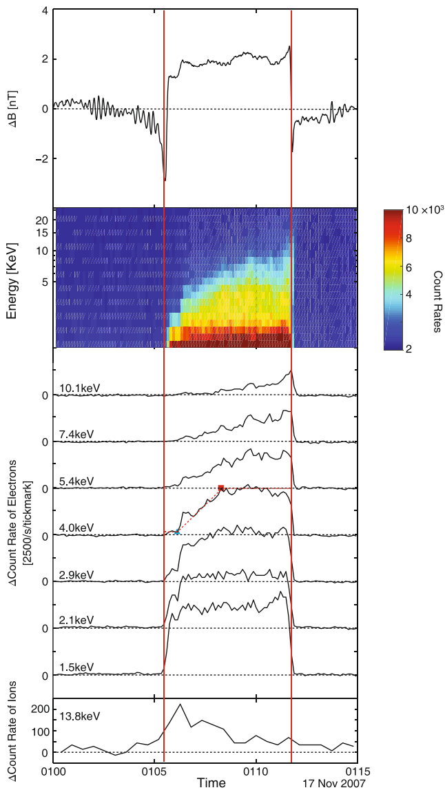
Figure 1. Detrended magnetic field and plasma profiles during the event on November 17, 2007 (Paranicas et al., 2016). The two vertical red lines mark the boundary of the flux tube that is empty of water group ions and has “floated” inward from the tail. The sinusoidal oscillations in the top panel are ion cyclotron waves induced by water group ions added by the Enceladus plume. This event was detected at a Saturn-centric distance of 5.9 R_s , a latitude of 3.19°, and a local time of 21.03 hr.
