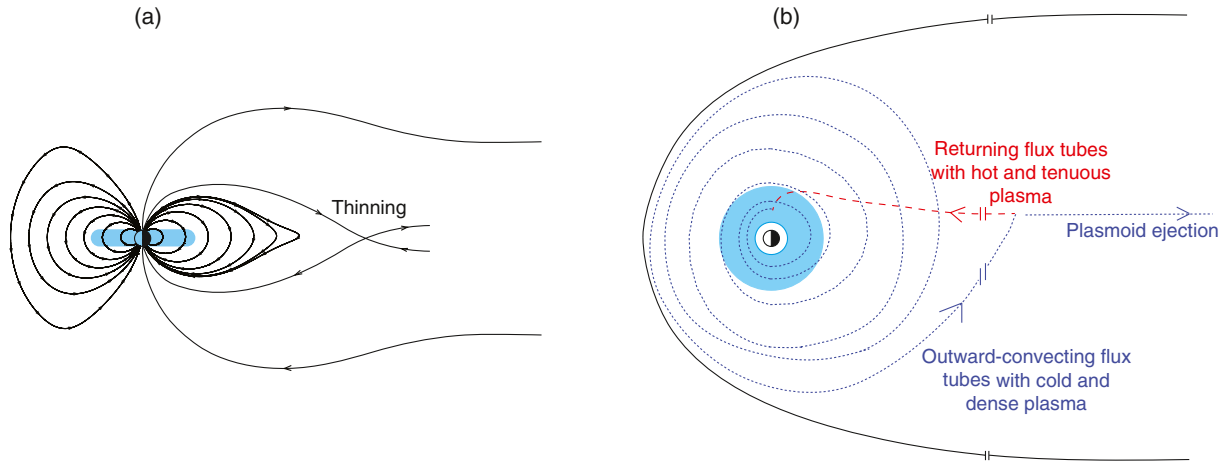
Figure 4. Illustration of the time-integrated circulation of magnetic flux in the Saturnian magnetosphere, indicated by our result. The blue ring is the neutral torus from Enceladus. (a) Black lines are magnetic field lines drawn until around the tail reconnection site in side view. (b) The black line marks the magnetopause. The blue dotted curve sketches the radially slow convection of plasma-loaded magnetic flux tubes spinning outward into the tail. The red dashed line indicates the return of plasma-depleted magnetic field tubes directly back to the inner magnetosphere at a higher radial speed. This red line may not end at the dawn side, but is not expected to wind multiple circles as indicated by the age estimation.
