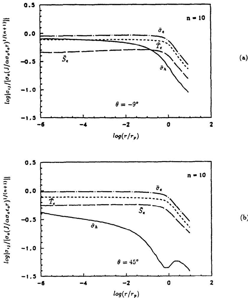
Fig. 11. Case 2 ( M_{12}^s = 0.5 , M_{13}^s = 0.39 and M_{23}^s = 0.39 ): the normalized effective stress \bar{\sigma}_e , the normalized effective in-plane shear stress \bar{S}_e , the normalized effective out-of plane shear stress \bar{T}_e , and the normalized hydrostatic stress \bar{\sigma}_h for n = 10 as functions of r/r_p plotted in a log-log scale at (a) \theta = -9^\circ , and (b) \theta = 45^\circ .
