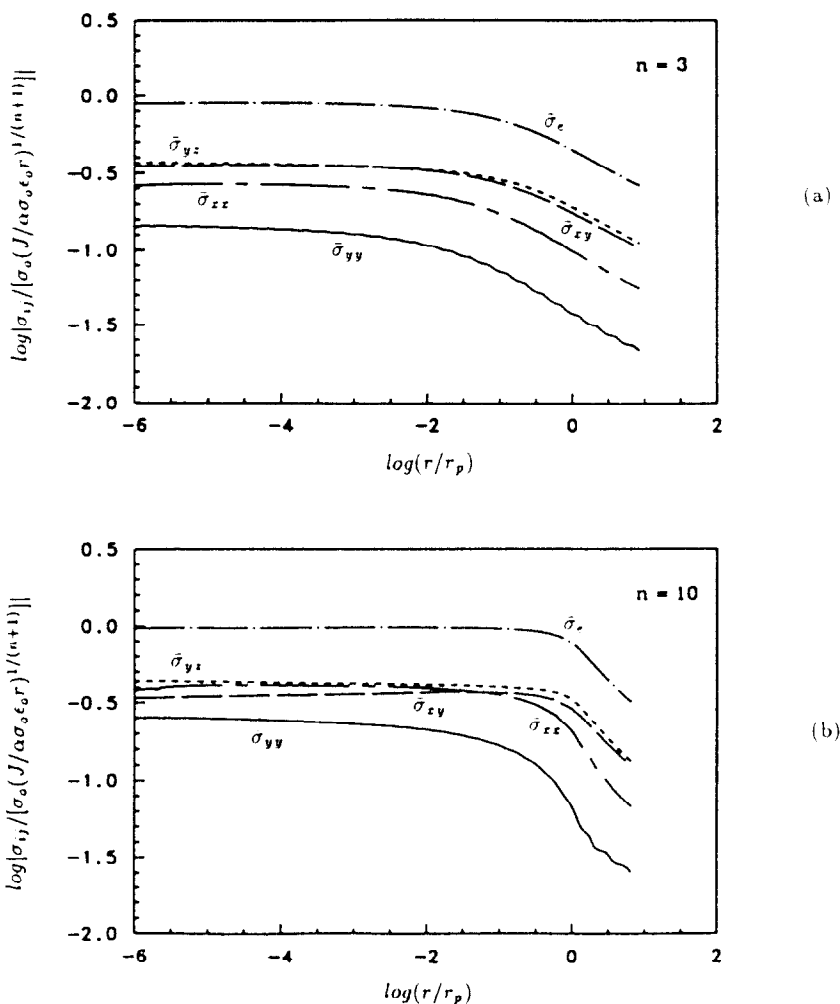
Fig. 5. Case 3 ( M_{12}^c = 0.17 , M_{11}^c = 0.16 and M_{21}^c = 0.49 ): the normalized stresses \bar{\sigma}_{ij} at \theta = -90^\circ as functions of r/r_p plotted in a log-log scale for (a) n = 3 , and (b) n = 10 .
