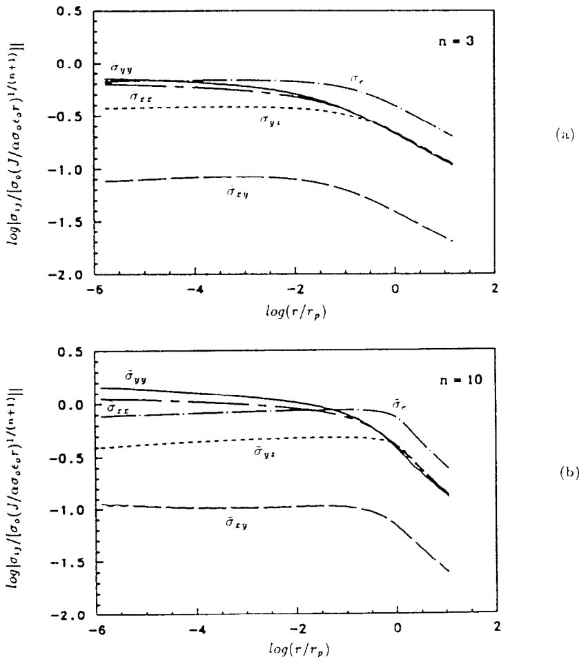
Fig. 3. Case 1 ( M_{I2}^e = 0.83 , M_{I3}^e = 0.49 and M_{I3}^e = 0.16 ): the normalized stresses \bar{\sigma}_{ij} at \theta = -9 as functions of r/r_p plotted in a log-log scale for (a) n = 3 , and (b) n = 10 .
