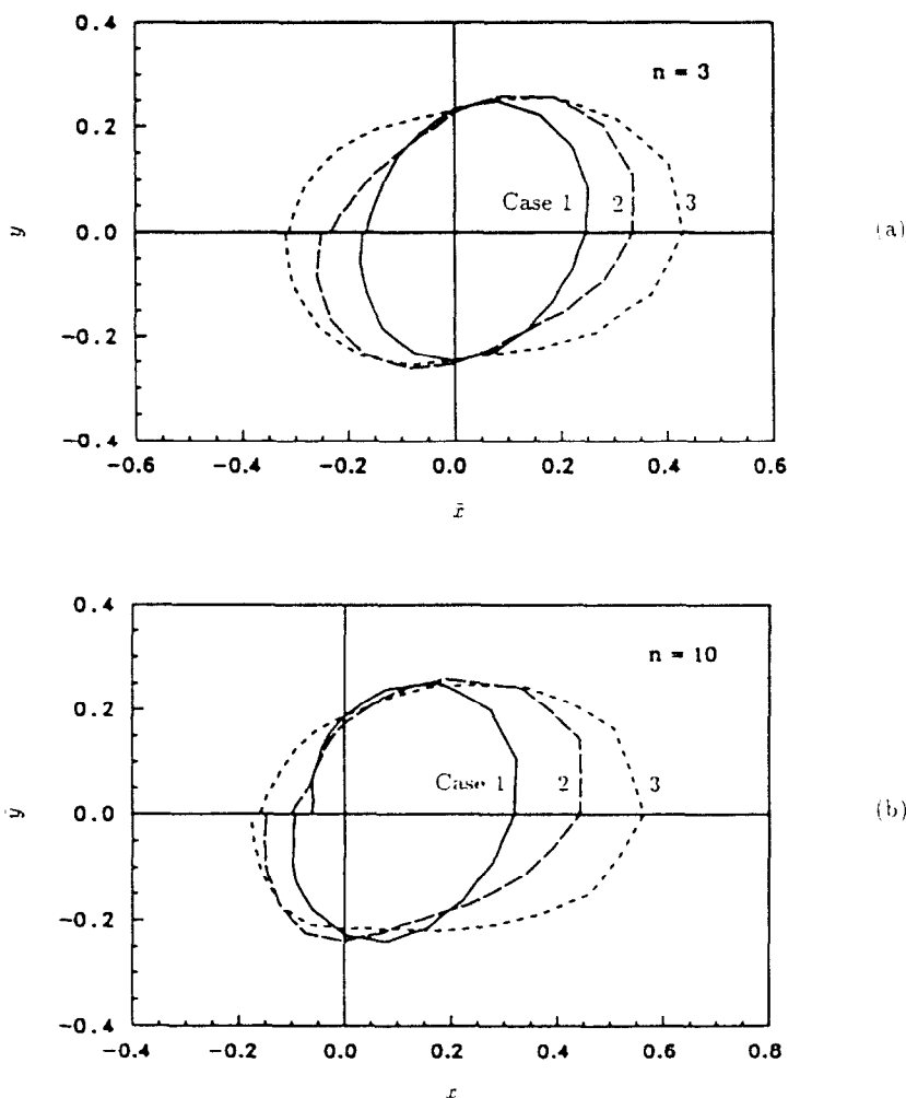
Fig. 9. The plastic zones for Cases 1-3 plotted in the normalized coordinates \bar{x} ( = x\sigma_0^2/JE ) and \bar{y} ( = y\sigma_0^2/JE ) for (a) n = 3 and (b) n = 10 .
