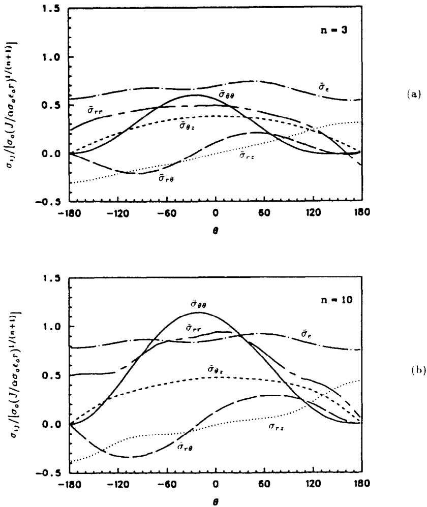
Fig. 6. Case 1 ( M_{12}^e = 0.83 , M_{13}^e = 0.49 and M_{23}^e = 0.16 ): the normalized stresses \bar{\sigma}_{ij} at r/r_p \approx 10^{-3} plotted as functions of \theta for (a) n = 3 and (b) n = 10 .
