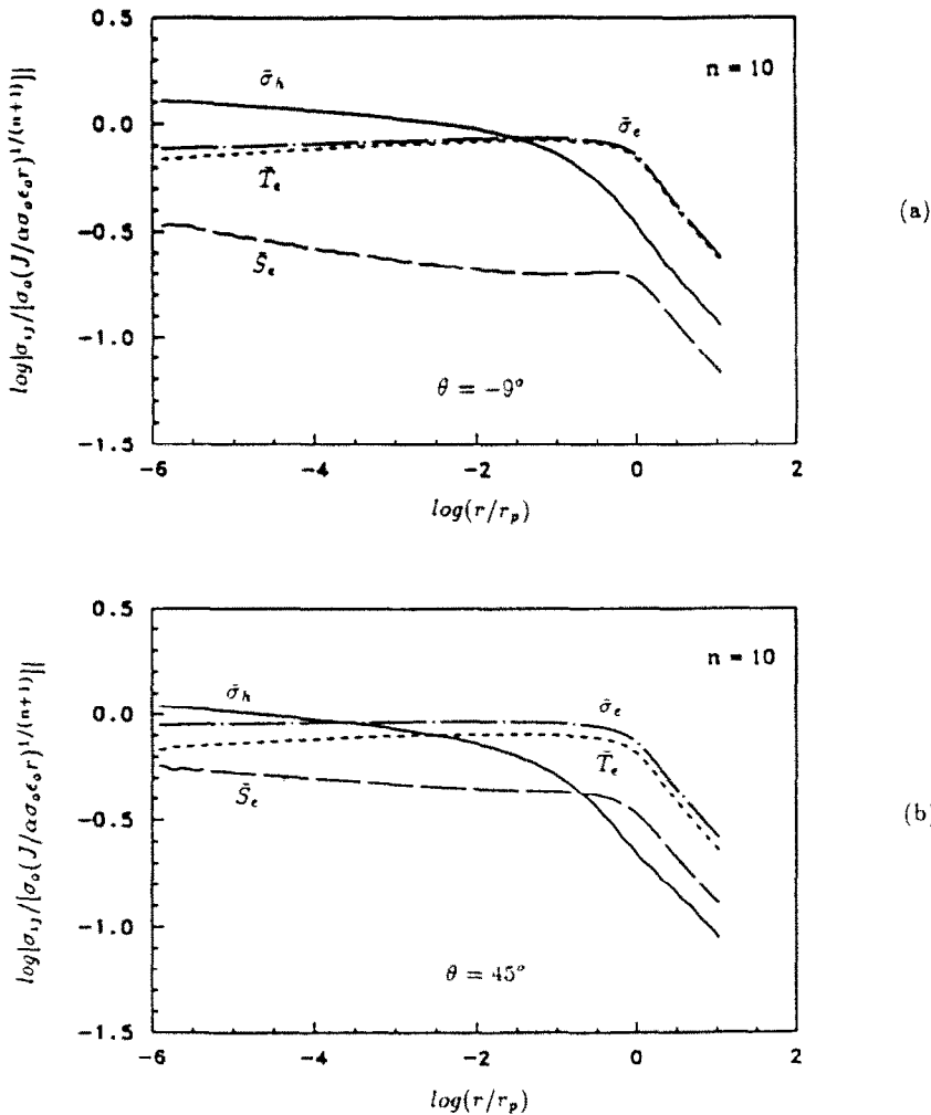
Fig. 10. Case 1 ( M_{12}^s = 0.83 , M_{11}^s = 0.49 and M_{23}^s = 0.16 ): the normalized effective stress \bar{\sigma}_e , the normalized effective in-plane shear stress \bar{S}_e , the normalized effective out-of-plane shear stress \bar{T}_e , and the normalized hydrostatic stress \bar{\sigma}_h for n = 10 as functions of r/r_p plotted in a log-log scale at (a) \theta = -9^\circ , and (b) \theta = 45^\circ .
