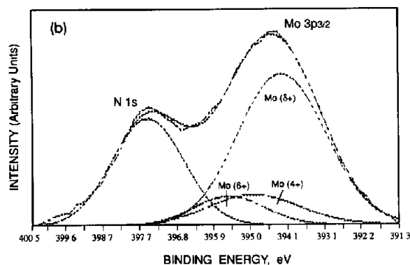
Fig. 3. X-ray photoelectron spectra in the (a) Mo(3d) and (b) Mo(3p) regions.
