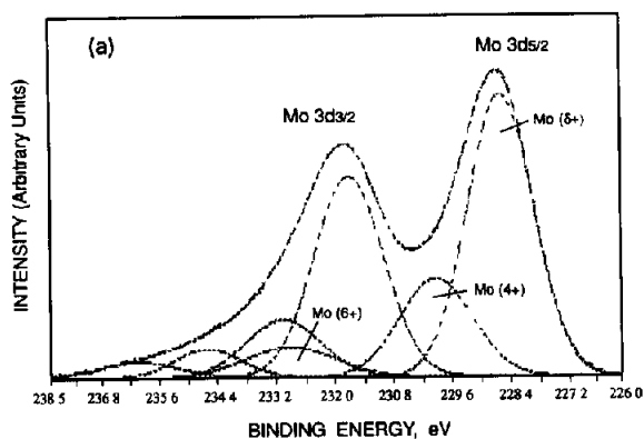
Fig. 3. X-ray photoelectron spectra in the (a) Mo(3d) and (b) Mo(3p) regions.
