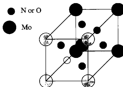
Fig. 4. Hypothetical Mo_2N_{3-x}O_x structure in which all of the octahedral interstices are filled (with nitrogen or oxygen). Note: similar shading indicates atoms lying on the same plane and similar size denotes atoms of the same type
