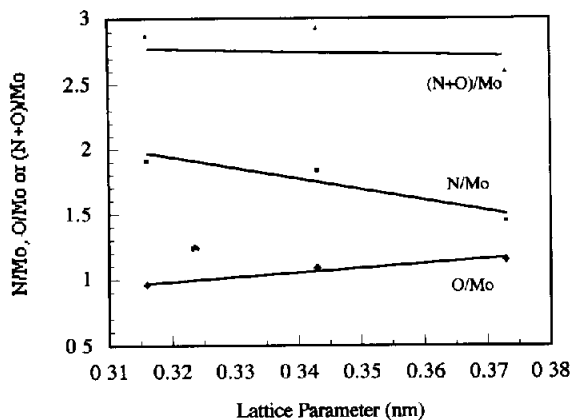
Fig. 2. N/Mo, O/Mo and (N+O)/Mo ratios as a function of the calculated lattice parameter.
