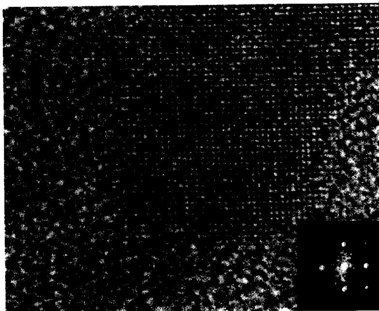
Fig. 1. Atomic-resolution transmission electron micrograph of MoN-2 looking down a \langle 100 \rangle zone axis, showing \{001\} and \{011\} atomic columns. The inset shows the corresponding optical diffraction pattern, containing (001) and (011) type reflections.
