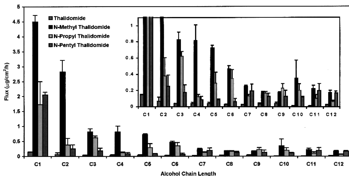
Fig. 3. Steady-state fluxes of thalidomide and its N -alkyl analogs from saturated n -alcohol solutions plotted against the alcohol chain length. These data are the mean \pm standard deviation (SD) of 3 diffusion experiments.
