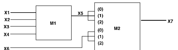
Fig. 2. Modular circuit with virtual fanouts.
