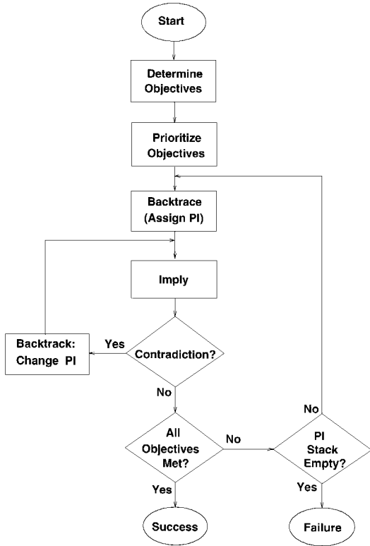
Fig. 8. MODET algorithm.
