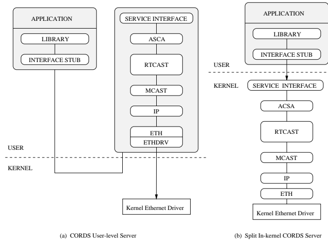
Figure 10. RTCAST protocol stack as implemented
