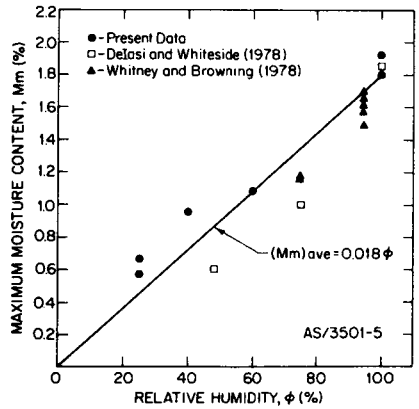
Figure 10. Maximum moisture content as a function of relative humidity for Hercules AS/3501-5 composites. Solid line is fit to data.
