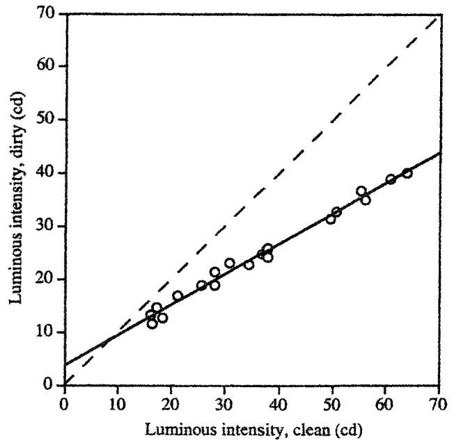
Figure 1 The relationship between the 'clean' and 'dirty' luminous intensities for the left lamp after the snowy/salty drive. The solid line is the best-fitting linear model ( y = 0.57x + 4.0 ). For comparison, the dashed line shows where points would fall if luminous intensities were unaffected by dirt ( y = x ).
