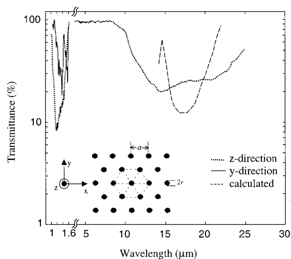
FIG. 3. Transmission spectra show a stop band between 15 and 20 \mu\text{m} along z direction for a PBG material with a=6.3 \mu\text{m} , r=0.15\text{--}1.5 \mu\text{m} , and index contrast of 2.36. Also shown are the stop bands around 1 \mu\text{m} measured along the y and z directions and the calculated stop band.
