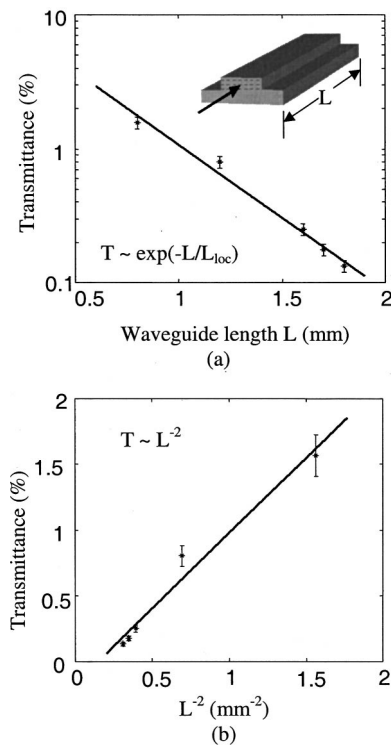
FIG. 4. Measured transmission of end-fired 1.15 \mu\text{m} light through waveguides (y direction) as a function of guide length. The polarization of the incident light is parallel to the heterostructure layers. The measured transmission is fitted to: (a) exponential and (b) quadratic variation with waveguide length. Both fits are good, indicating possibly photon localization.
