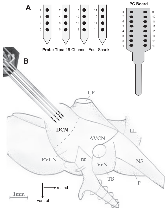
FIG. 2. (A) Geometry of the four-shank 16-channel silicon probe used in this study. The leads from each electrode are connected to the PC board shown at the top. The recording sites are distributed across the array, with four recording sites per shank separated by 100 μm. The four shanks are each separated by 250 μm. (B) The probe tips were placed on the surface of the dorsal cochlear nucleus (DCN) and advanced in a dorsal-to-ventral-to-rostral direction until the tips were located 0.5 mm below the surface of the DCN. The electrode tips were located in the same medial-lateral location (1 mm medial to the parafloccular recess) in all animals. AVCN, anteroventral cochlear nucleus; PVCN, posteroventral cochlear nucleus; nr, VIII nerve root; VeN, vestibular nerve; P, pons; TB, trapezoid body; LL, lateral lemniscus; N5, Vth nerve; CP, cerebellar peduncle.
