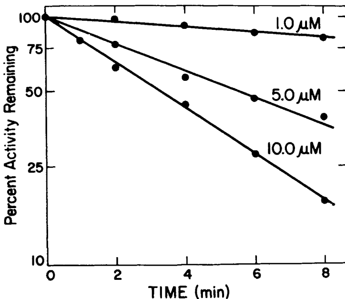
FIGURE 4. The inactivation of urokinase by Phe-Ala-ArgCH 2 Cl. Prior to activity determination by the standard assay, urokinase ( 1.08 \times 10^{-10} M) was incubated with the indicated concentration of the tripeptidyl inhibitor in 80 mM sodium glycinate, pH 8.50 with 1 mg/ml bovine serum albumin, 25^\circ C. At the indicated times, 5 \mu\text{l} of the reaction solution were diluted into 85 \mu\text{l} of the same glycine buffer at 0^\circ . At the completion of the inactivation reaction ( 8 min) all activation reactions were initiated simultaneously by addition of 10 \mu\text{l} of 10 \mu\text{M} plasminogen and removal to a 37^\circ C incubator. 900 \mu\text{l} rather than 950 \mu\text{l} of plasmin reaction solution was used. k_{app}/[I] = 260 \times 10^3 \text{ min}^{-1} \cdot \text{M}^{-1} .
