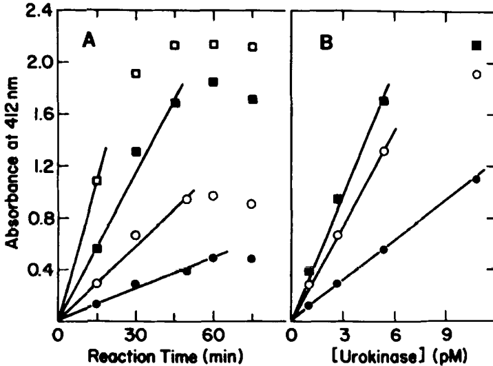
FIGURE 2. The time- and urokinase concentration-dependence of the plasminogen activation reaction coupled to the hydrolysis of Z-Lys-SBzl by plasmin. The conditions for the thiol ester hydrolysis are described in the Experimental section. A. The reaction was terminated at the indicated time by addition of 950 \mu l of the plasmin reaction solution as described in the text. Urokinase concentrations were 1.08 (●), 2.7 (○), 5.4 (■), and 10.8 (□) pM. B. Conditions were as described in FIGURE 2A. The activations were quenched at 15 (●), 30 (○), and 45 (■) min. Data at 60 and 75 min are not presented since the response is not a linear function beyond 45 min (see FIGURE 2A). All times and concentrations relate to the 50 \mu l activation reaction. The lines represent a linear-regression fit of the data and are drawn to encompass only the linear portion of the data. All data points represent the average of duplicates.
