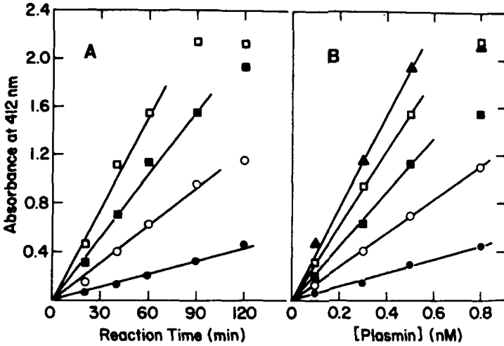
FIGURE 1. The time- and plasmin concentration-dependence of Z-Lys-SBzl hydrolysis. A. Reactions were stopped at the time indicated by addition of soybean trypsin inhibitor. Reaction volume was 1.0 ml. [Z-Lys-SBzl] = 200 \mu M, [DTNB] = 220 \mu M. Plasmin concentrations were 0.1 (●), 0.3 (○), 0.5 (■), and 0.8 (□) nM. B. Conditions were as stated in FIGURE 1A. The reactions were stopped at 20 (●), 40 (○), 60 (■), 90 (□), and 120 (▲) min. The lines were determined by linear-regression fit of the data and are drawn to encompass only the linear portion of the data. All data points represent the average of duplicates.
