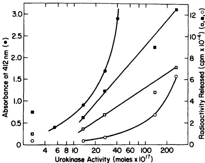
FIGURE 3. A comparison of spectrophotometric and radiometric coupled assays for urokinase. The spectrophotometric assay (●) was performed according to the standard procedures outlined in the text. The volume of continuous radiometric assay is 1.0 ml in 100 mM sodium glycinate, pH 8.50 with 50 nM plasminogen. Total CPM released at 60 (□) and 105 (■) min of incubation are presented. The latter time is the total time required by the discontinuous assays. In the discontinuous radiometric assay (○) plasminogen (1.0 \mu\text{M} ) was activated by urokinase in the glycine buffer for 45 min then a 50 \mu\text{l} aliquot was added to the [ ^{125}\text{I} ]fibrin-coated well containing 950 \mu\text{l} of 200 mM sodium phosphate and 200 mM NaCl. Total CPM released after 60 min in the presence of fibrin are presented. All reactions were performed at 37° C. All radiometric points are averages of triplicates. All spectrophotometric points are averages of duplicates.
