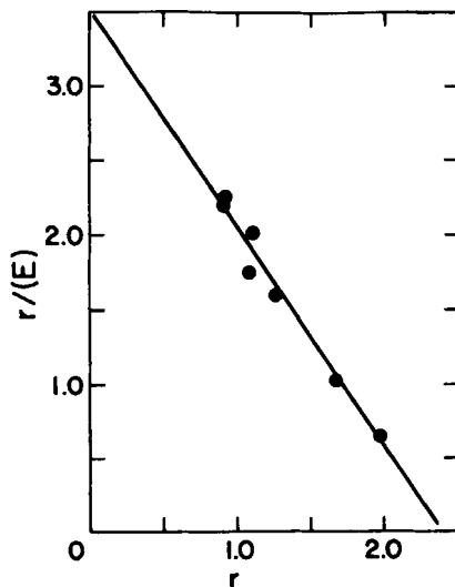
FIGURE 5. Scatchard analysis of the inhibition of urokinase by the plasminogen-activator inhibitor from hepatoma tissue-culture cells. The inhibitor test solution was the serum-free conditioned medium from dexamethasone-induced ( 10^{-7} M, 16 h) cells. 1–5 \mu l of test solution were incubated with urokinase ( 2.7 \times 10^{-10} moles) for 15 min at 25° in 45 \mu l total volume. The activation reaction was started by the addition of 5 \mu l of 10 \mu M plasminogen and shifted to 37° C. E is the concentration of active urokinase; r is the concentration of inactive urokinase.
