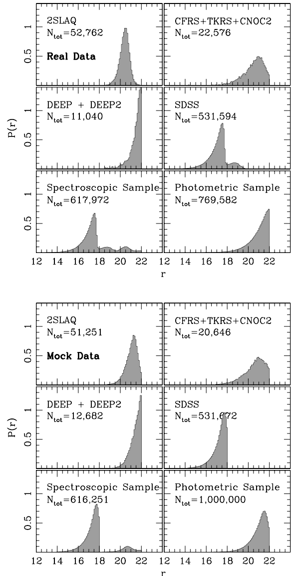
Figure 1. Normalized r magnitude distributions for the catalogues comprising the real SDSS DR6 (top: figure a) and the mock SDSS DR6 (bottom: figure b) catalogues. In each figure, the top four panels indicate the distributions for the different spectroscopic subsamples (see text), bottom left-hand panels indicate flux distributions for the combined spectroscopic samples and bottom right-hand panels indicate distributions for the photometric samples. In each panel, N_{\text{tot}} denotes the total number of galaxy measurements used in each sample.
