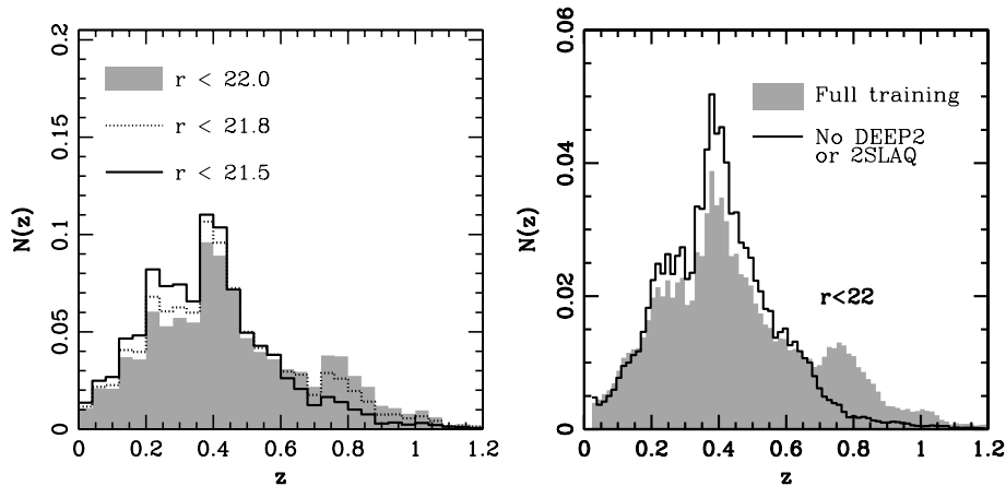
Figure 17. Left: weighted estimates of the redshift distribution for the SDSS DR6 photometric sample, with r < 21.5 , r < 21.8 and r < 22 . Right: p(z) estimates of redshift distribution for SDSS DR7 photometric sample using the full training set as well as a training set without the DEEP2 (the non-EGS part) and without 2SLAQ.
