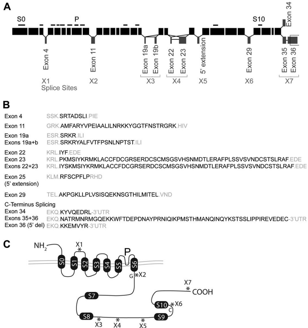
Figure 1. A: A schematic diagram illustrating the exon structure for chick KCNMA1. Constitutive exons in the short isoform (insertless) are shown as black boxes with relative size corresponding to exon length. Alternatively spliced exons and splice-junction modifications are offset. The number and arrangement of facultative and obligatory exons were derived from online databases (Ensembl ENSGALT00000007982) and prior reports of splice variant expression in chick cochlea (Navaratnam et al., 1997; Rosenblatt et al., 1997). Splice sites (X1–X7) are marked and numbered according to the scheme of Fettiplace and Fuchs (1999). Variations at the 5' end of the gene (X0, not shown) have been reported elsewhere (Rosenblatt et al., 1997) but appear to be artifacts (Beisel et al., 2007). Alternative inserts occur at sites X1, X2, X3, X4, X6, and X7. A 3' deletion can truncate the alternative exon at X3, giving rise to two possible inserts (exon 19a or exon 19a+b). Two separate alternative inserts at X4 may occur alone or in combination. At X5 a 5' extension of exon 25 can occur in some species. At X7, mutually exclusive exon use generates several unique C-termini, one consisting of exon 34 ending in the coding sequence QEDRL, one containing exons 35 and 36 and ending in VEDEC, and one incorporating exon 36 with a 5' deletion resulting in a frameshift ending in EMVYR. The subunit contains 12 hydrophobic domains (horizontal black bars), including seven membrane-spanning regions (S0–S6), four additional soluble hydrophobic domains (S7–S10), and a pore loop (P). B: Coding changes are shown for the alternative splicing events illustrated in (A). Gray amino acid residues correspond to flanking obligatory exons and black residues result from splice variation. C: The structure of the BK \alpha subunit is shown, relating splice sites to protein topology. The arrangement of transmembrane domains S0–S6 results in an extracellular amino terminus (NH 2 ) and intracellular carboxy terminus (COOH). Two RCK domains (i.e., regulators of the conductance for potassium) are present, spanning S7 to S8 (RCK1) and S9 to S10 (RCK2). G, glutamate ring essential for the large conductance in BK channels; C, calcium bowl, a high-affinity calcium binding site.
