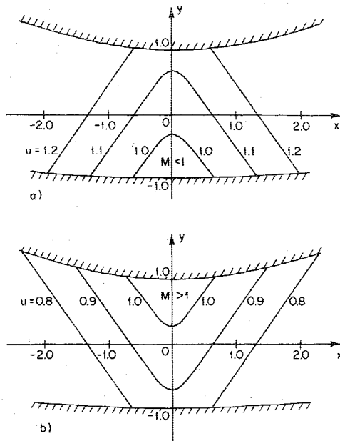
Fig. 2 Isotachs corresponding to Eq. (15a) when \beta_1 > (f''_1)^2/3 ; y_w = \pm 1 + \epsilon x^2/2 \pm \epsilon^2 [1 + 20(\gamma + 1)/9]x^2/2 , \beta_1 = 5/12 , \epsilon = 0.1 . a) + sign taken for all x in Eq. (13b), b) - sign taken for all x in Eq. (13b).
