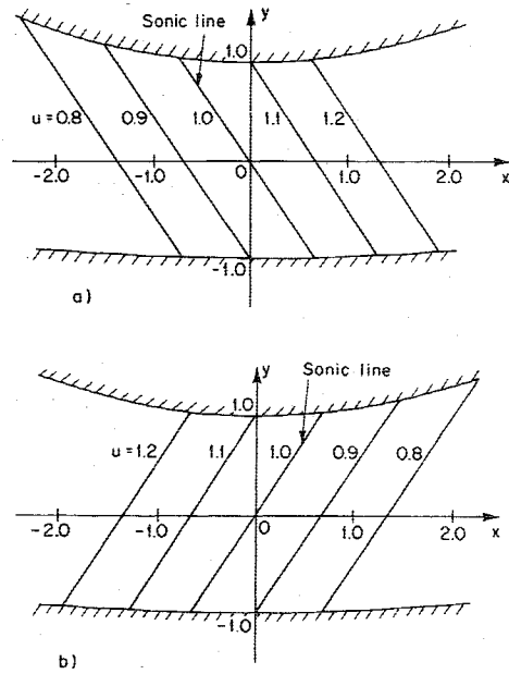
Fig. 4 Isotachs corresponding to Eq. (15a) when \beta_1 = (f''_1)^2/3 = 1/3 , for same wall shapes and \epsilon as in Fig. 2. a) + sign taken for all x in Eq. (13b), b) - sign taken for all x in Eq. (13b).
