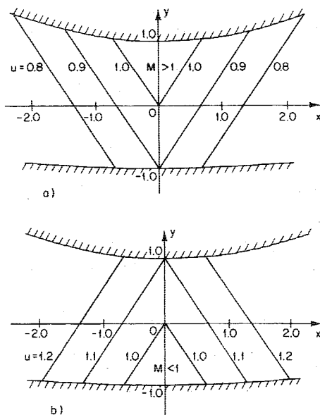
Fig. 3 Isotachs corresponding to Eq. (15a) when \beta_1 = (f''_1)^2/3 = 1/3 , for some wall shapes and \epsilon as in Fig. 2. a) + sign for x < 0 and - sign for x > 0 in Eq. (13b), b) - sign for x < 0 and + sign for x > 0 in Eq. (13b).
