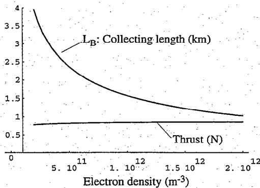
Figure 2 – Variation in thrust with electron density for a 10-km tether with a 5-km-long bare segment. Thrust drops only 10% as density drops by a factor of 10. The reason is clear: the collecting length has increased from 1 to 4 km. The EMF is 1200 V; input power 10 kW.
