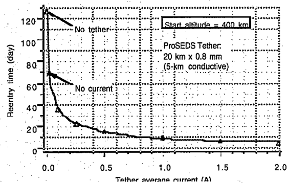
Figure 4 – Predicted ProSEDS performance as a function of average tether current (Courtesy E. Lorenzini, SAO).
