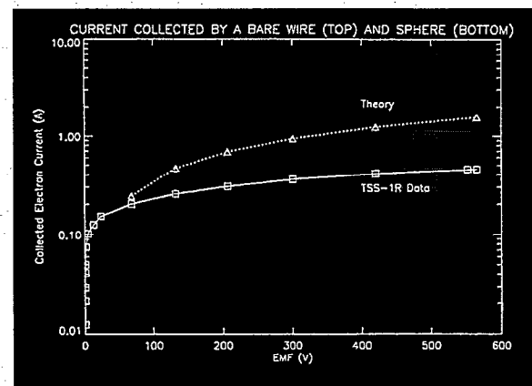
Figure 1 – Current collection efficiency of the bare tether compared to a sphere of equal area.
