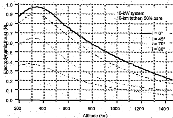
Figure 6 – The performance of an electrodynamic tether thruster varies with altitude in the magnetosphere (where i is the orbital inclination).
