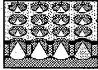
Figure 8 – Sketch of a Field Emitter Array Cathode. Typical tip-to-tip separation is on the order of 2–5 \mu\text{m} .
