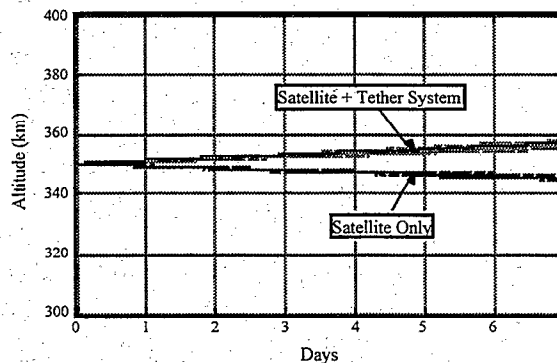
Figure 5— 150-W, 2-km ED-tether orbit maintenance of a 1000 kg, 35° inclination orbit spacecraft system.
