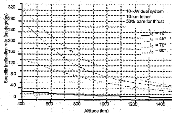
Figure 7 – Electrodynamic tethers can be used to change orbital inclination without propellant consumption. To determine the available inclination change for a spacecraft/payload mass, divide the 'specific inclination rate' indicated by the total system mass at a given altitude.
