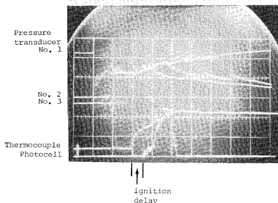
Fig. 4c RDX ( 2 \mu\text{m} ) + air/ \text{O}_2 (88/12), 1300 \text{ g/m}^3 , 1.0 \text{ ms/div} .
