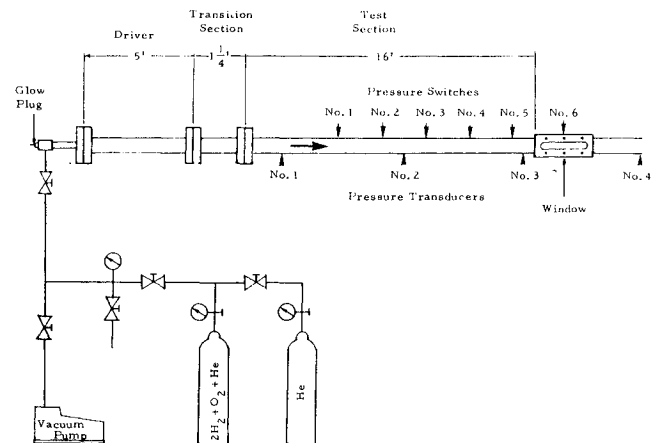
Fig. 1a Schematic of experimental setup.
