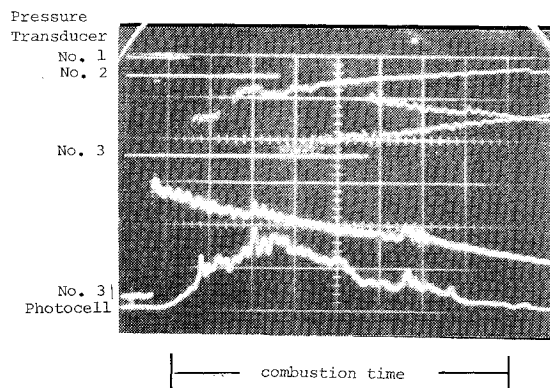
Fig. 4a RDX ( 37 \mu\text{m} ) + air/ \text{O}_2 (88/12), 1300 \text{ g/m}^3 , 0.5 \text{ ms/div} for top three traces, 0.2 \text{ ms/div} for bottom two traces.
