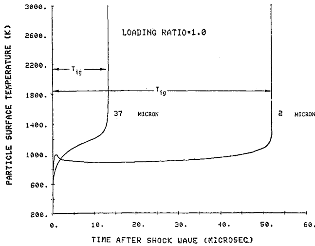
Fig. 6a Surface temperature histories of 2 and 37 \mu\text{m} RDX particles in air/O 2 (88/12) subject to shock wave of M=5.1 .
