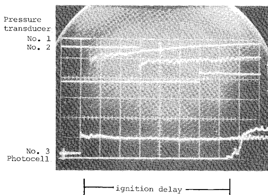
Fig. 4b RDX ( 37 \mu\text{m} ) + \text{N}_2 , 1300 \text{ g/m}^3 , 0.5 \text{ ms/div} .
