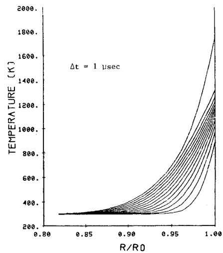
Fig. 7b Time histories of temperature distribution inside a 37 \mu\text{m} RDX particle.
