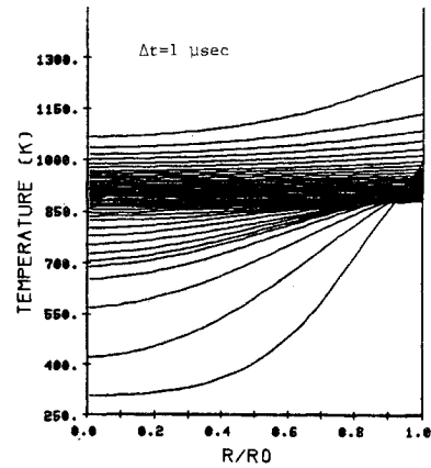
Fig. 7a Time histories of temperature distribution inside a 2 \mu\text{m} RDX particle.
