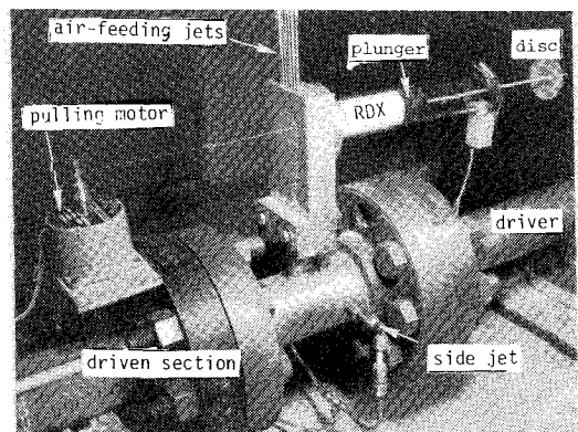
Fig. 1c Transition section and dust feeder.
