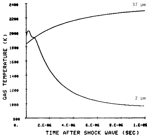
Fig. 6b Gas temperature histories, same flow conditions as in Fig. 6a.
