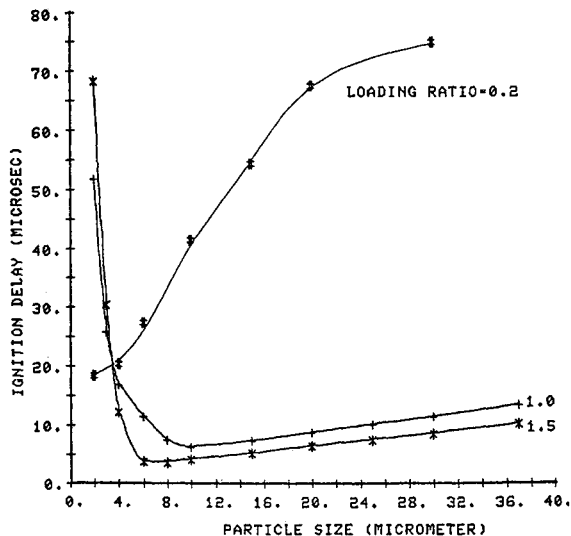
Fig. 8 Ignition delay vs particle size of RDX in air/O 2 (88/12) subject to shock wave of M=5.1 .
