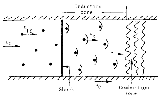
Fig. 5 Schematic of gas/particle flow.
