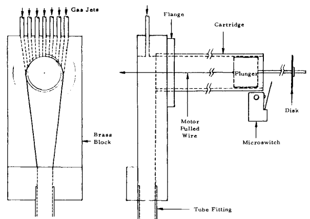
Fig. 1b Schematics of dust feeder.
