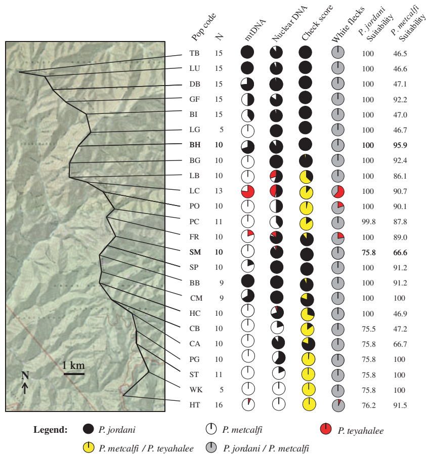
Fig. 3 Map of Balsam Mountain showing transect (bold line), collection localities, sample sizes, marker scores and habitat-suitability values. Pie charts are interpreted as follows: mtDNA = proportion of samples at a given locality that are diagnostic for each parental species, nuclear DNA = proportion of alleles at a given locality that are diagnostic for each parental species, cheek score = the average scaled cheek pigmentation score (i.e. average score divided by the average for pure parental Plethodon jordani ), and white flecks = the proportion of animals that have at least some white flecks. Habitat-suitability values are extracted from the ecological niche models presented in Fig. 7 and are given as a percentage from 0 to 100. Note that more than one collection locality may lie within a single grid cell; therefore, identical values may not be independent from one another.
