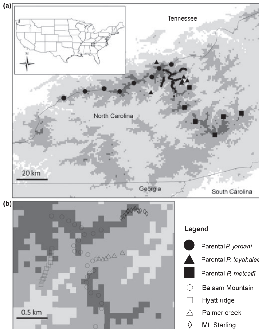
Fig. 1 (a) Map of study area showing collection localities of parental ( Plethodon jordani , Plethodon metcalfi , and Plethodon teyahalee ) and hybrid samples. Inset depicts location of study within the continental United States. (b) Expanded map of hybrid zones from A showing collection localities of hybrid samples. In both a and b, darkened areas = high elevation and light areas = low elevation.
