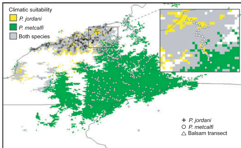
Fig. 7 Ecological niche modelling results showing present-day predicted geographic distributions for Plethodon jordani and Plethodon metcalfi . For comparison, collection localities are shown for both Plethodon jordani (+) and Plethodon metcalfi (O). The inner box encompasses the hybrid zone and is expanded to show sampling localities (Δ) along the Balsam Mountain transect. Colours indicate habitat-suitability values as assigned by Maxent and are given as percentages (cumulative probability × 100; see text for more detail).
