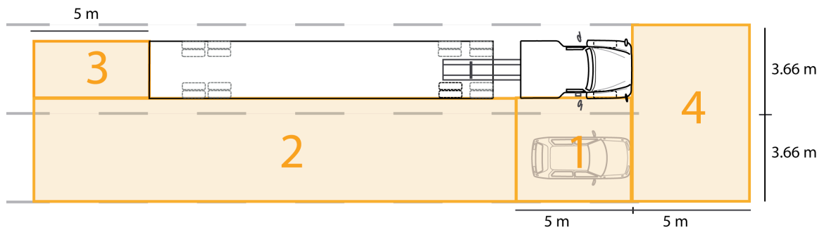
Figure 28. Prioritized zones for driver vision improvement. The highest priority zone is indicated with numeral 1.
