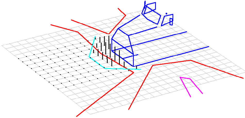
Figure 36. Fraction of the pedestrian population obscured by the hood. A vertical black line indicates fractional obscuration (height is fractional obscuration times one meter). The obscuration boundaries at the 1.2 m plane for the hood (cyan) and greenhouse (red) are shown.
