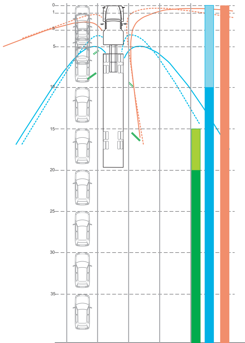
Figure 14. The field setup, showing the position of the tractor-trailer and the potential positions of the passenger car one lane to the left (similar positions could be occupied in the first or second lane to the right of the tractor-trailer). Approximate mirror fields of view are shown for the planar mirrors (green), door-mounted convex (blue) and fender-mounted convex (orange) on the ground plane (solid lines) and 1.2-m plane (dotted lines). The colored bars to the right show the approximate visibility of the target vehicle in each of the right-side mirrors as a function of distance aft of the front bumper. For example, the vehicle was partially visible in the planar mirror at the 10-m mark and fully visible at the 20-m mark.
