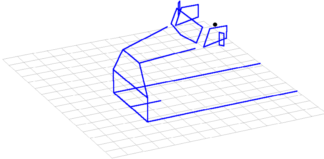
Figure 30. Computer model of vision obstructions for the example vehicle, including window perimeters and the hood. The viewing point (representative driver eye point) is shown with a black dot.
