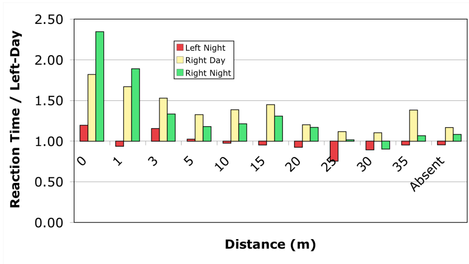
Figure 24. Reaction times referenced to the left-day condition.
