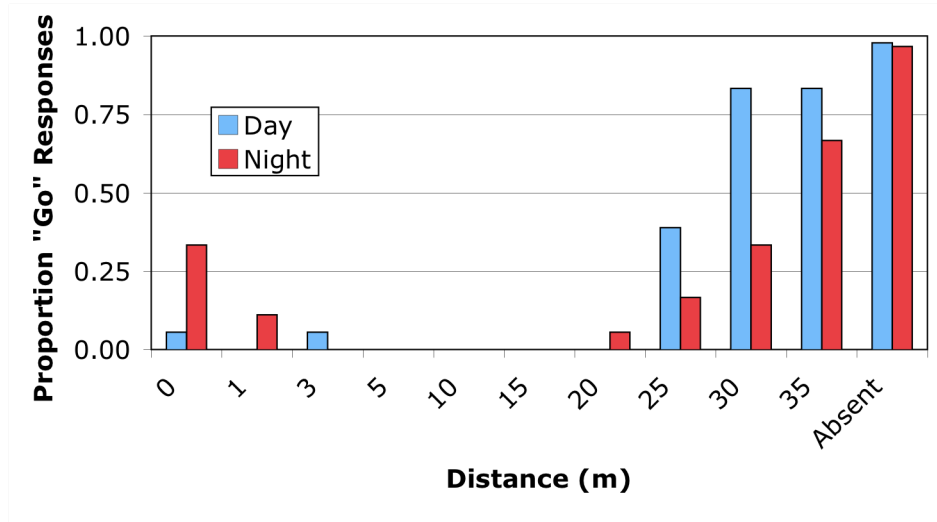
Figure 17. Proportion “go” responses by light condition and distance of the target passenger car. Right-side data only.
