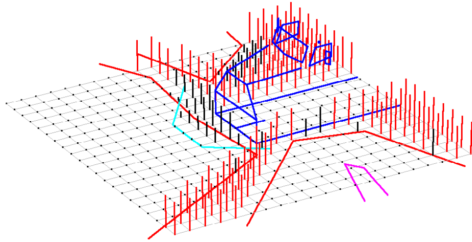
Figure 35. Depiction of the fraction of the population that is obscured for direct vision for the example vehicle geometry. A vertical red line (all are 1-m tall) indicates that the population is completely obscured and a vertical black line indicates fractional obscuration (height is fractional obscuration times one meter). The obscuration boundaries at the 1.2 m plane are shown. Pedestrian obscuration calculations were not performed for mirrors.
