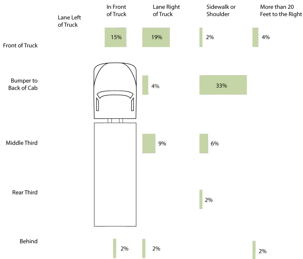
Figure 13. Position of nonmotorist at truck driver's decision point, Turn Right/Nonmotorist Crashes, TIFA 1999-2000, N=70. One case was not applicable (driver lost control due to a medical emergency). Sixteen of 70 cases were excluded from the calculation of percentages because the position could not be coded.
