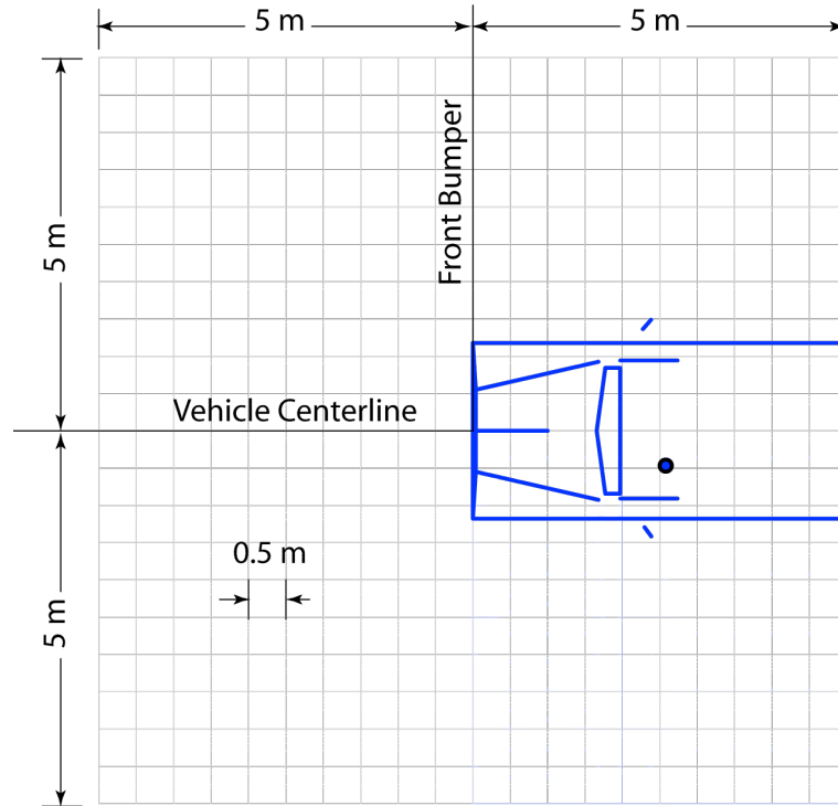
Figure 31. Laying out sample points (plan view). Each intersection point on the grid is a sample point.
