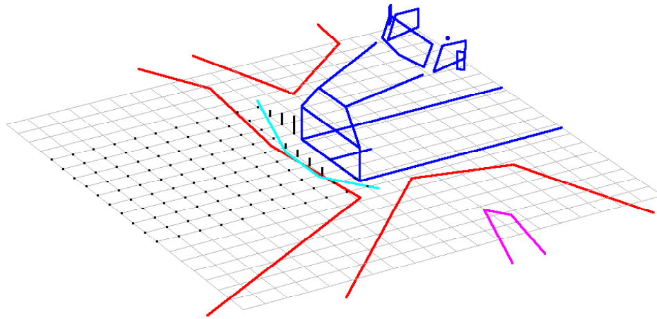
Figure 37. Fraction of the pedestrian population obscured by the hood, using the example cab geometry with front hood points lowered by 0.2 m. A vertical black line indicates fractional obscuration (height is fractional obscuration times one meter). The obscuration boundaries at the 1.2 m plane for the hood (cyan) and greenhouse (red) are shown.
