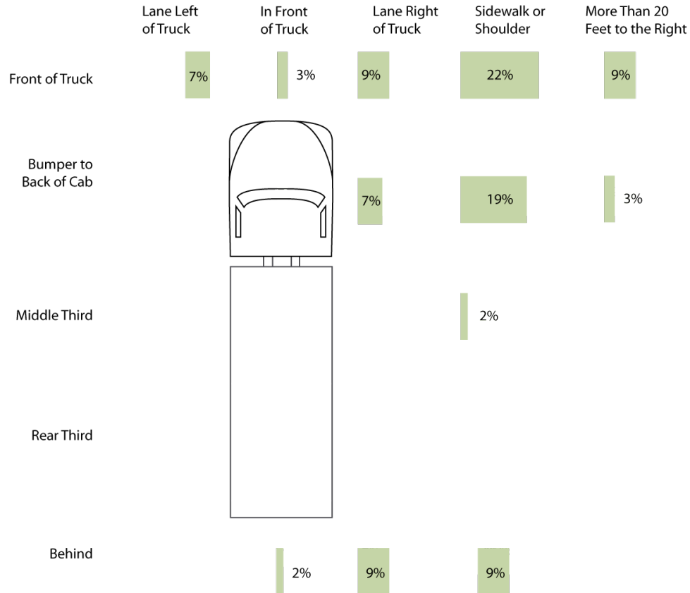
Figure 12. Position of nonmotorist 3-5 seconds prior to decision point, Turn Right/Nonmotorist Crashes, TIFA 1999-2000, N=70. Twelve of 70 cases are excluded from calculation of percentages because the position could not be coded.
