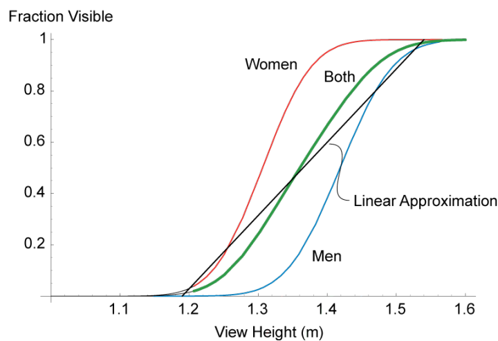
Figure 34. Fraction of adult pedestrian population that is visible as a function of view height from the ground.
