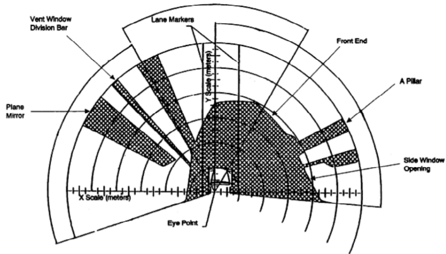
Figure 29. Sample horizontal projection plot from SAE J1750.
