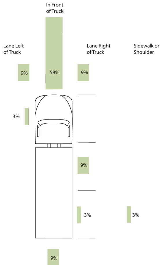
Figure 9. Position of nonmotorist at truck decision point, Start Up Crashes, TIFA 1999-2000, N=38. Other (underneath truck): 3.0%. Position could not be coded for 13.2% of the 38 cases, and are excluded from the percentage calculations.
