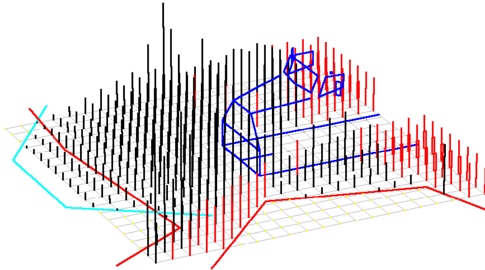
Figure 33. Illustration of direct view heights on sampling points. A vertical red line indicates that a vertical line through the sampling point is completely obscured. A black line indicates that the view is partially obscured and shows the minimum height that is visible. The obstruction perimeters on the ground plane are shown for the windows and windshield (red lines) and hood (cyan line).
