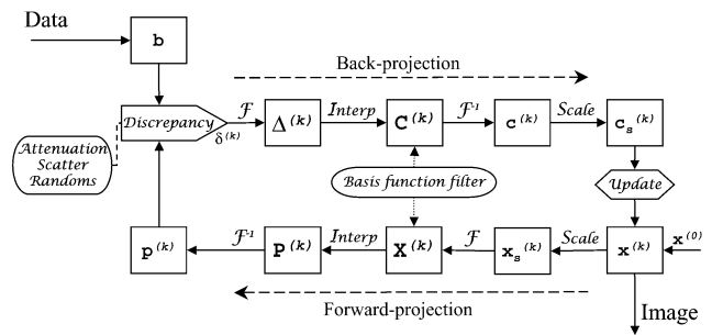
Fig. 2. Flowchart of iterative reconstruction using Fourier-based forward and back-projection. Discrepancy and Update operators are defined by a particular iterative technique. For the 2-D case, the Fourier transformations are 1-D (I)FT of projections on the data side and 2-D (I)FT on the image side. Interpolation operations are performed between data (polar) and image (rectangular) spectrum grids. For Scale and Basis function filter , see caption of Fig. 1.
