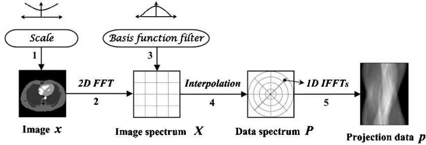
Fig. 1. Basic steps of the NUFFT forward-projection illustrated on the 2-D case: 1) point-wise multiplication of the image with the Scale function—pre-compensation for interpolation imperfections; 2) Fast Fourier Transform on uniform (rectangular) rasters from image into spectrum domain; 3) point-wise spectrum multiplication by Basis function filter —modeling effects of the image representation using basis functions (Section II-D) and of the shift-invariant detector resolution kernels (Section II-E1, for other possibilities of resolution modeling see text); 4) Interpolation into nonuniform (polar) data spectrum raster locations—using the fixed size interpolation kernel; 5) Inverse Fast Fourier Transforms on set of polar lines to obtain a set of projections (sinogram).
