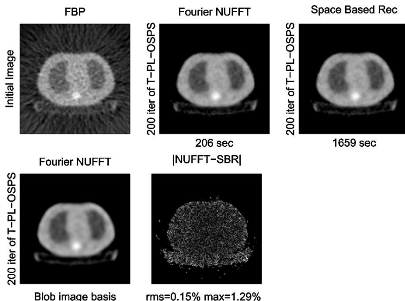
Fig. 17. FBP (serving as initial image) (top left) and T-PL-OSPS reconstructions (200 iterations) from transmission data (from ECAT-921 scanner) of physical thorax phantom using Fourier-based NUFFT with (theoretically) optimized KB kernel ( K/N = 2 , m = 0 , J = 4 , and \alpha/J = 2.34 ) (top middle) and space-based (SBR) (top right) forward and back-projectors. Illustrative times are for Matlab implementations. Bottom left is illustration of NUFFT iterative reconstruction including modeling of a blob basis function and bell-shaped detector resolution kernel. Bottom right is absolute difference image (including measures of root-mean-square difference and maximum absolute difference) between reconstructions using Fourier-based NUFFT and space-based projectors.
