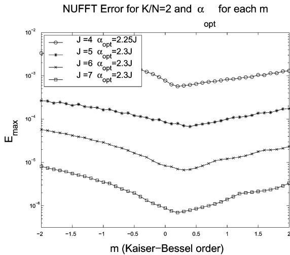
Fig. 6. Maximum error E_{\max} of KB interpolator as a function of the order m , for several sizes J , 100% zero-padding ( K/N = 2 ) and using optimum ratio \alpha/J for each particular value of m . The optimum order parameter m is slightly above 0 for all kernel sizes; \alpha_{\text{opt}} in the legend represent global optimum of the \alpha parameter for the given kernel size.
