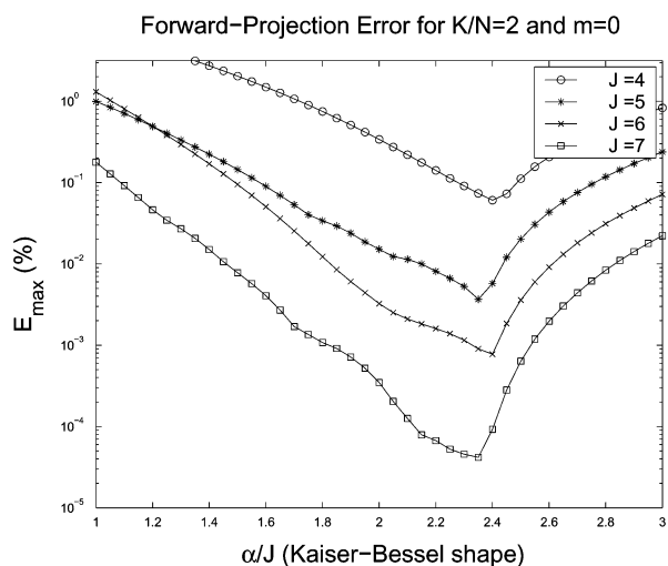
Fig. 9. Maximum interpolation error (% of projection maximum) of forward-projection of modified Zubal phantom using NUFFT with KB interpolator of several sizes J as a function of the parameter \alpha . Same set of parameters used as for the Fig. 5.
