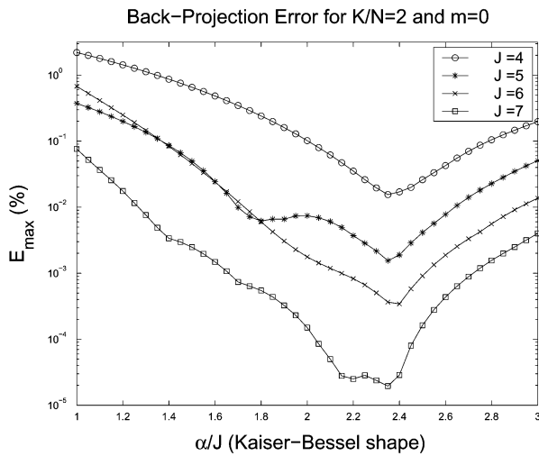
Fig. 12. Maximum interpolation error (% of phantom maximum) of discrete back-projection using NUFFT with KB interpolator of several sizes J as a function of the parameter \alpha . Same set of parameters used as for the Figs. 5 and 9.
