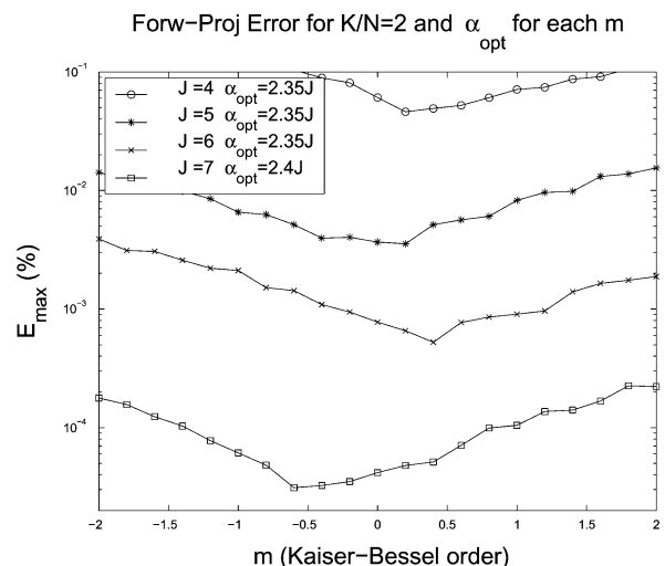
Fig. 10. Maximum interpolation error (% of projection maximum) of forward-projection of modified Zubal phantom using NUFFT with KB interpolator of several sizes J as a function of the KB order m . For each individual m an optimum \alpha was used. \alpha_{\text{opt}} in the legend represent global optimum of the \alpha parameter for the given kernel size.
