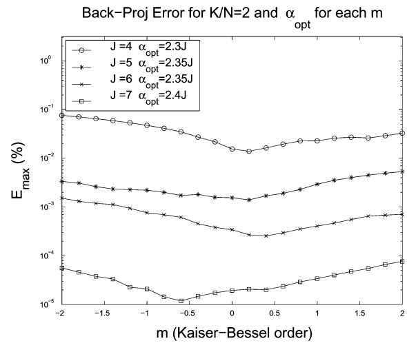
Fig. 13. Maximum interpolation error (% of phantom maximum) of discrete back-projection using NUFFT with KB interpolator of several sizes J as a function of the KB order m . For each individual m an optimum \alpha was used. \alpha_{opt} in the legend represent global optimum of the \alpha parameter for the given kernel size.
