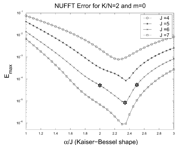
Fig. 5. Maximum error E_{\max} of KB interpolator as a function of the shape parameter \alpha , for several interpolation kernel sizes J , Bessel order m = 0 and using 100% zero-padding of the spatial domain ( K/N = 2 ) (NUFFT interpolator has been found to perform best for the KB orders close to m = 0 —see Fig. 6). Note that the optimum ratio \alpha/J is about 2.34 for various kernel sizes.
