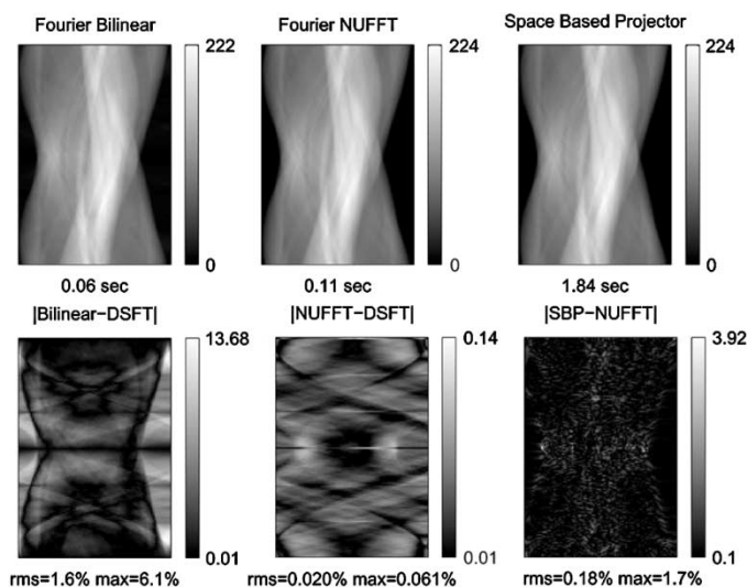
Fig. 8. Example of sinograms (illustrated using 144 angular samples) of Zubal phantom obtained by Fourier-based forward-projector using bilinear interpolation ( K/N = 2 ) (top left), Fourier-based forward-projector using NUFFT with optimized KB kernel ( K/N = 2, m = 0, J = 4 , and \alpha/J = 2.4 ) (top middle) and a space-based forward-projector (SBP) (top right). Illustrative times are for Matlab implementations. Bottom row shows corresponding absolute difference sinograms (including measures of root-mean-square difference and maximum absolute difference) with respect to the exact Fourier projector (DSFT) (bottom left and middle), and Fourier NUFFT projector (bottom right).
