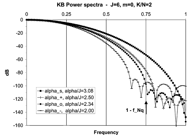
Fig. 4. Power spectra of KB interpolation kernels using optimum ( \alpha_{o} ) and suboptimum parameters for J = 6 , m = 0 and K/N = 2 , whose profiles are shown in Fig. 3.
