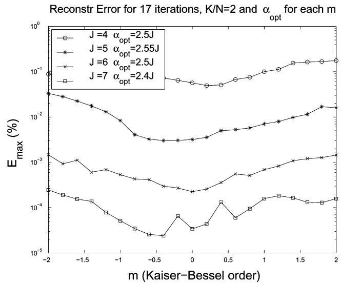
Fig. 16. Maximum interpolation error (% of phantom maximum) of 17 iterations of QPWSL reconstruction using NUFFT forward and back-projectors with KB interpolator of several sizes J as a function of the KB order m . For each individual m an optimum \alpha was used. \alpha_{opt} in the legend represent global optimum of the \alpha parameter for the given kernel size.
