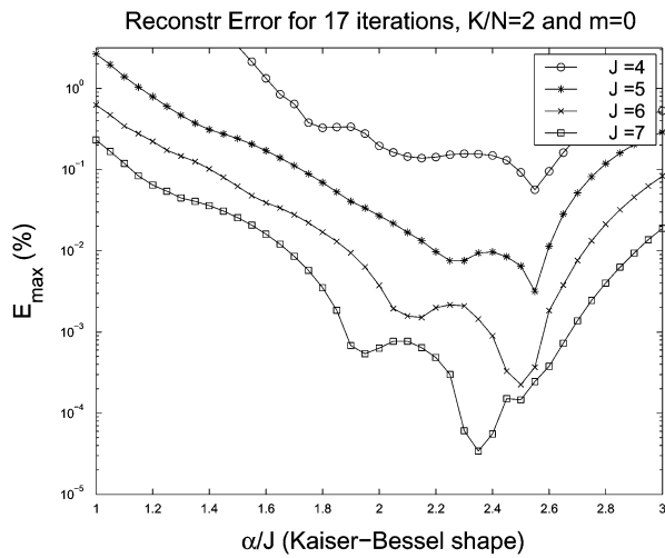
Fig. 15. Maximum interpolation error (% of phantom maximum) of 17 iterations of QPWSL reconstruction using NUFFT forward and back-projectors with KB interpolator of several sizes J as a function of the parameter \alpha . Same set of interpolation parameters used as for the Figs. 5, 9, and 12.
