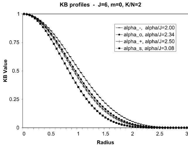
Fig. 3. Profiles of four KB interpolation kernels of size J = 6 using optimum ( \alpha_{o} ) and suboptimum parameters for m = 0 and K/N = 2 . \alpha_{-} and \alpha_{+} represent two suboptimum KB kernels ( \alpha parameter located on both sides from the optimum—star symbols in Fig. 5) providing comparable maximum errors, which are about 6.5 times higher than in the optimum case. For comparison, we show also \alpha_{s} representing typical KB window having desirable properties for the spatial image representation [35], but poor performance as the interpolation kernel. It is interesting that although all of them have similar shape, they provide quite dramatic difference in the NUFFT performance.
